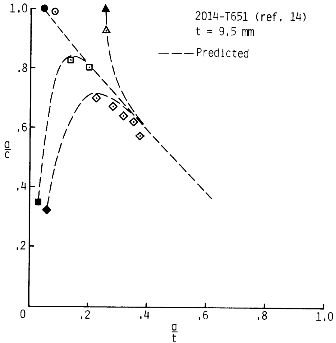
Figure 13.- Experimental and predicted fatigue-crack growth patterns for a surface crack in an aluminum alloy cantilever plate under bending. (Solid symbols denote initial conditions.)
