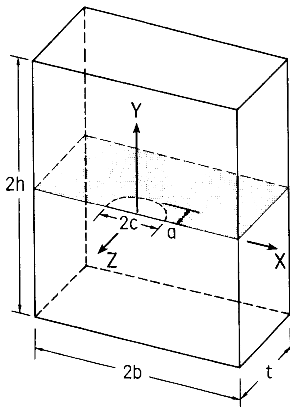
Figure 1.- Surface crack in a finite plate.
