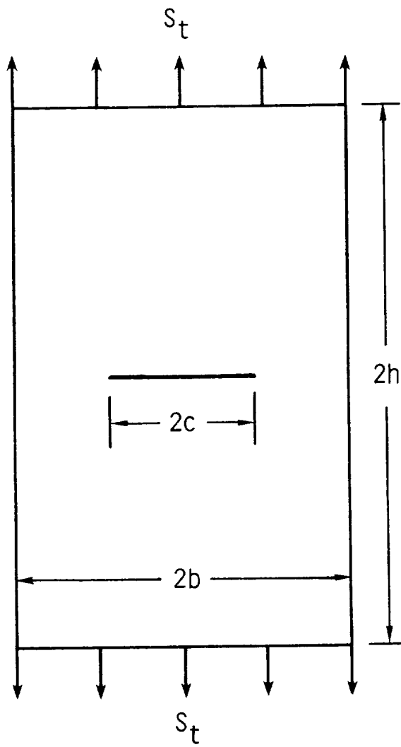
(a) Tension.
