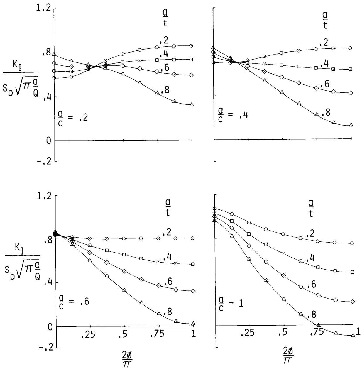
Figure 7.- Normalized stress-intensity factors along the front of a semielliptical surface crack in a plate under bending. ( c/b \leq 0.2 .)
