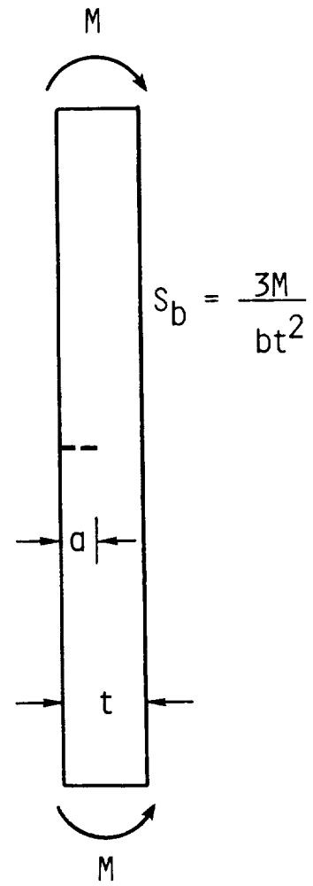
(b) Bending.
