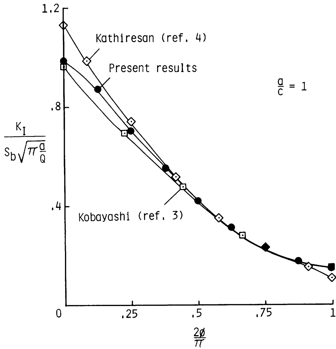
(a) a/t = 0.6 .
