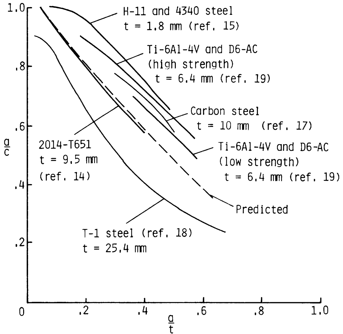
Figure 15.- Experimental and predicted fatigue-crack-growth patterns of surface cracks in plates of various materials under bending.
