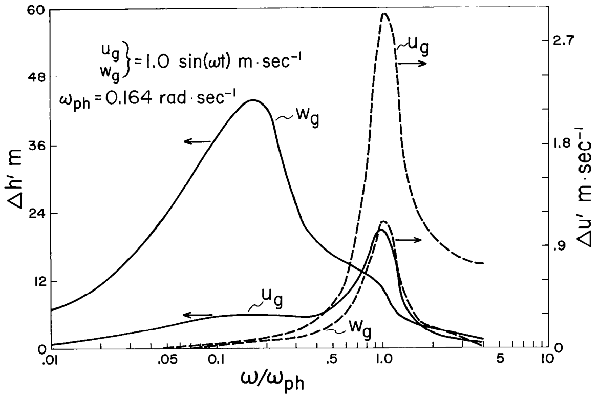
Fig. 4. RMS altitude and velocity deviations of a Boeing 727 class airplane to continuous one \text{m} \cdot \text{sec}^{-1} horizontal or vertical sine wave winds during a landing from 500 m altitude to the ground.
