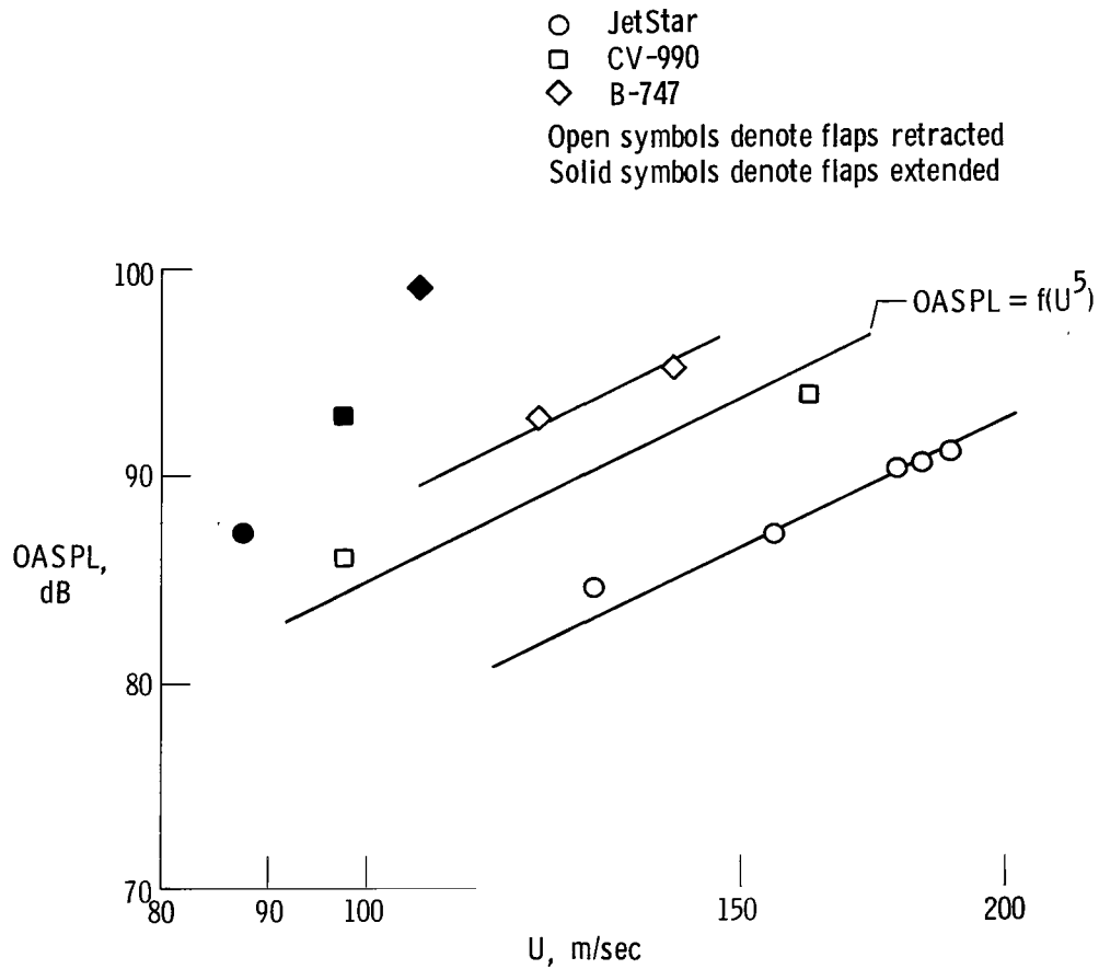
Figure 5. Variation of airframe noise with airspeed for the jet aircraft in landing-gear-up configuration. Data are normalized to an altitude of 152 meters.
