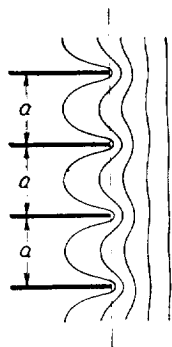
FIG. 60.—Conformal transformation
