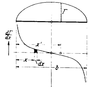
FIG. 44.—Velocity at a point x' due to vortex leaving wing at point x .
