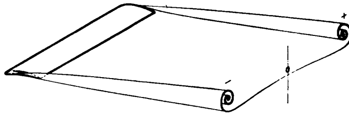
FIG. 42.—Change in shape of vortex ribbons at great distances behind the wing.
