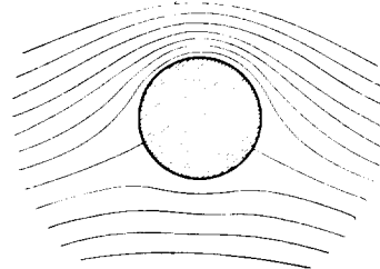
FIG. 21.—Superposition of two preceding flows.
