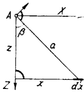
FIG. 52.—Velocity at a point A off the lifting line, but in the transverse plane, due to the vortex system.
