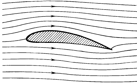
FIG. 25.—Transformation of simple potential flow, figure 19.
