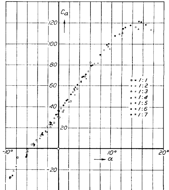
FIG. 49.—Lift coefficients as function of angle of attack, reduced for aspect ratio 1.5.
