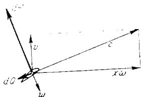
FIG. 58.—Velocity field near a blade of a screw-propeller.
