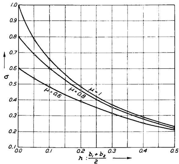
Fig. 51.—Curve of the function \sigma for biplanes whose span ratio, \mu = \frac{b_2}{b_1} , is varied.
