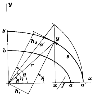
FIGURE 2.—Geometric data for confocal ellipses. x = a' \cos \eta = r \cos \beta ; y = b' \sin \eta = r \sin \beta ; b'/a' \tan \theta = \tan \eta = b'/r \tan \beta = a'/r \tan \theta ; h_1 = r \sin(\theta - \beta) ; h_2 = r \cos(\theta - \beta) . f = ae = a' e' , e = \sqrt{1 - b^2/a^2} being eccentricity of ab
