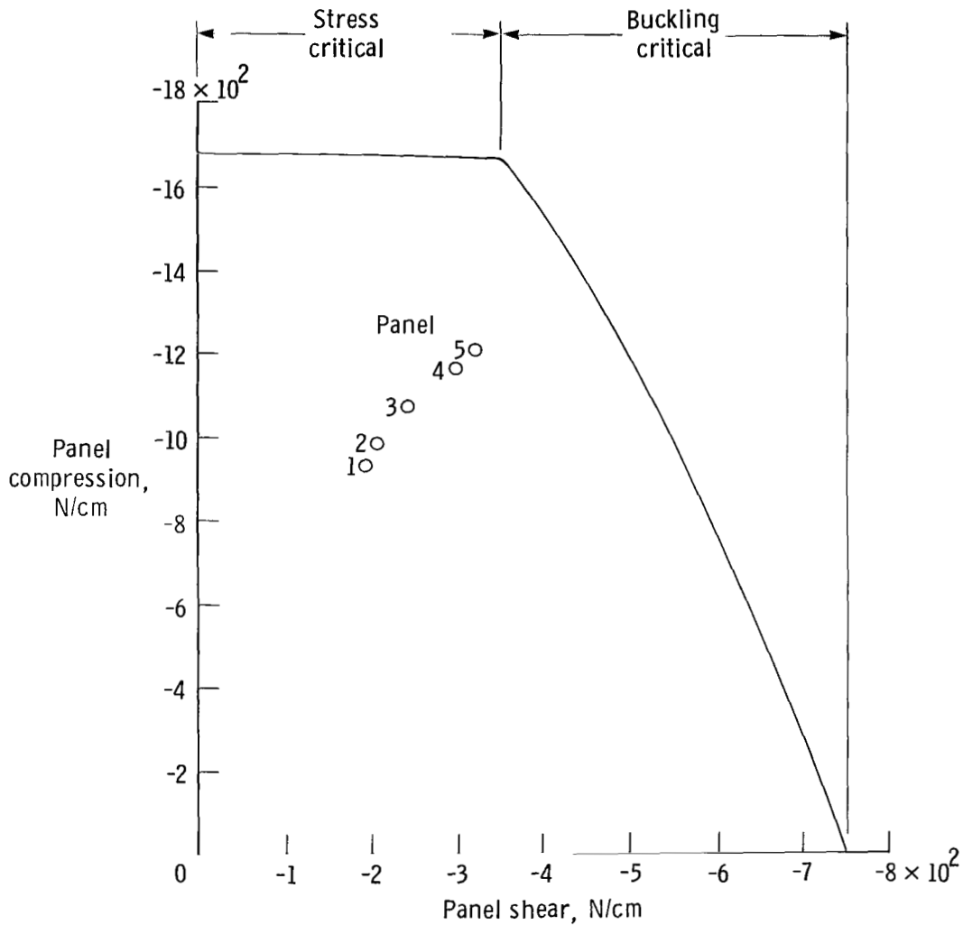
Figure 18. Beaded panel strength interaction curve at 1005 K and 5.2 \text{ kN/m}^2 from OPTBEAD program (ref. 5).
