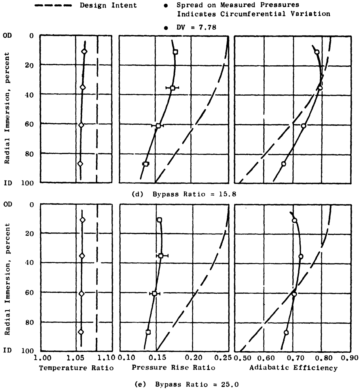
Figure 30. Comparison of Radial Profiles of Temperature Ratio, Pressure Rise Ratio, and adiabatic Efficiency at Transition Duct Discharge for Various Bypass Ratios at 90% Speed with Nominal Rotor Pitch ( \beta_F = 0^\circ ) (Concluded).
