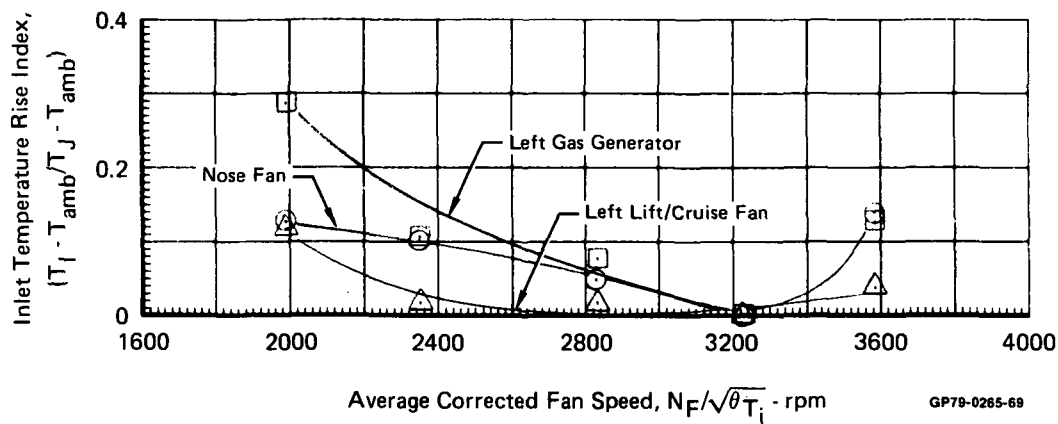
FIGURE 4-55 EFFECT OF FAN SPEED ON INLET REINGESTION Baseline Configuration 3-Unit Configuration H/D = 6.45
