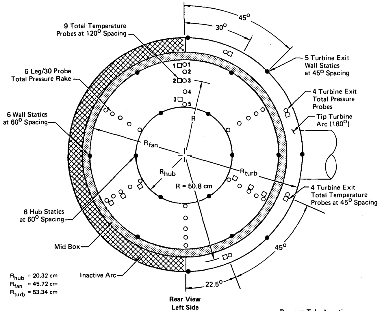
Thermocouple Locations
