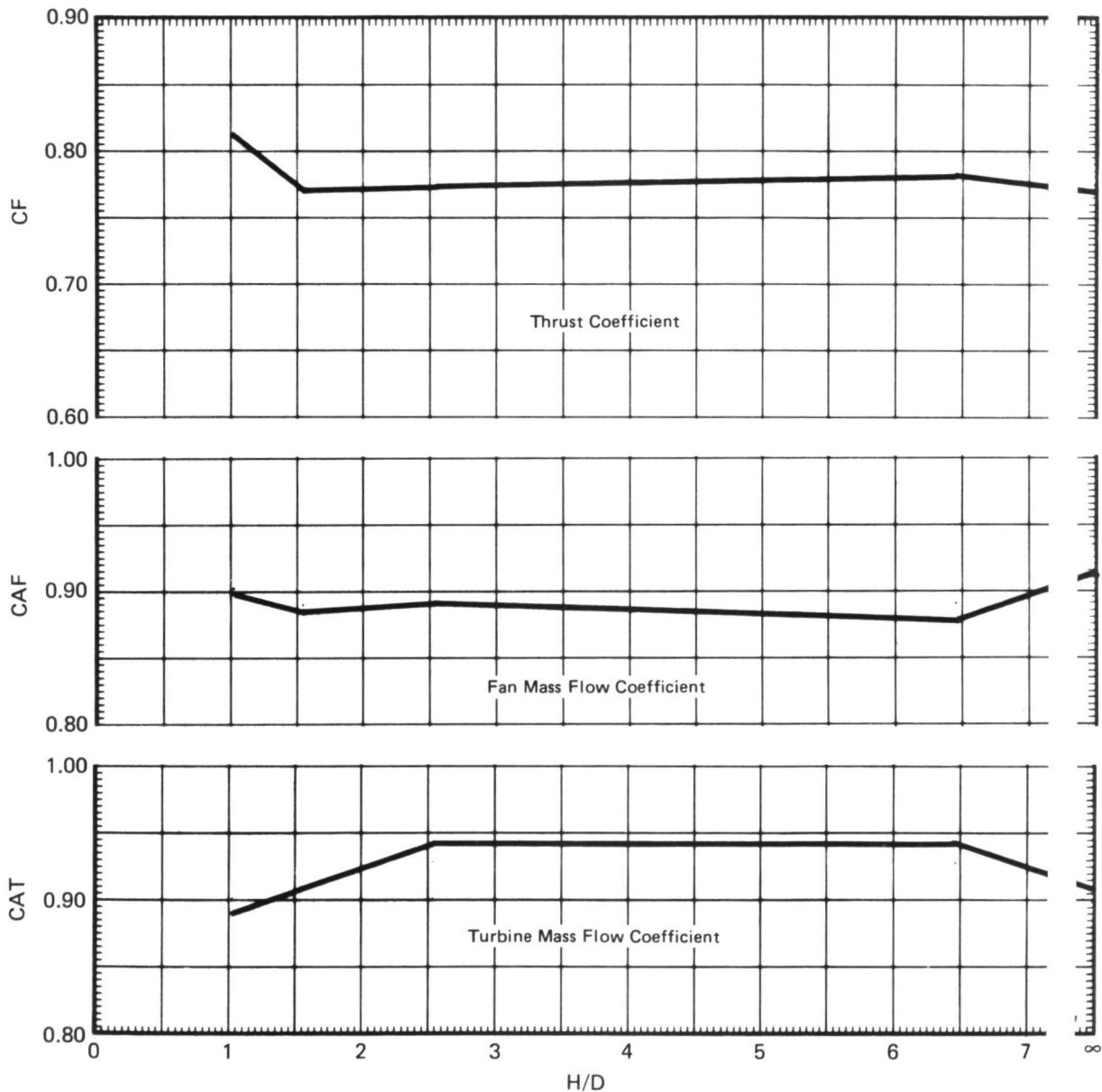
FIGURE 3-4 X376B/T58 NOSE LIFT UNIT FAN EXIT RAKE THRUST AND MASS FLOW COEFFICIENTS \delta_{NL} = 95^\circ \delta_Y = 0^\circ N_F/\sqrt{\theta T_i} = 3600 \text{ RPM} Hemispherical Hub
