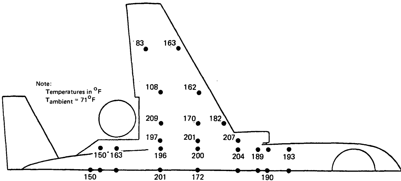
FIGURE 4-57 LOWER SURFACE TEMPERATURE DISTRIBUTION Baseline Configuration H/D = 1.53
