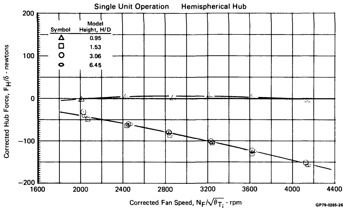
FIGURE 4-38 NOSE UNIT EXIT HUB FORCE
