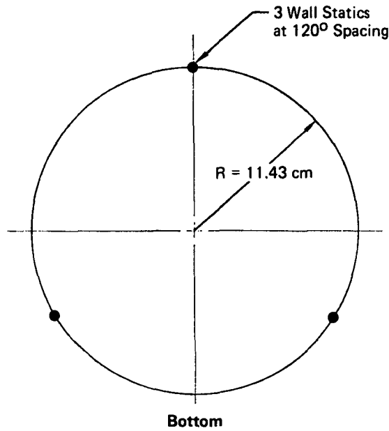
FIGURE 2-24 ENGINE EXIT INSTRUMENTATION
