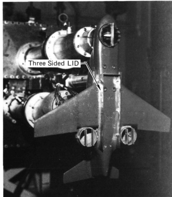
FIGURE 2-31 4.1 PERCENT SCALE MODEL LID APPARATUS
