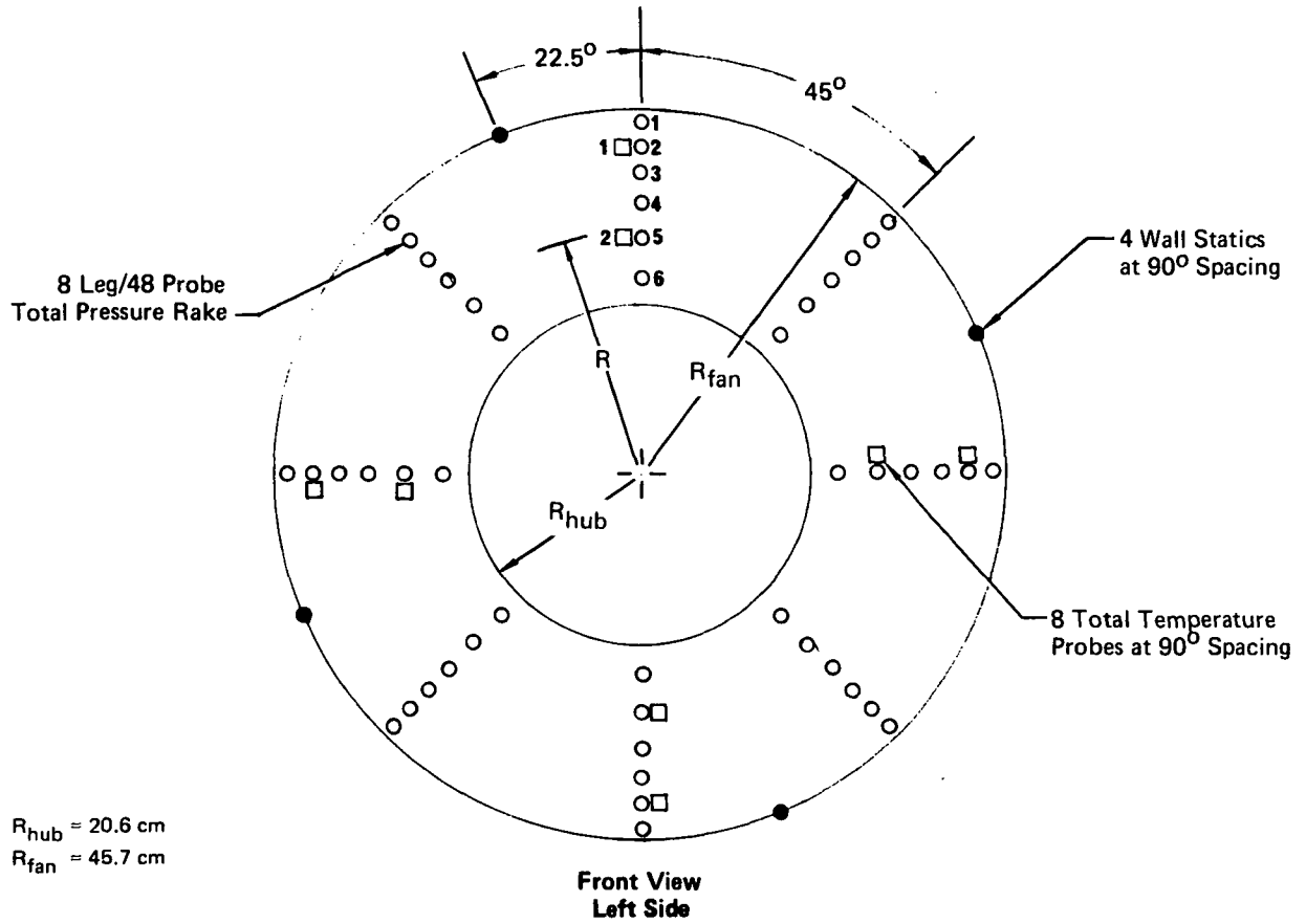
Thermocouple Locations
