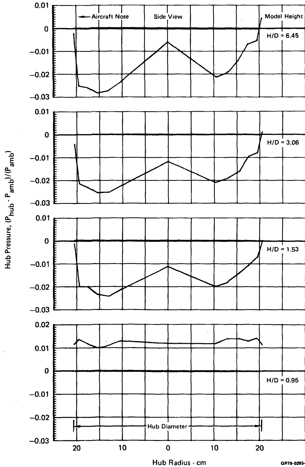
FIGURE 4-40 NOSE UNIT EXIT HUB PRESSURE PROFILES Single Unit Operation Flat Plate Hub N_F/\sqrt{\theta T_i} = 3600 \text{ RPM}
