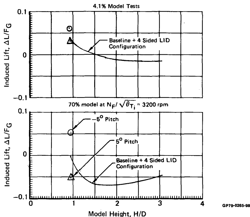
FIGURE 4-33 4-SIDED LID CONFIGURATION 3-Unit Operation
