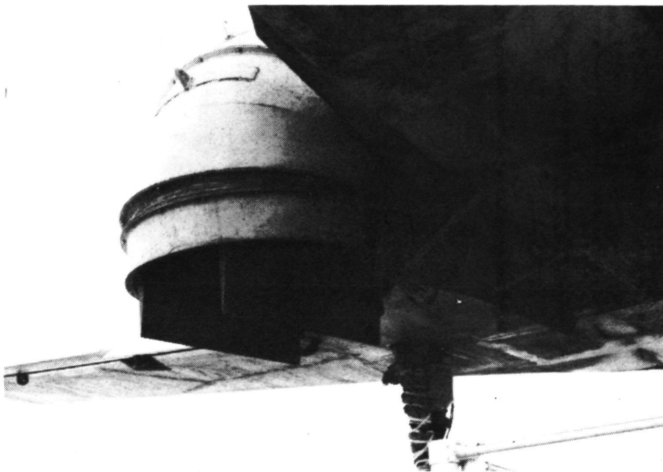
FIGURE 2-13 LIFT/CRUISE NOZZLE RAIL INSTALLATION
