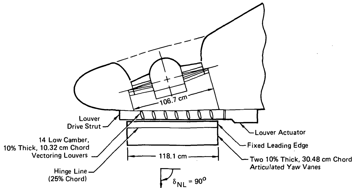
FIGURE 2-7 NOSE LIFT UNIT VECTORING SYSTEM GEOMETRY
