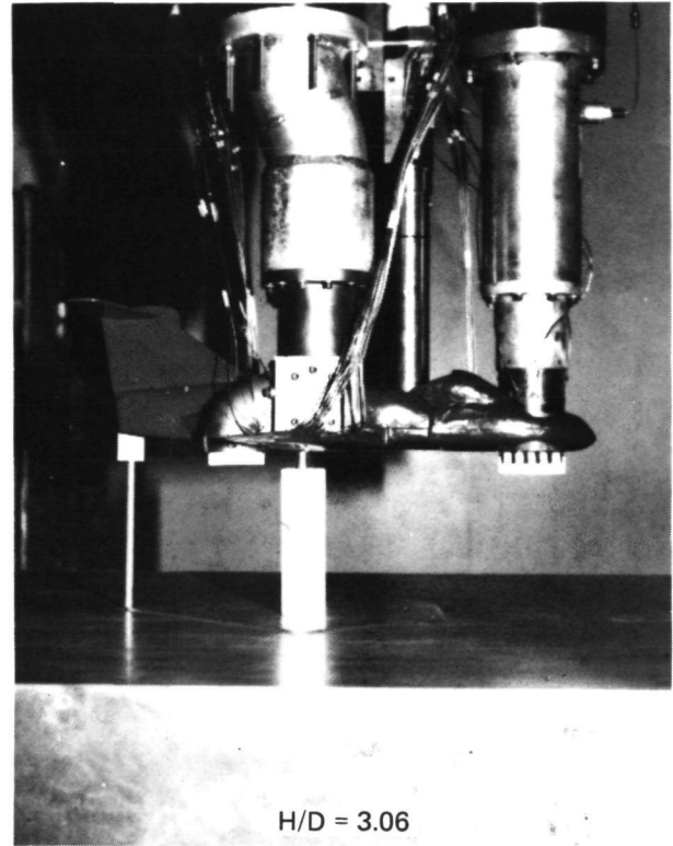
FIGURE 2-30 4.1 PERCENT SCALE MODEL AND STRUT HARDWARE
