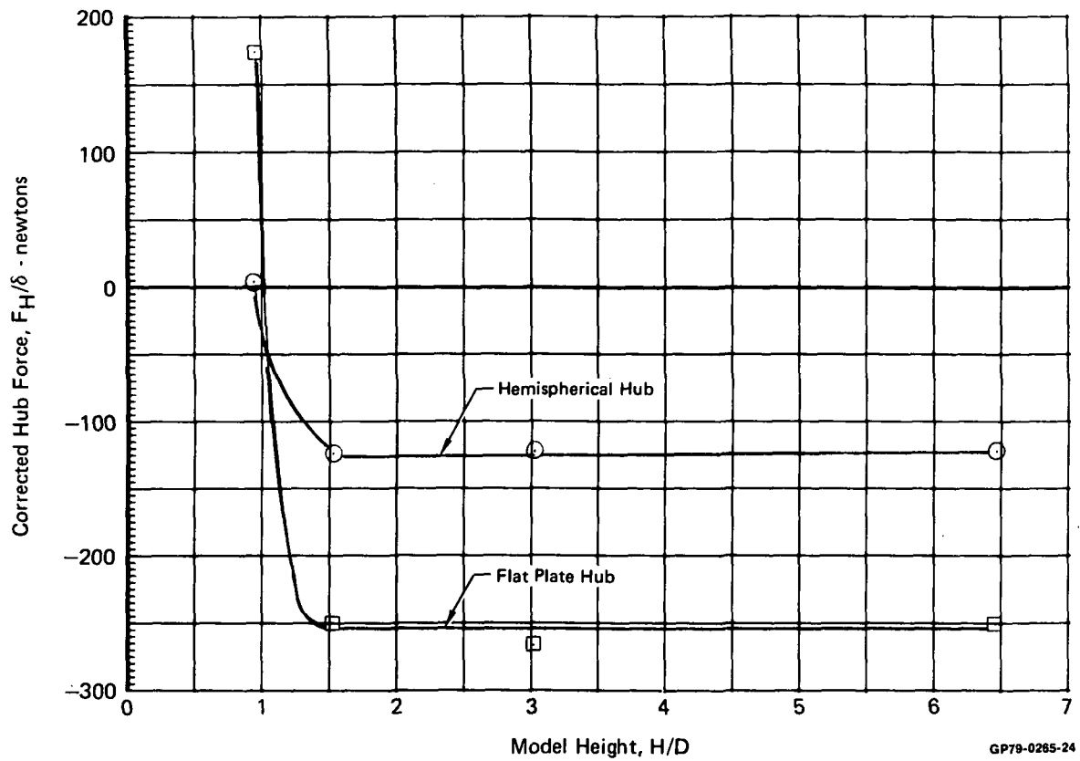
FIGURE 4-39 EFFECT OF GROUND HEIGHT ON NOSE UNIT EXIT HUB FORCE Single Unit Operation N_F/\sqrt{\theta_{T_i}} = 3600 \text{ RPM}
