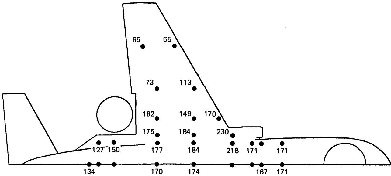
FIGURE 4-56 LOWER SURFACE TEMPERATURE DISTRIBUTION Baseline Configuration H/D = 0.95
