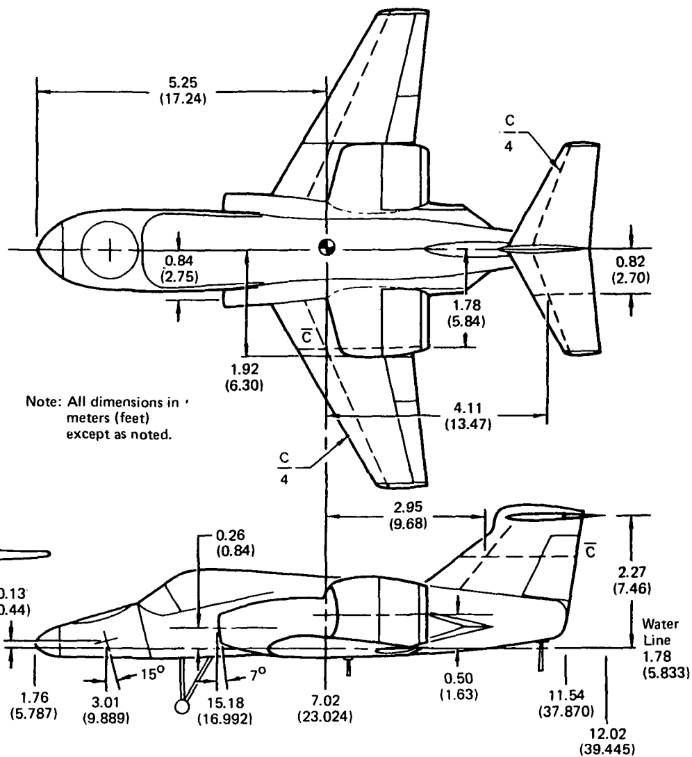
FIGURE 2-2 LARGE SCALE POWERED MODEL Basic Geometry
