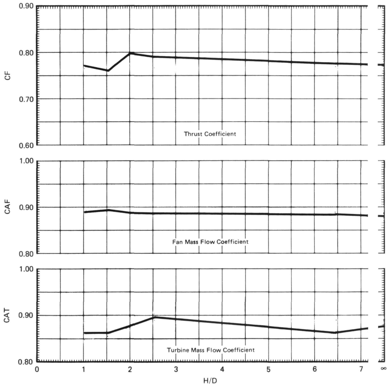
FIGURE 3-2 X376B/T58 RIGHT LIFT/CRUISE UNIT FAN EXIT RAKE THRUST AND MASS FLOW COEFFICIENTS \delta_{LC} = 95^\circ , \delta_Y = 0^\circ N_F/\sqrt{\theta T_i} = 3600 RPM
