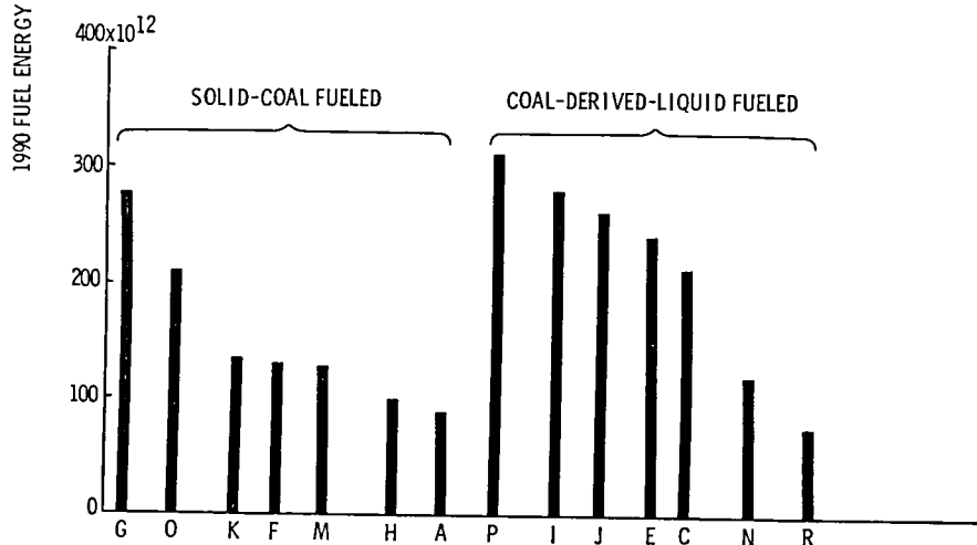
Figure 13. - Potential national energy savings for advanced systems if no export of electricity is allowed. (All values relative to noncogeneration boiler burning residual-grade, coal-derived liquid fuels and coal-fired utility.)
