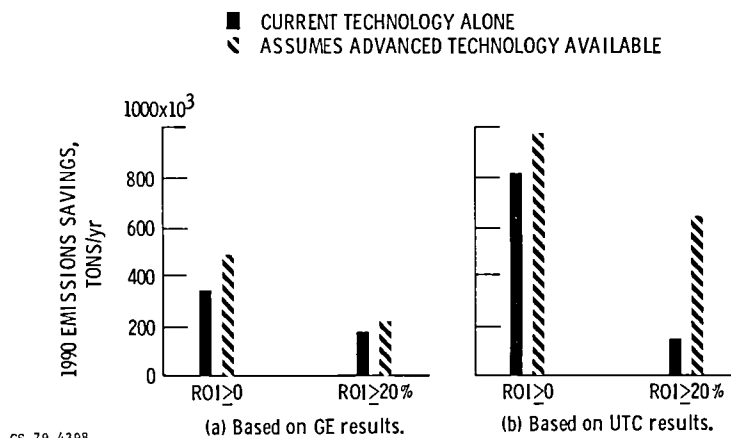
Figure 16. - Potential national emissions savings for current- and advanced-technology cogeneration systems. (All values relative to noncogeneration boiler burning residual-grade, coal-derived liquid fuels and coal-fired utility.)
