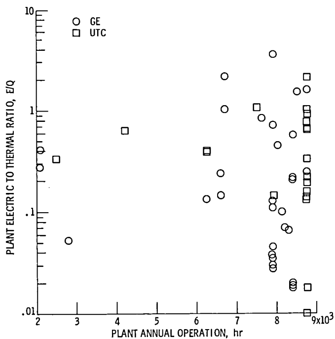
Figure 8. - Load factors for CTAS processes.
