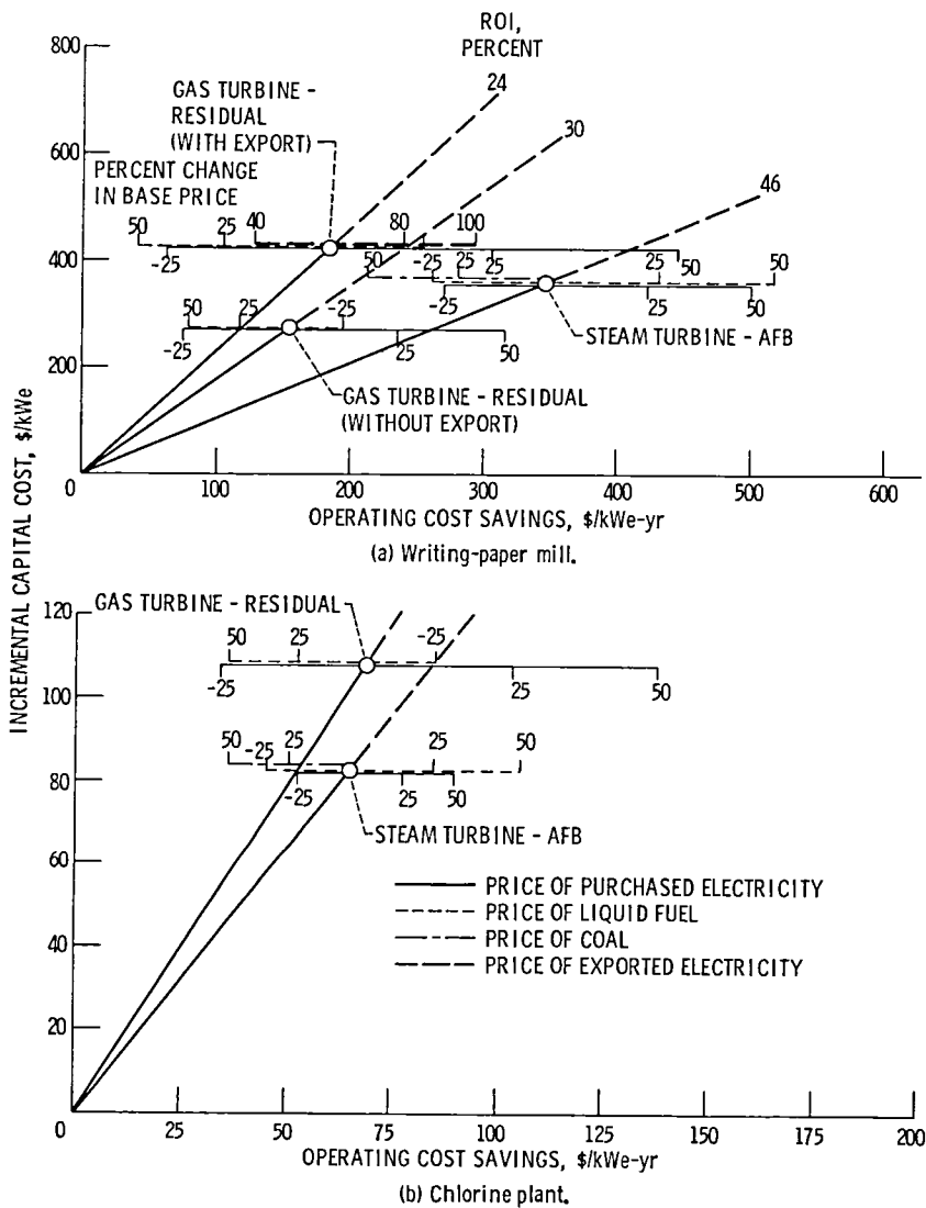
Figure 20. - Examples of sensitivity of cogeneration system economics to variations in fuel and electricity prices. (All values relative to noncogeneration boiler burning residual-grade, coal-derived liquid fuels and coal-fired utility.)
