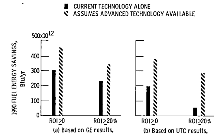
Figure 15. - Potential national fuel energy savings of current- and advanced-technology cogeneration systems. (All values relative to noncogeneration boiler burning residual-grade, coal-derived liquid fuels and coal-fired utility.)
