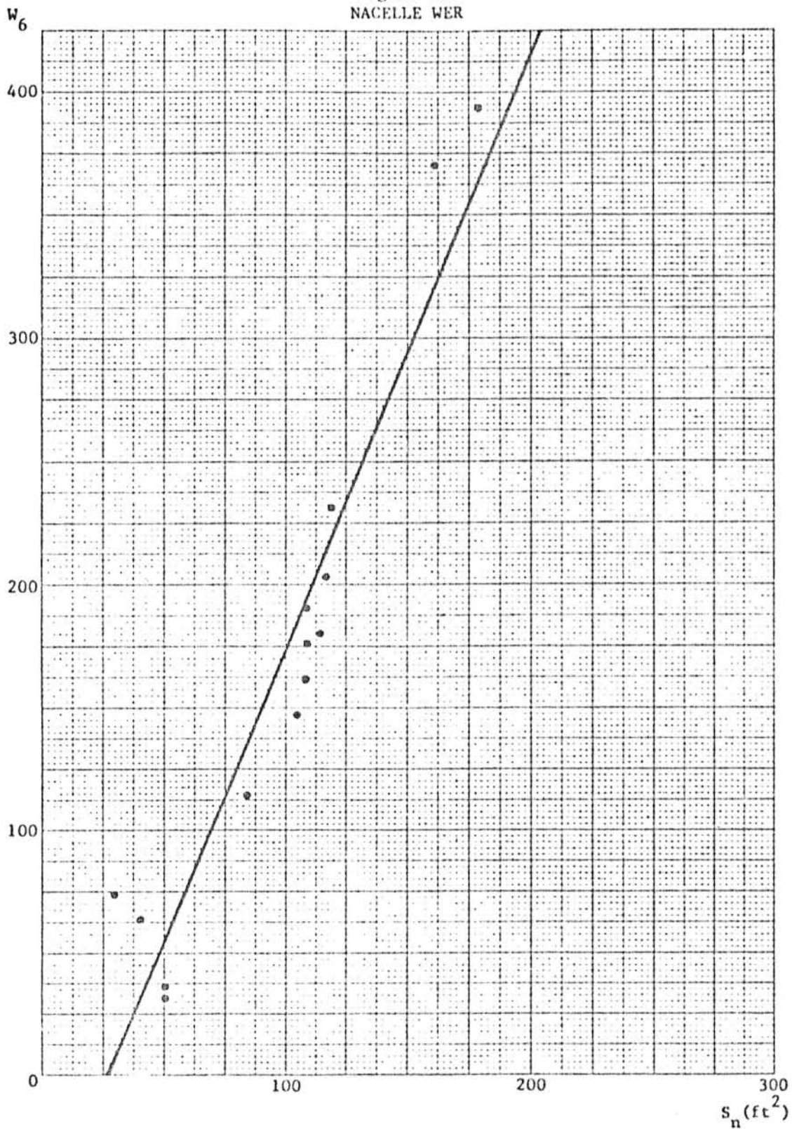
Figure 4.4 NACELLE WER
