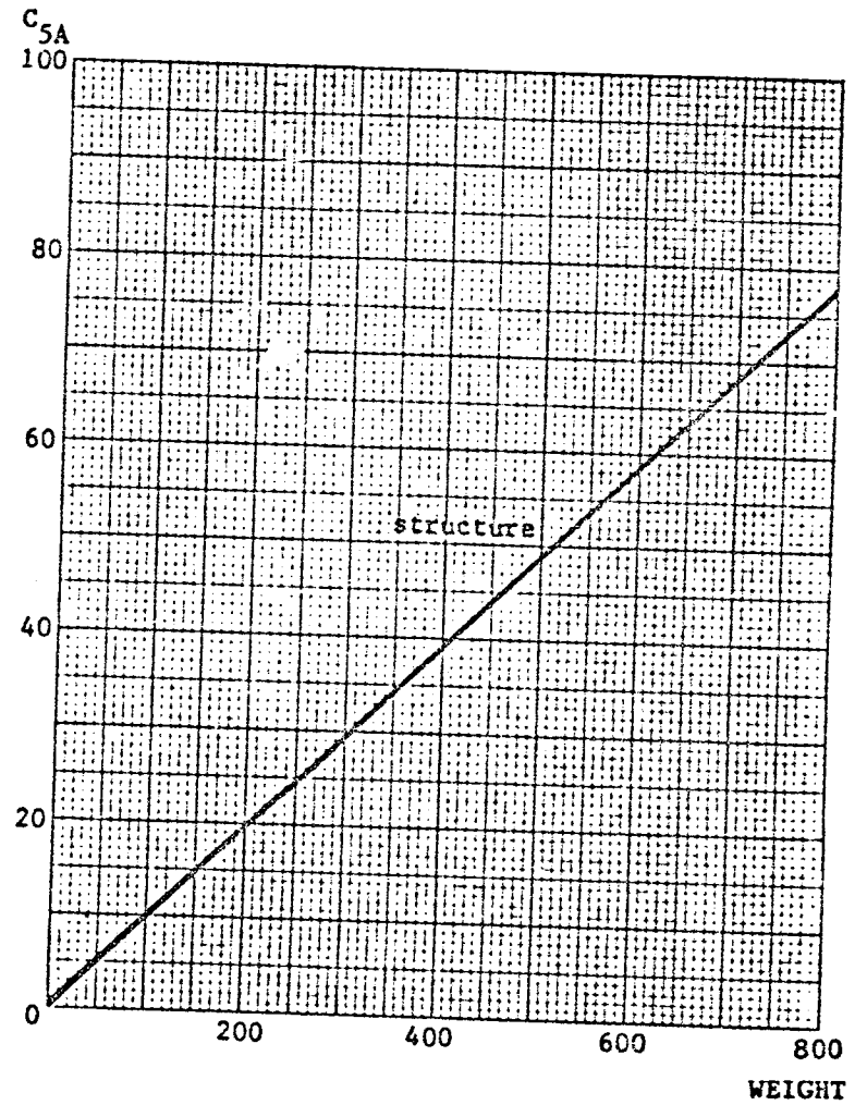
Figure 5.5 ALIGNING GEAR CERs (Thousands of $FY77)
