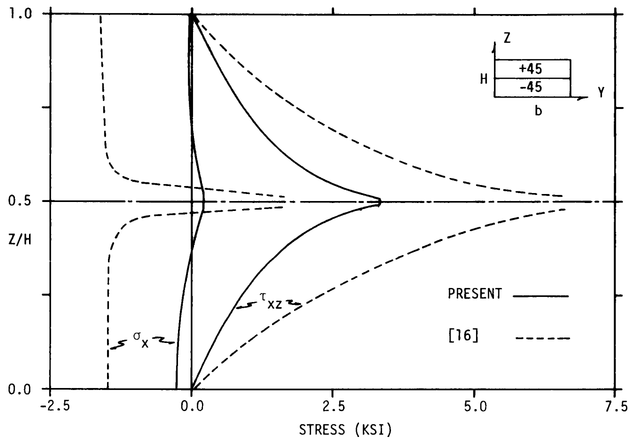
FIGURE 25. THROUGH-THE-THICKNESS DISTRIBUTIONS FOR THE RESIDUAL \sigma_x AND \tau_{xz} ALONG THE FREE EDGE IN A [\pm 45]_5 GR/E LAMINATE
