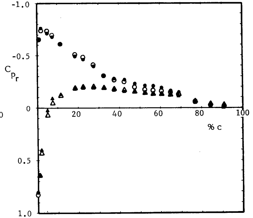
(b) r/R = 0.966 ; y/c = 0.163
