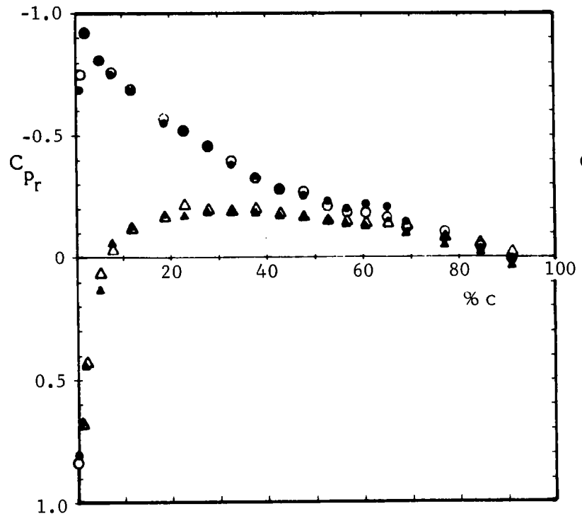
(a) r/R = 0.940 ; y/c = 0.288
