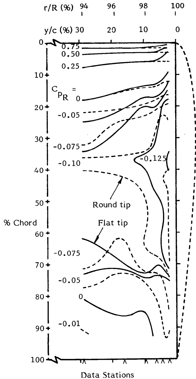
(a) Lower surface
