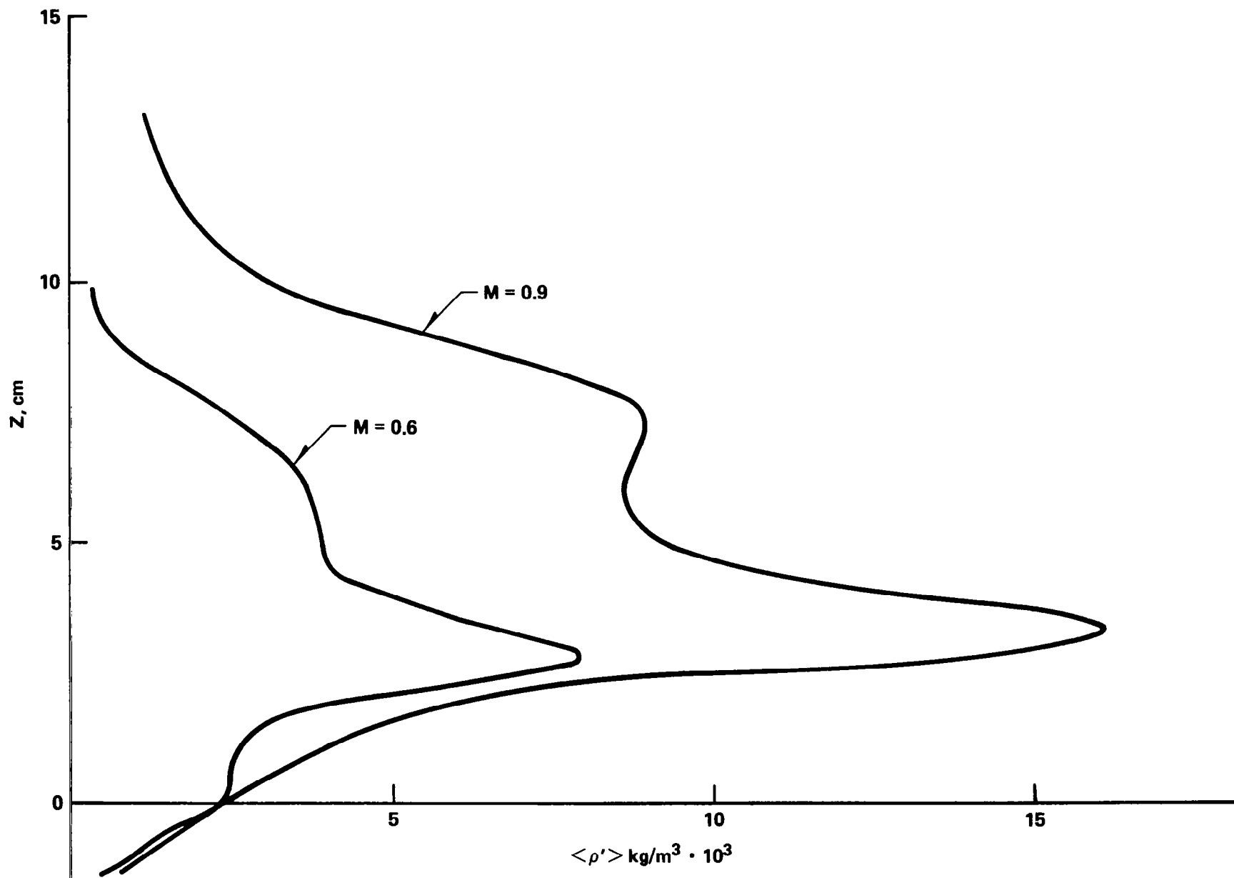
Figure 2. Density Fluctuations. c) Configuration 13.
