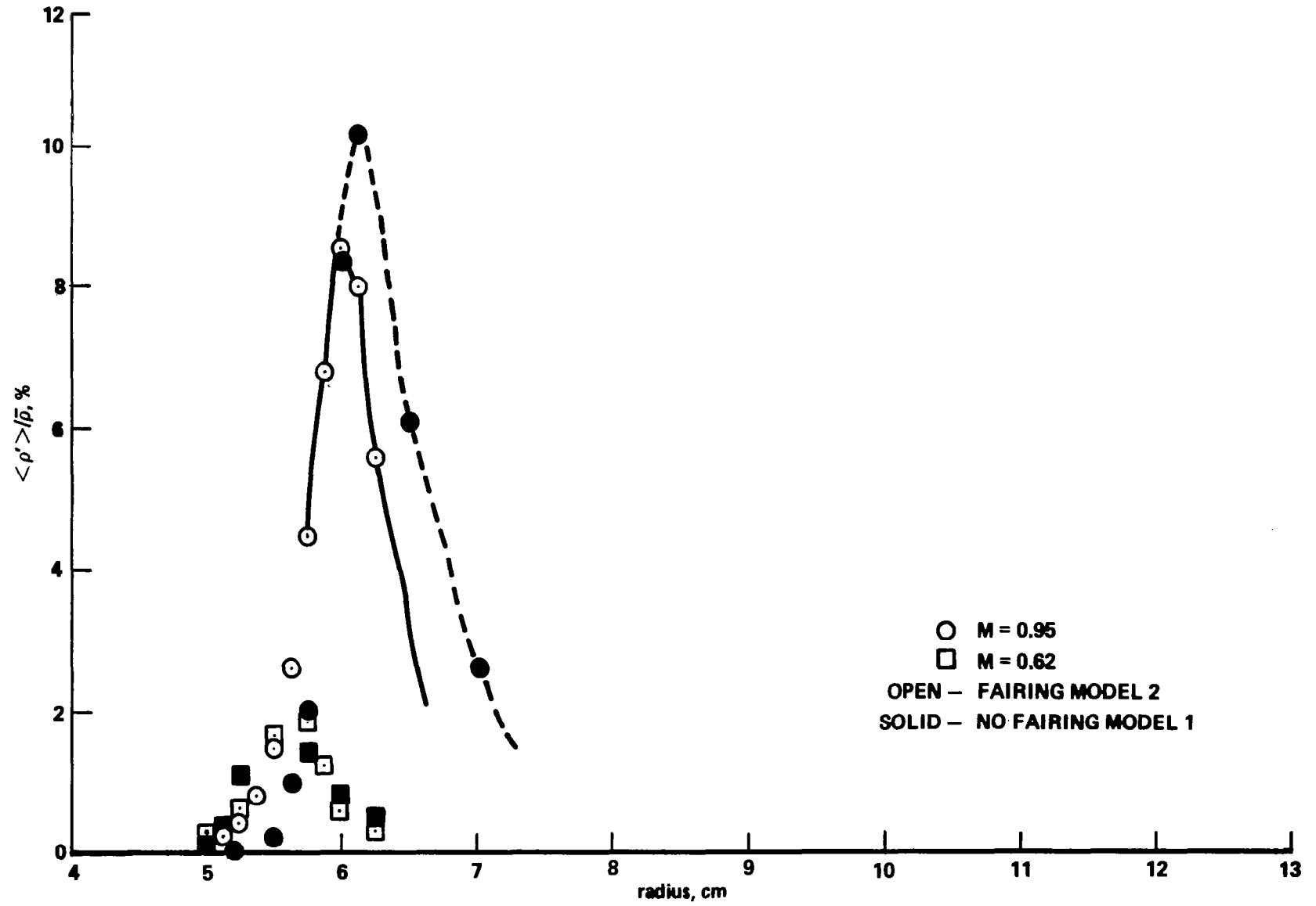
Figure 8. Effect of Fairing on Density Fluctuations at \theta = 120^\circ .
