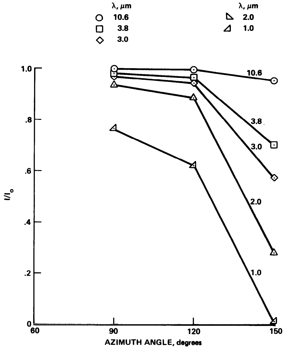
Figure 10. Effect of Wave Length on Optical Performance.
