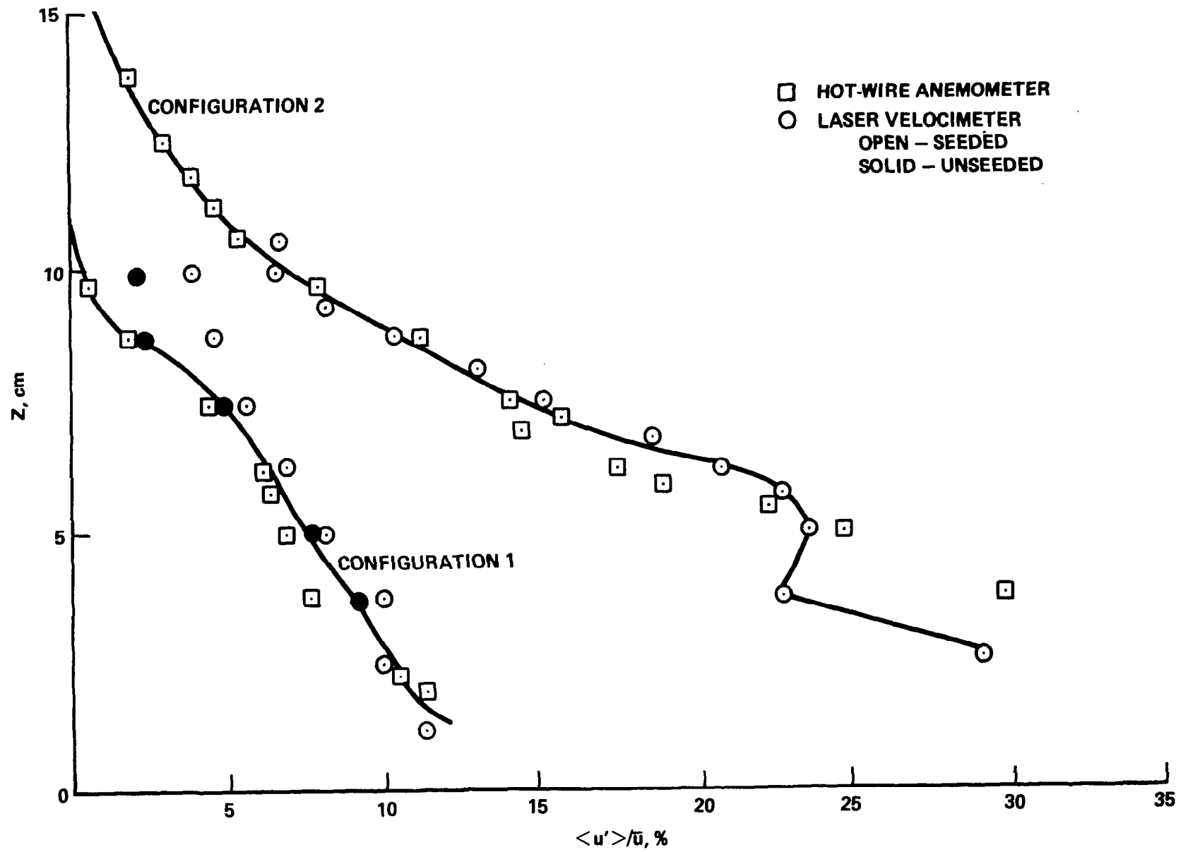
Figure 1. Velocity Fluctuations in Boundary and Shear Layers.
