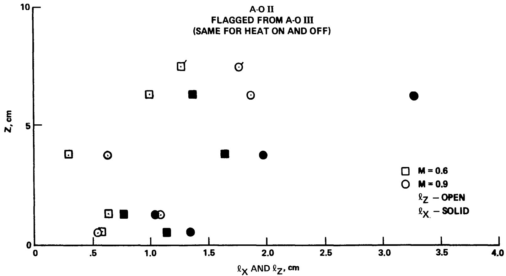
Figure 3. Correlation Lengths. b) Configuration 13.
