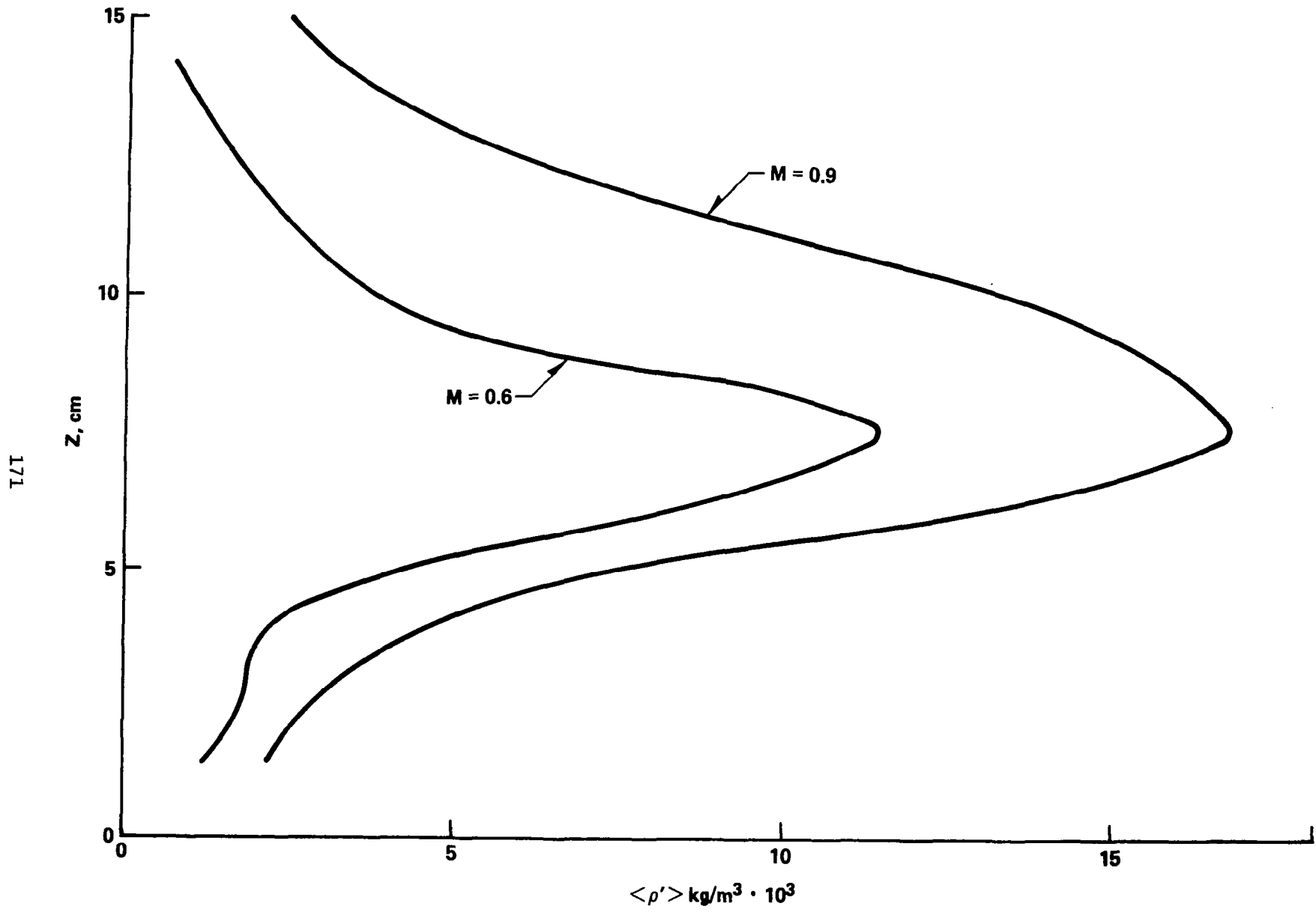
Figure 2. Density Fluctuations. b) Configuration 2.
