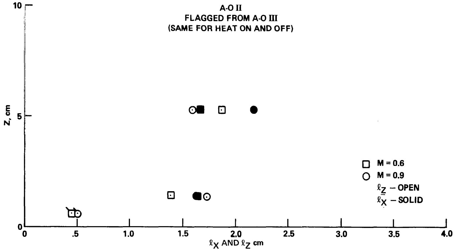
Figure 3. Correlation Lengths. a) Configuration 1.
