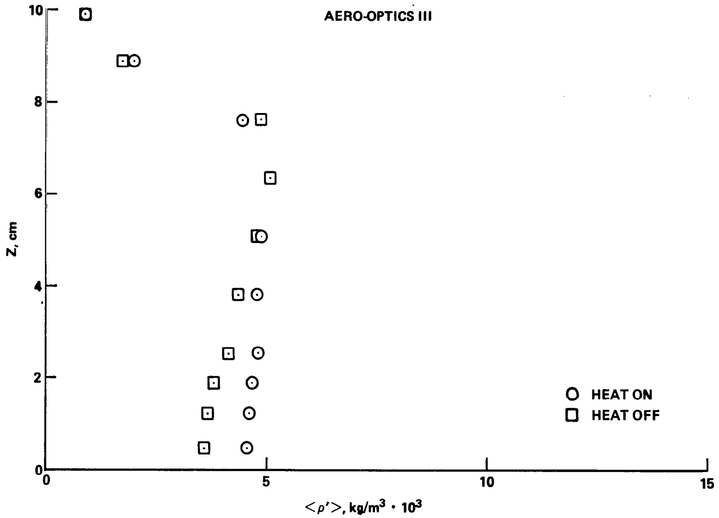
Figure 6. RMS Density Fluctuations, Config. 1, M = 0.9 .
