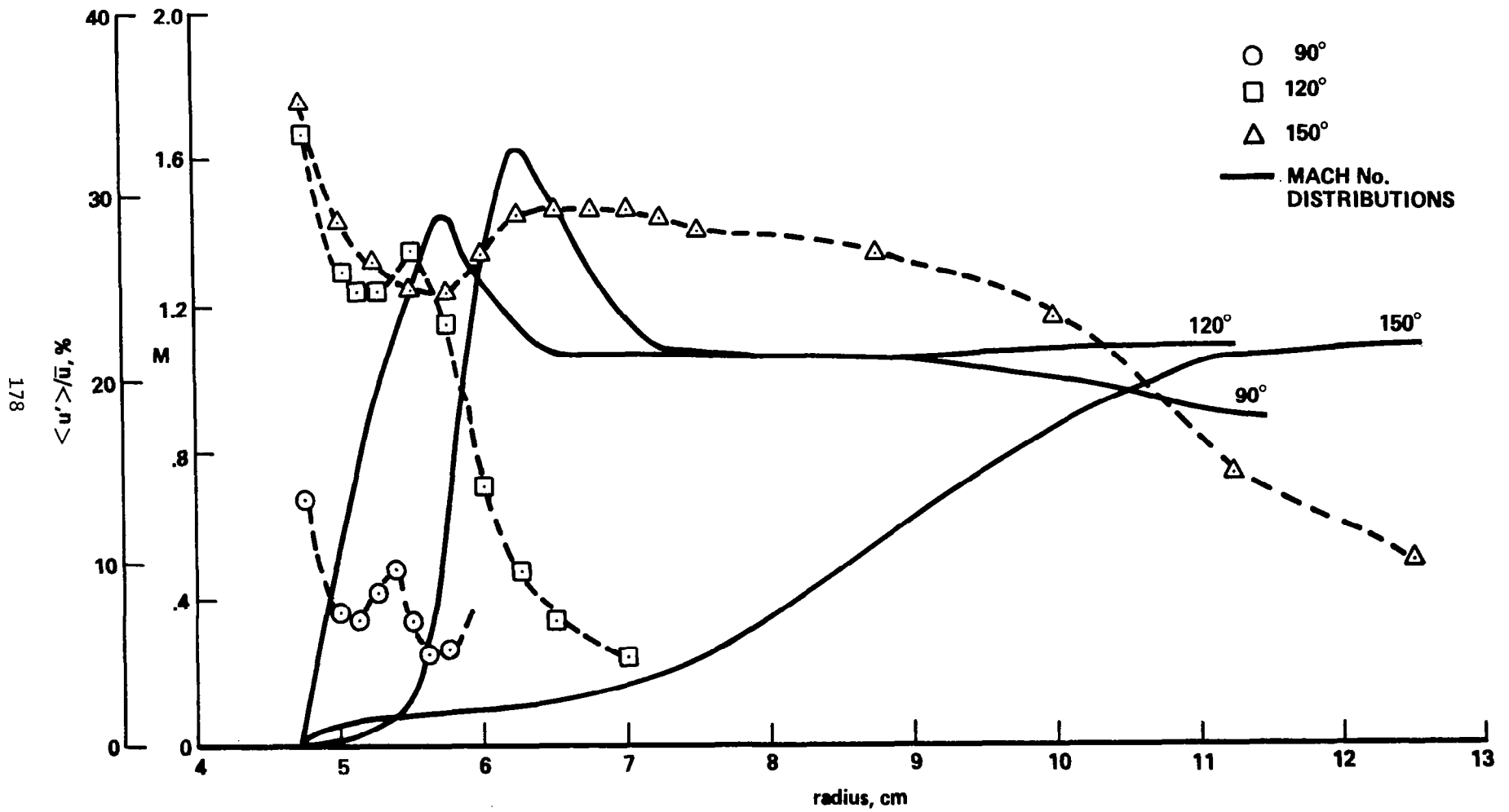
Figure 7. Kinematic (Velocity) Fluctuations and Mean Profiles from A-O IV.
