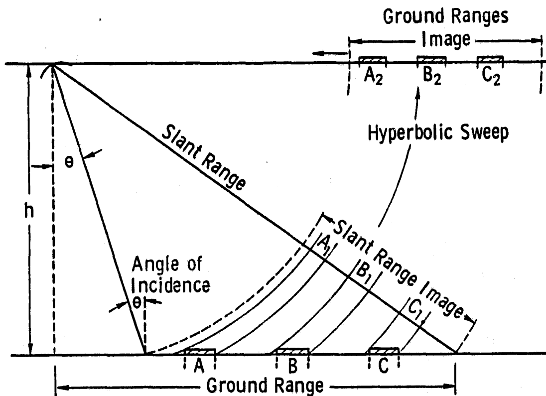
Figure 9. Range Compression
