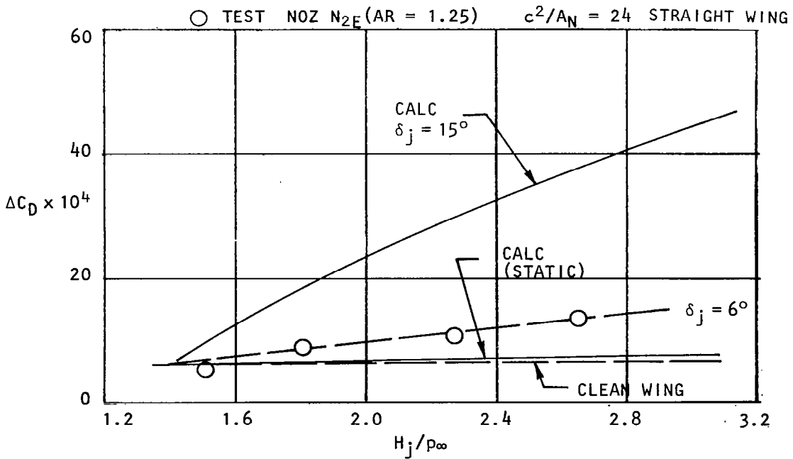
Figure 16. Variation of scrubbed area pressure drag with pressure ratio, \alpha = 2^\circ , M_\infty = 0.68 .
