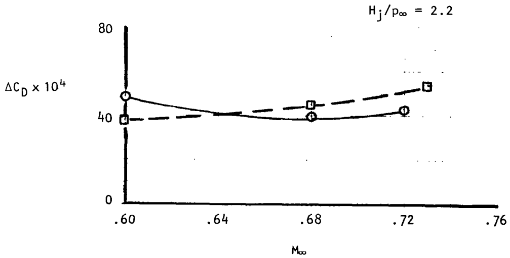
Figure 76. Comparison of streamlined and symmetrical nacelle drag, C_{LM} = 0.40 .
