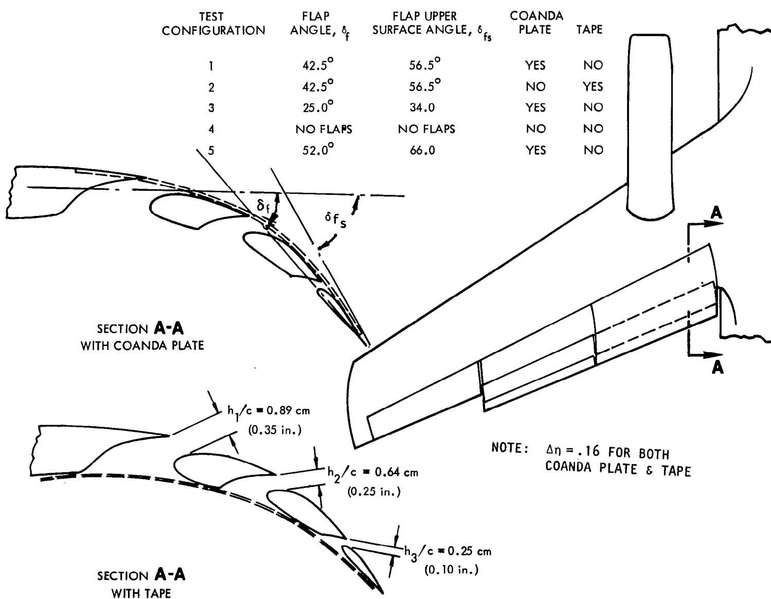
Figure 101. Trailing edge flap system design details, low speed model
