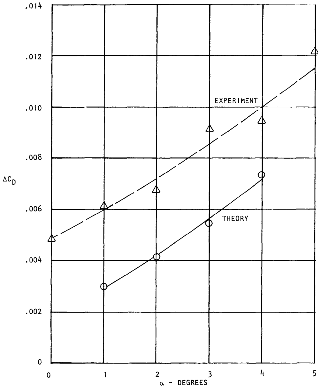
Figure 91. Comparison between predicted and measured drag increments for nacelle N 3E (D-Duct), c^2/A_N = 24 , M_\infty = 0.60 , H_j/p_\infty = 2.0
