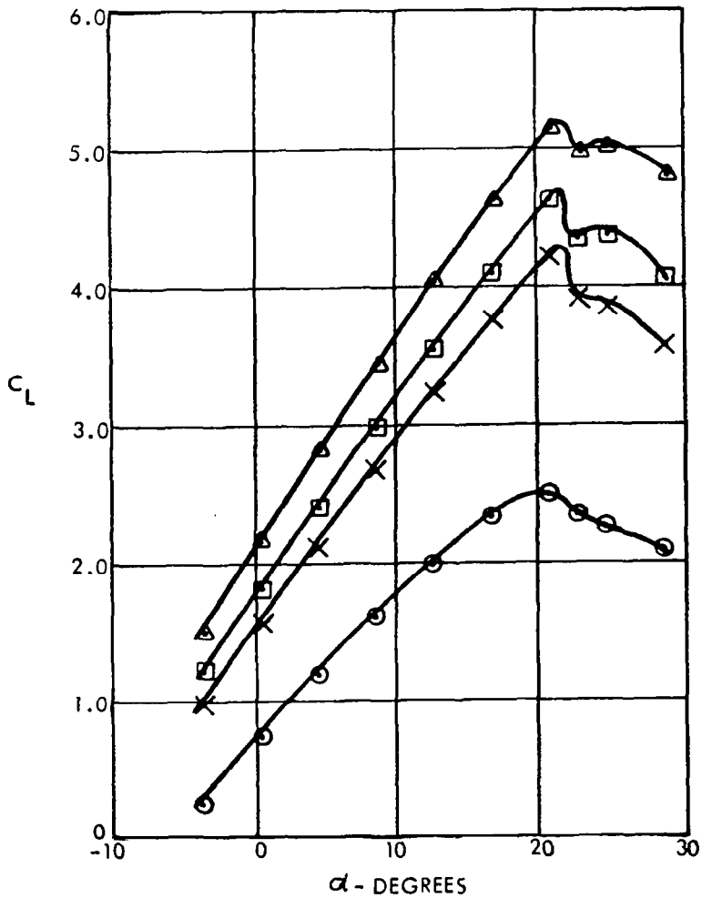
Figure 107. Variation of low speed model lift coefficient with angle of attack, q_{\infty} = 718.2 \text{ N/m}^2 (15 lb/ft 2 ), \delta_f = 25^\circ , Coanda plate
