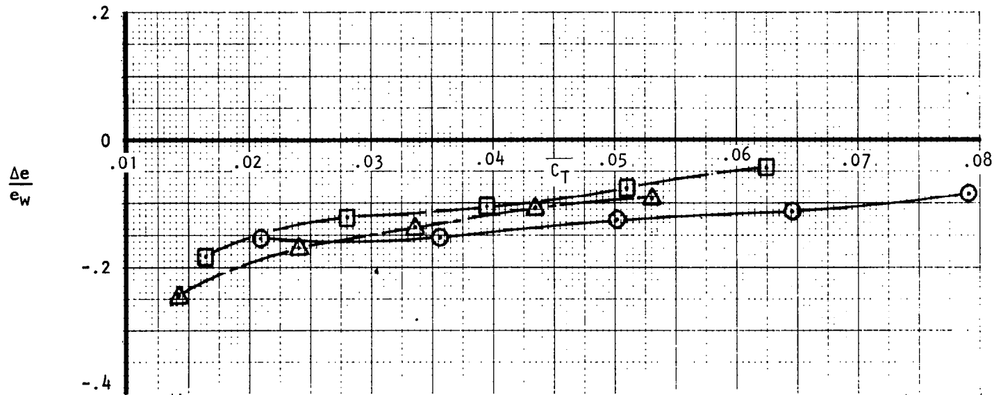
Figure 54. Variation of effective drag-due-to-lift parameter with thrust and Mach no., nozzle N_{12} , AR = 4 .
