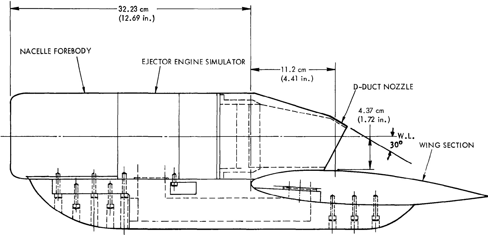
Figure 102. Nacelle installation on the wing
