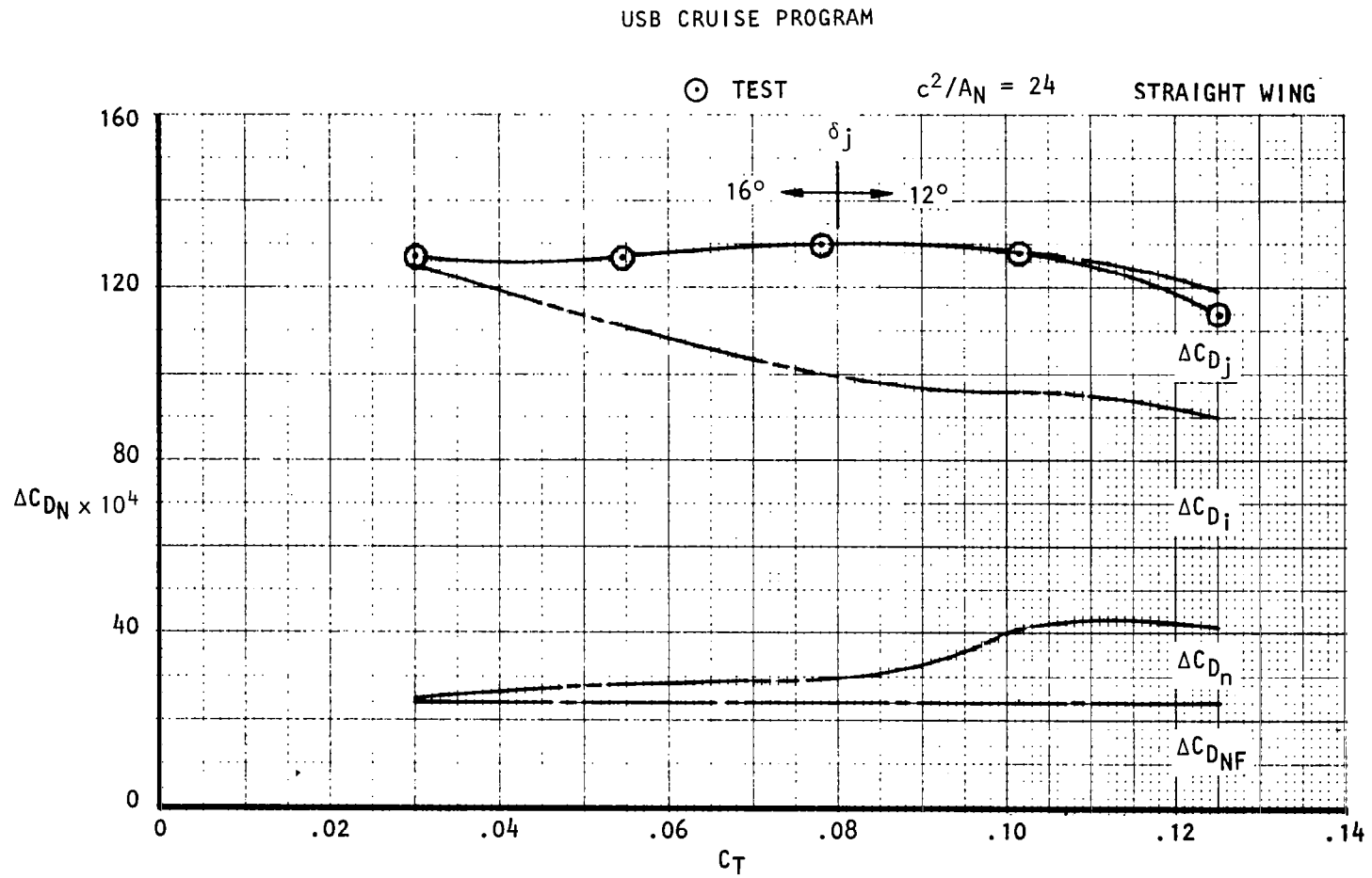
Figure 59. Incremental nacelle drag and component build-up noz N_5 , AR = 6 , M_\infty = 0.68 , C_{LM} = 0.40
