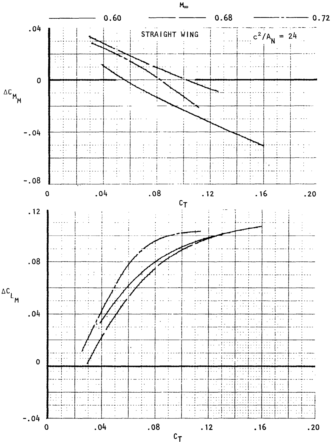
Figure 46. Variation of lift and moment increments due to blowing, noz N_{4E} , AR = 4.
