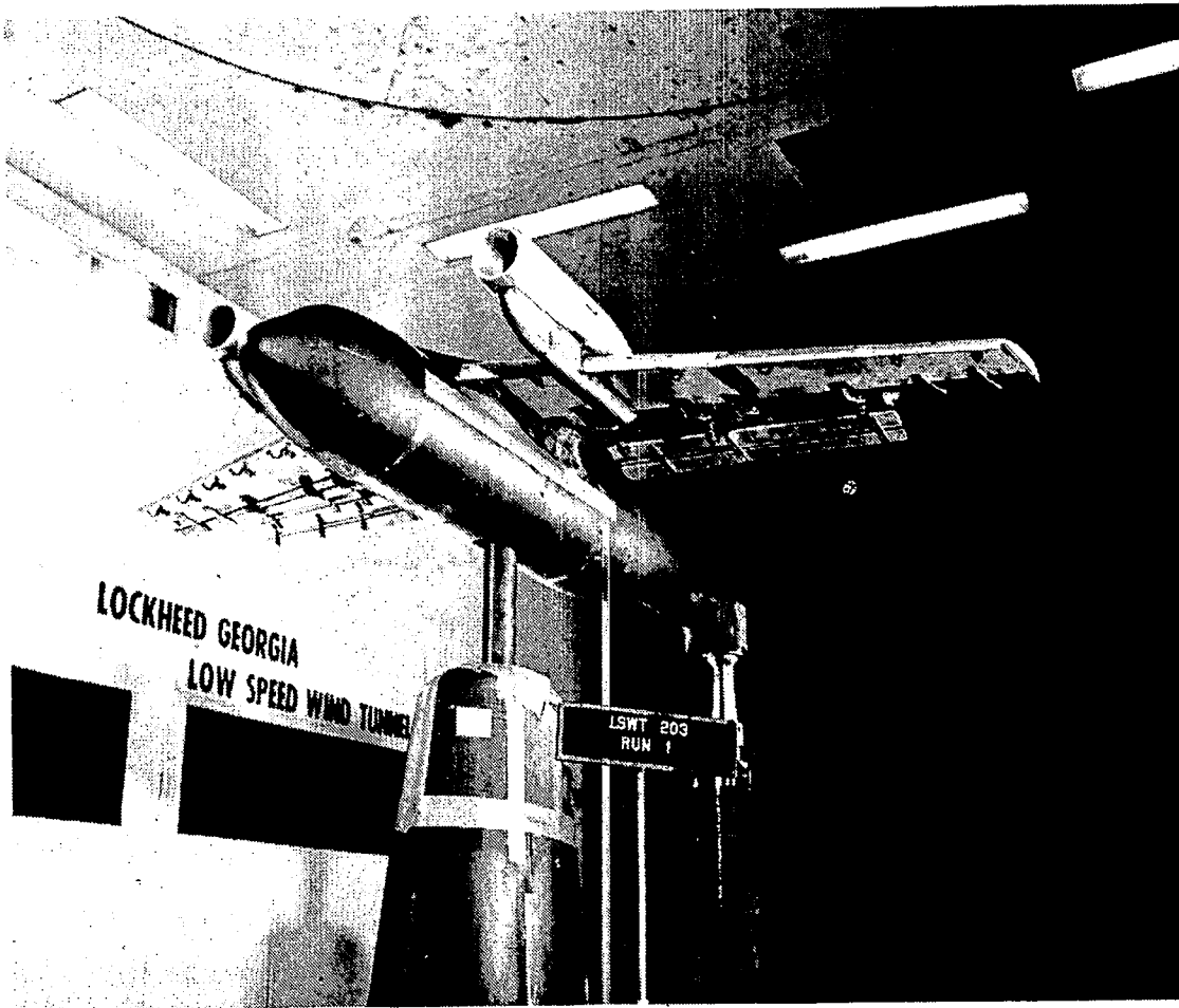
Figure 100. Low-speed, high-lift test model.
