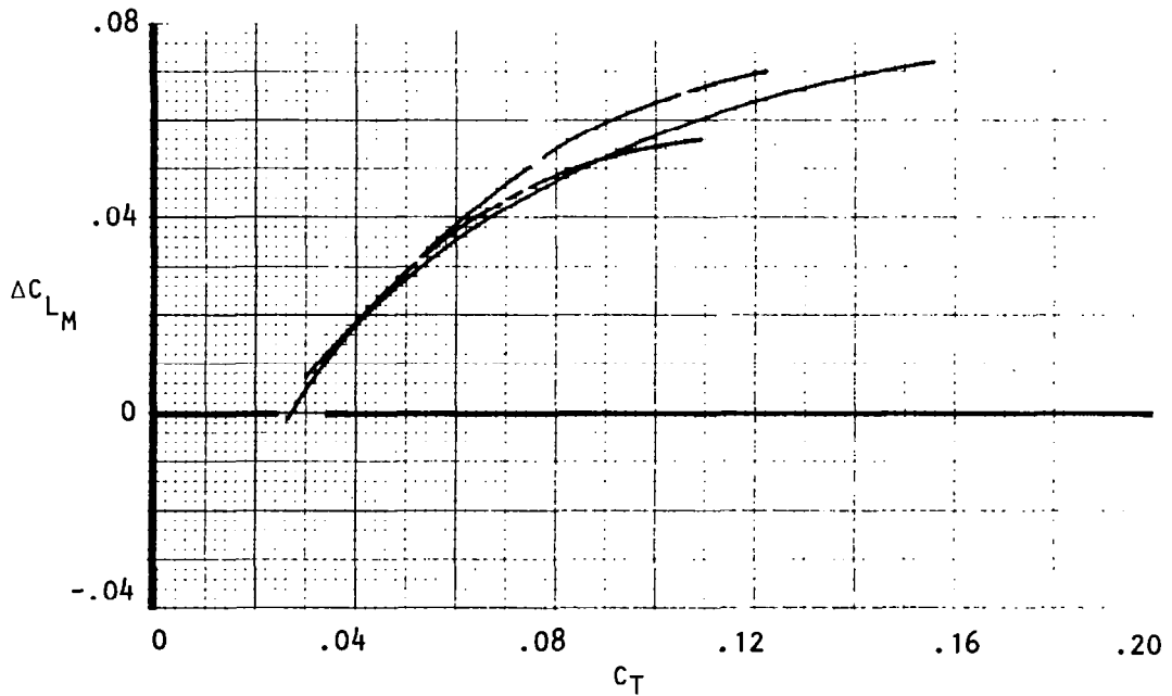
Figure 44. Variation of lift and moment increments due to blowing, noz N_{3E} , AR = 2.5.
