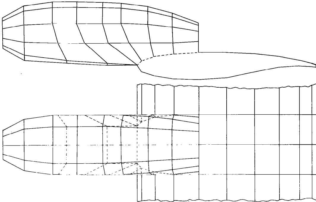
Figure 82. Panel details for D-duct nacelle and adjacent wing.
