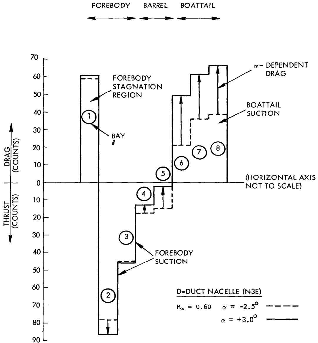
Figure 88. Computed drag count distribution along nacelle axis (Nacelle Surfaces Only).
