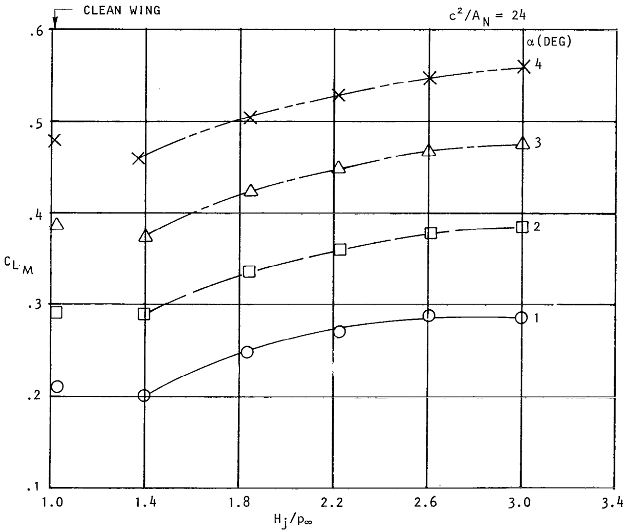
Figure 28. Effect of nozzle pressure ratio on total lift, noz N 5 , AR = 6.0, M ∞ = 0.68.
