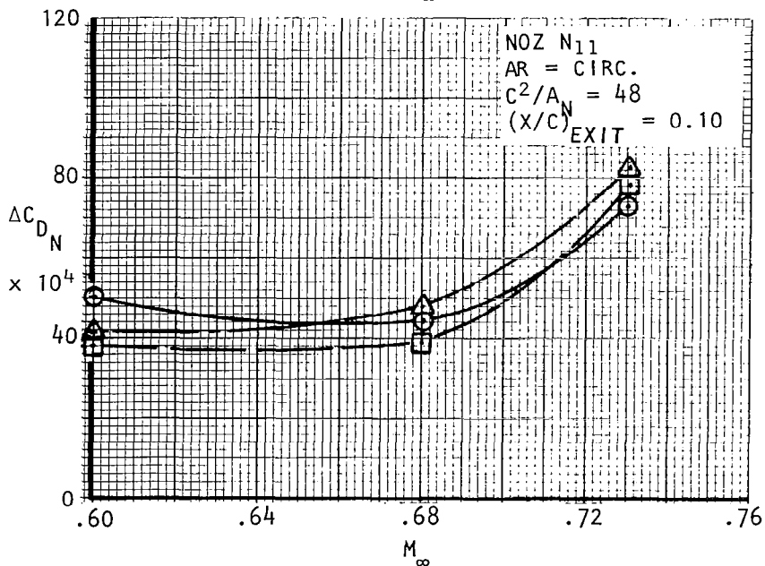
Figure 39. Effect of Mach number on nacelle drag coefficient, C_{L_M} = 0.40
