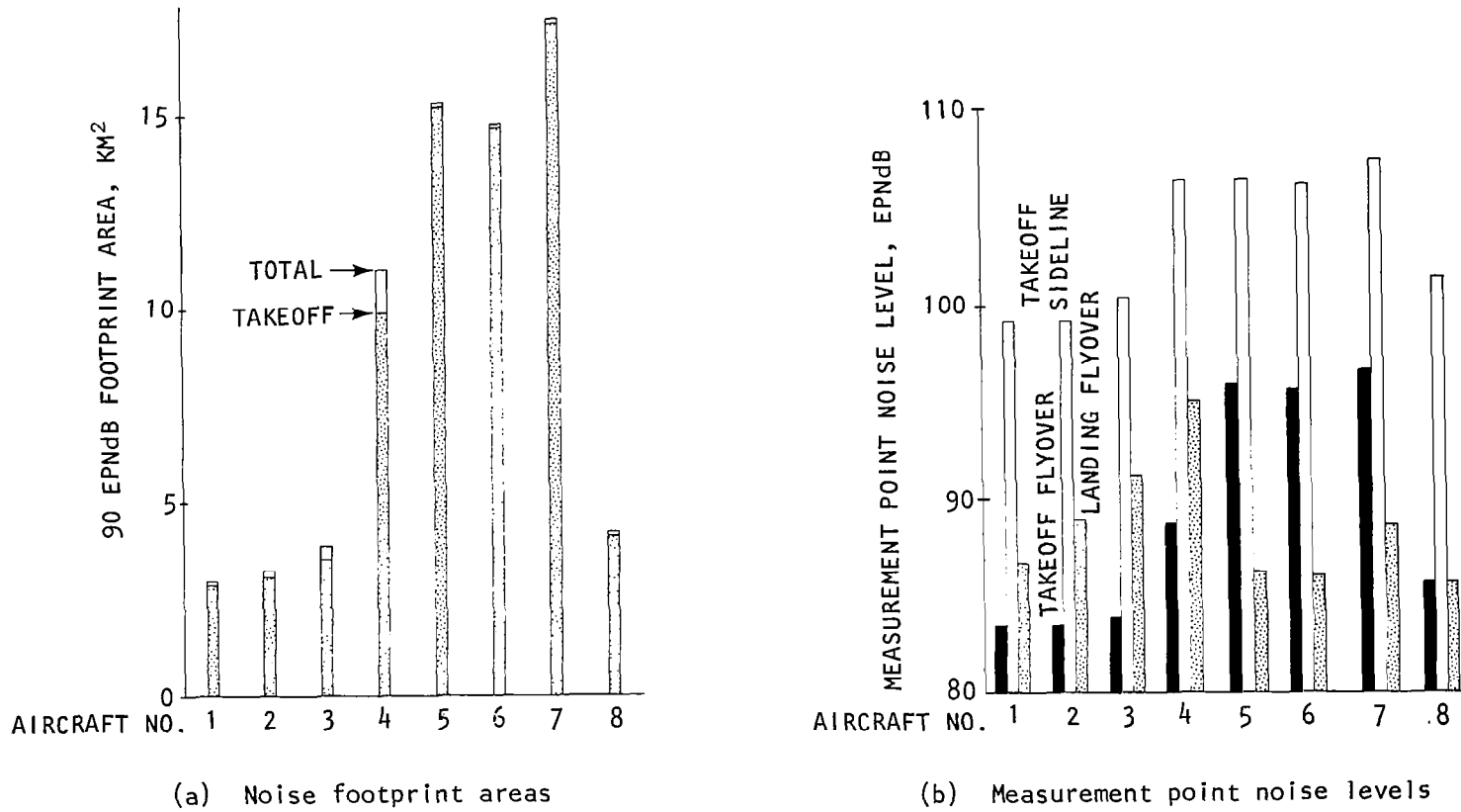
Figure 94. Noise footprint and measurement point noise levels, USB study aircraft
