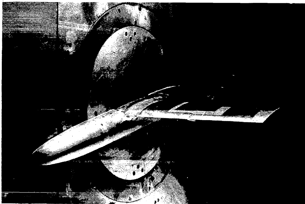
Figure 8. AR 4 nozzle installation on 3-D straight wing force model in 4' x 4' tunnel.
