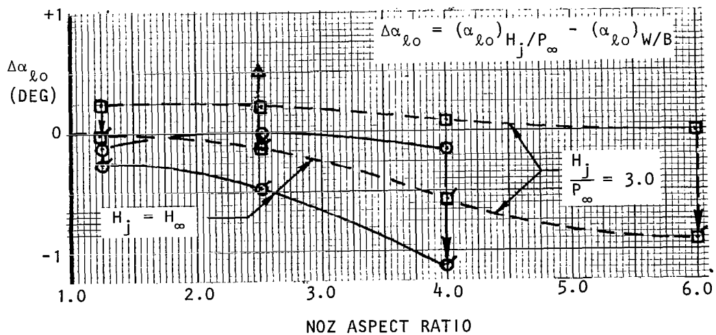
Figure 75. Effect of nacelle installation and blowing on lift, M_\infty = 0.68
