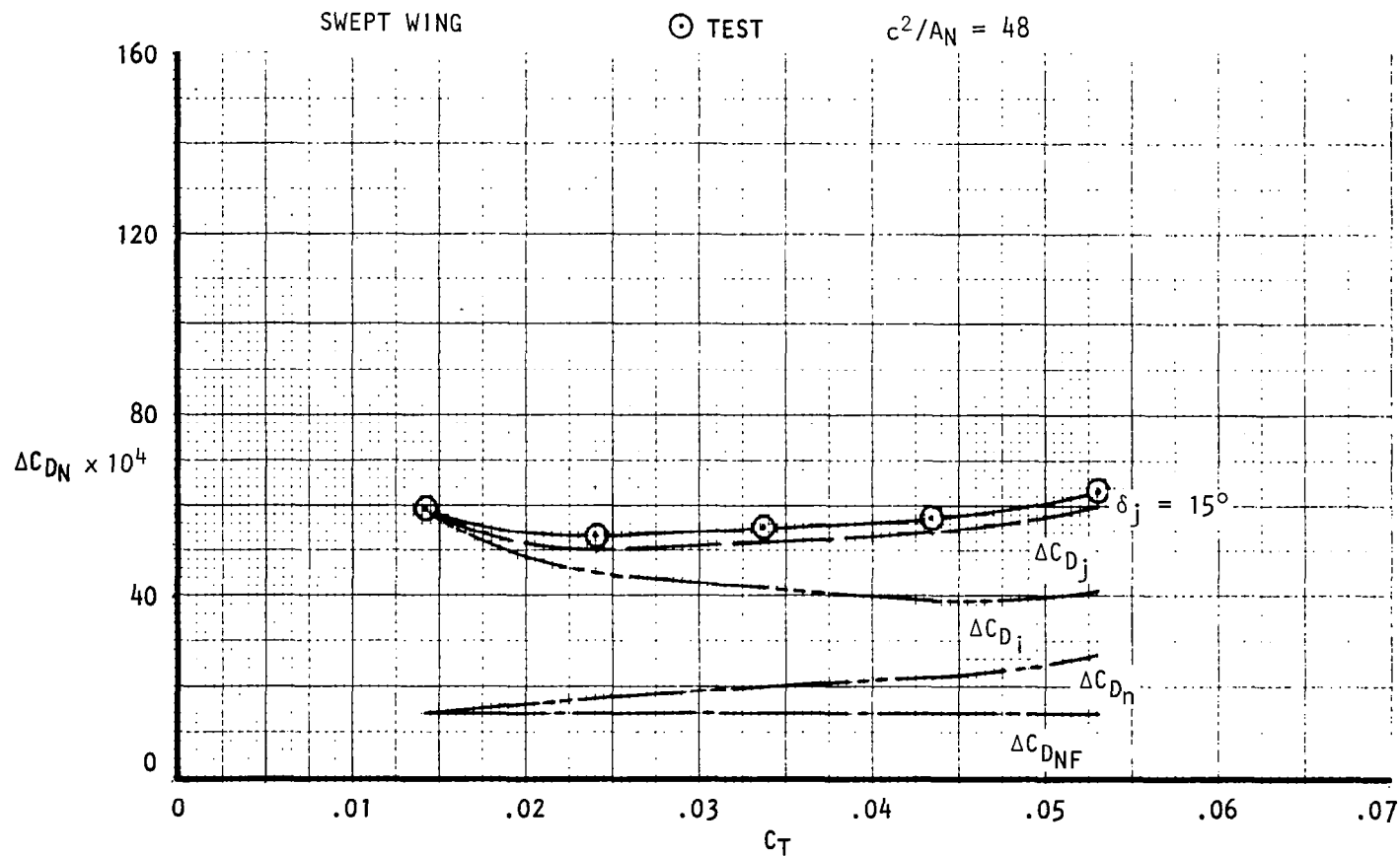
Figure 62. Incremental nacelle drag and component build-up, noz N 12 , AR = 4, M ∞ = 0.73, C LM = 0.40.
