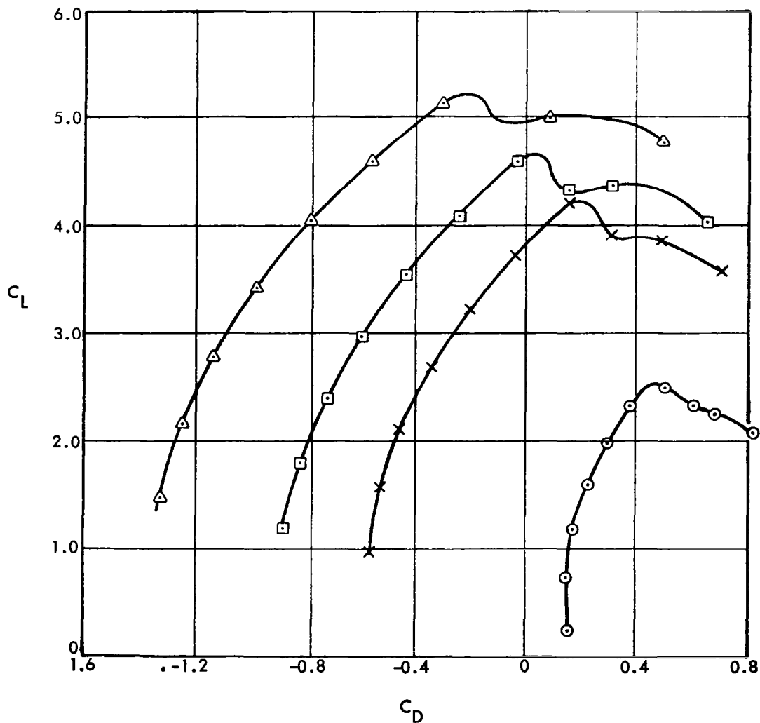
Figure 108. Variation of low speed model lift coefficient with drag coefficient, q_{\infty} = 718.2 \text{ N/m}^2 (15 lb/ft 2 ), \delta_f = 25^\circ , Coanda plate
