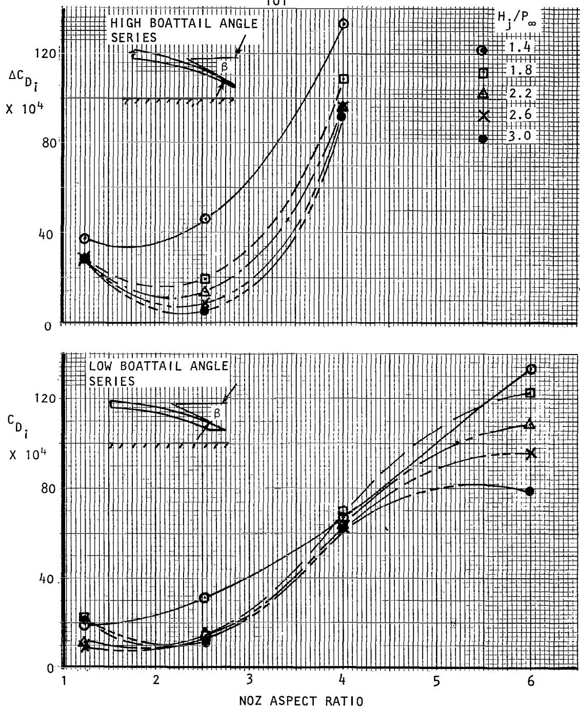
Figure 69. Effect of nozzle exit aspect ratio on lift-dependent drag, M_\infty = 0.68
