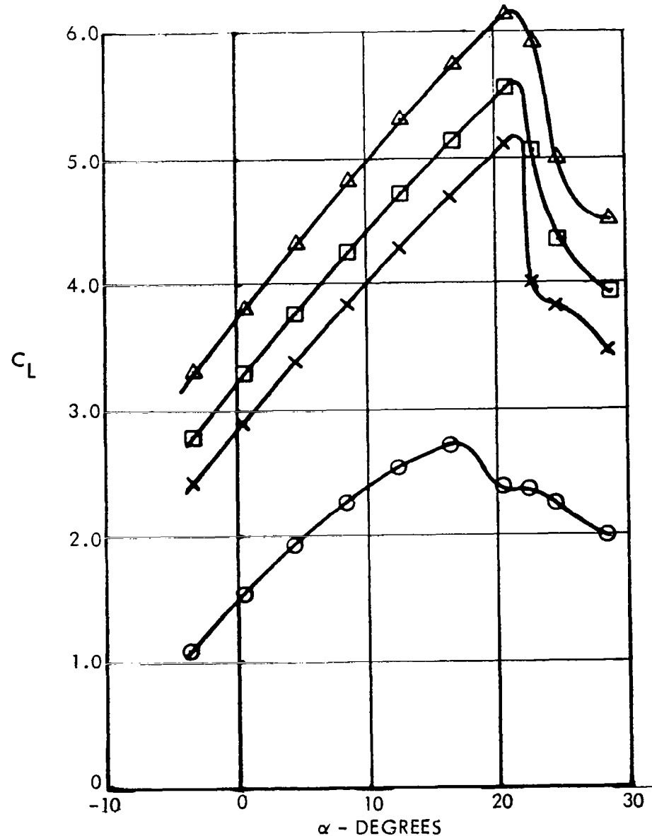
Figure 109. Variation of low speed model lift coefficient with angle of attack, q_{\infty} = 718.2 \text{ N/m}^2 (15 lb/ft 2 ), \delta_f = 52^\circ , Coanda plate
