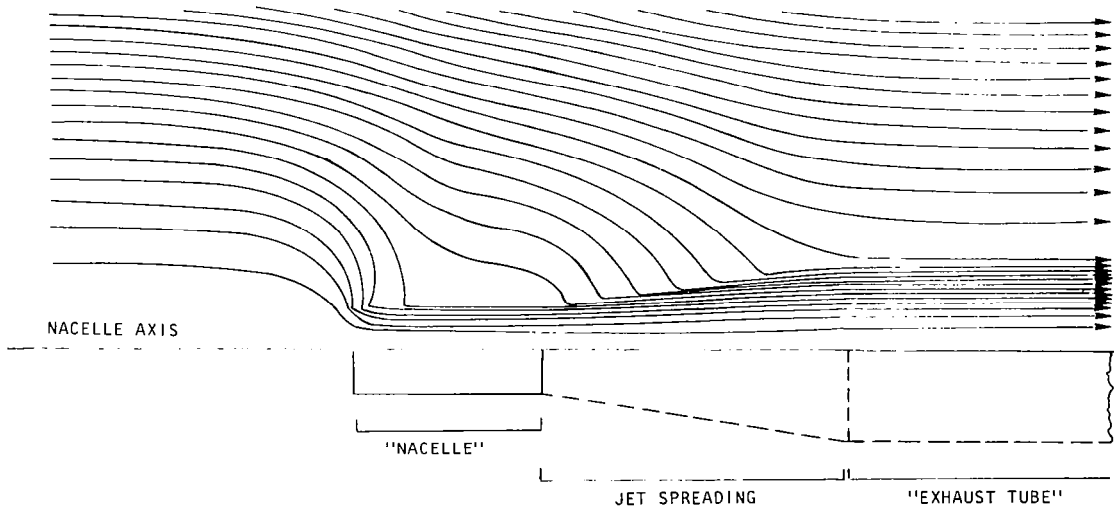
Figure 83. Representation of jet spreading and entrainment by vortex-ring polygons.
