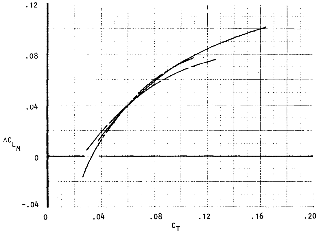
Figure 45. Variation of lift and moment increments due to blowing, noz N_4 , AR = 4.
