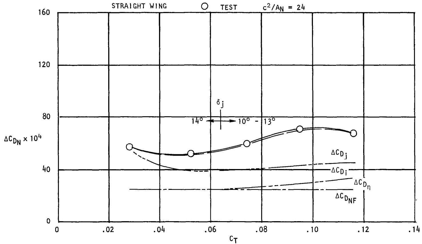
Figure 57. Incremental nacelle drag and component build-up, noz N_{3B} , AR = 2.5 , M_\infty = 0.68 , C_{LM} = 0.40 .
