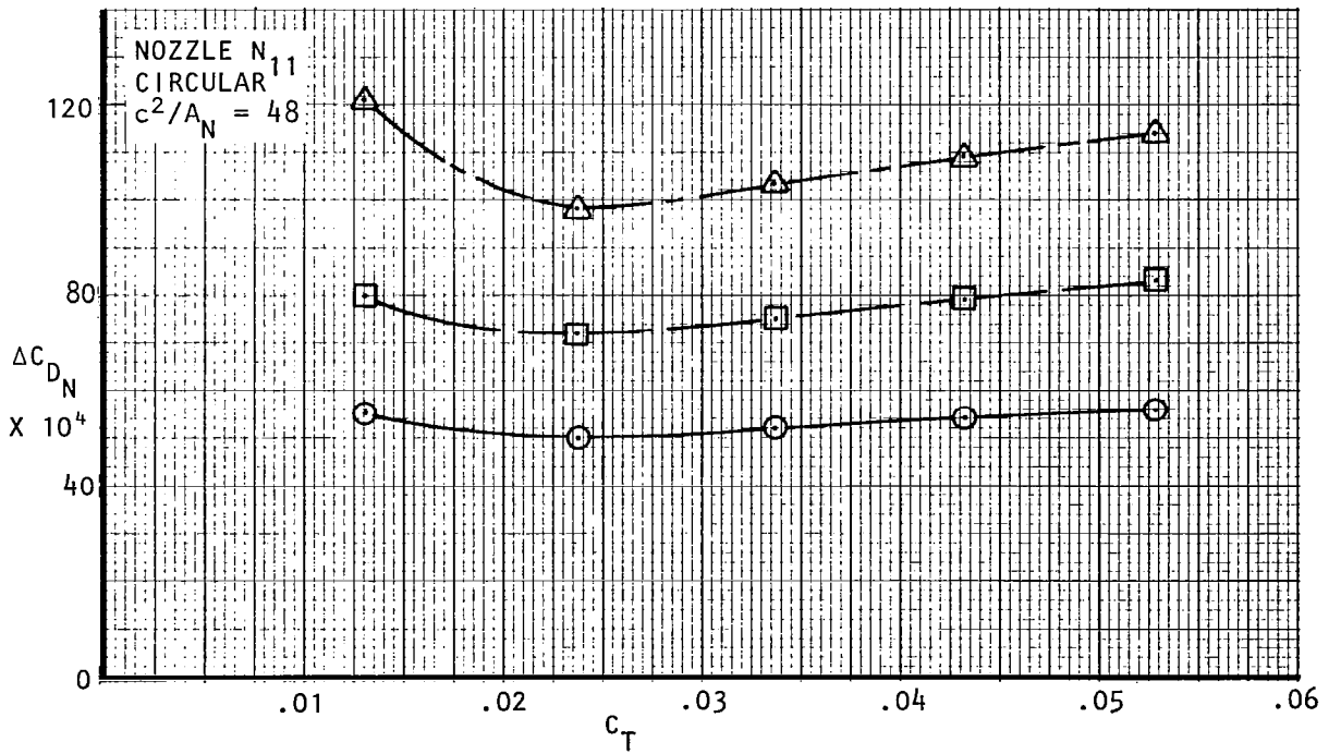
Figure 23. Effect of lift coefficient on nacelle drag, M_\infty = 0.73
