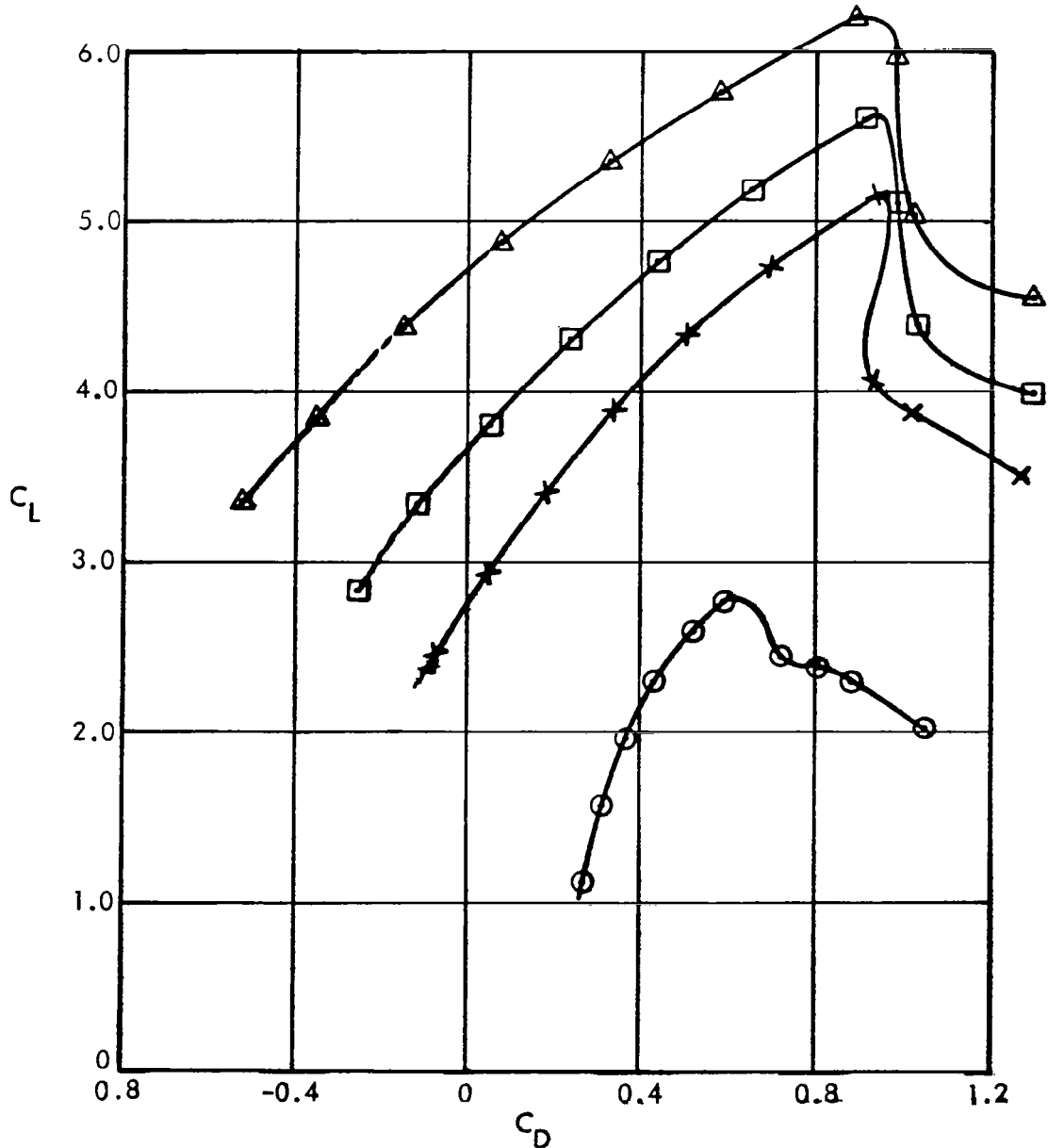
Figure 110. Variation of low speed model lift coefficient with drag coefficient, q_{\infty} = 718.2 \text{ N/m}^2 (15 lb/ft 2 ), \delta_f = 52^\circ , Coanda plate, tail-off
