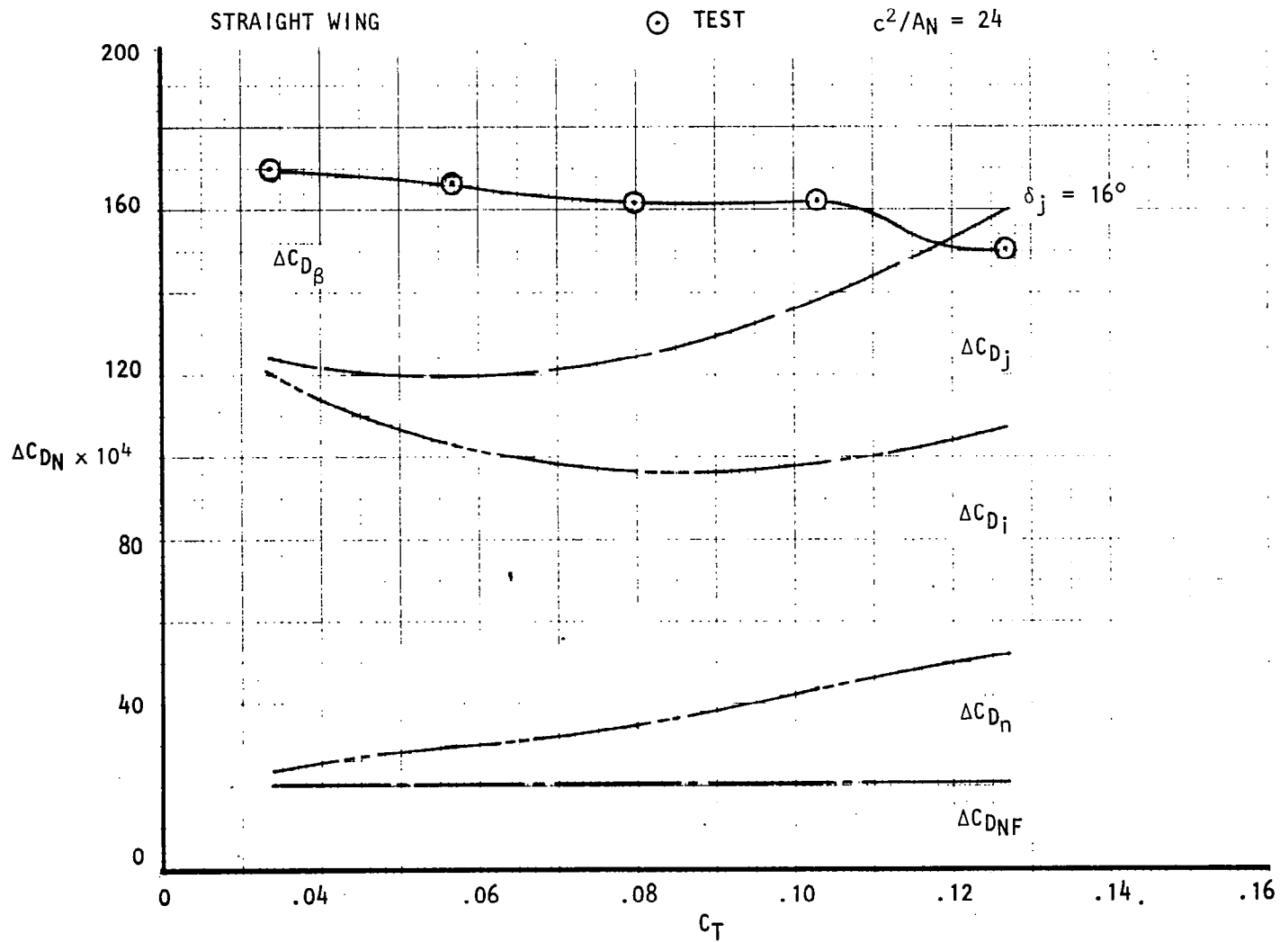
Figure 65. Incremental nacelle drag and component build-up noz N_{4E} , AR = 4 , M_\infty = 0.68 , C_{LM} = 0.40 .
