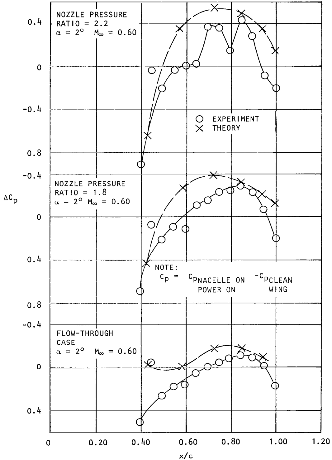
Figure 86. Predicted and measured surface pressure increments aft of nacelle (Row A).
