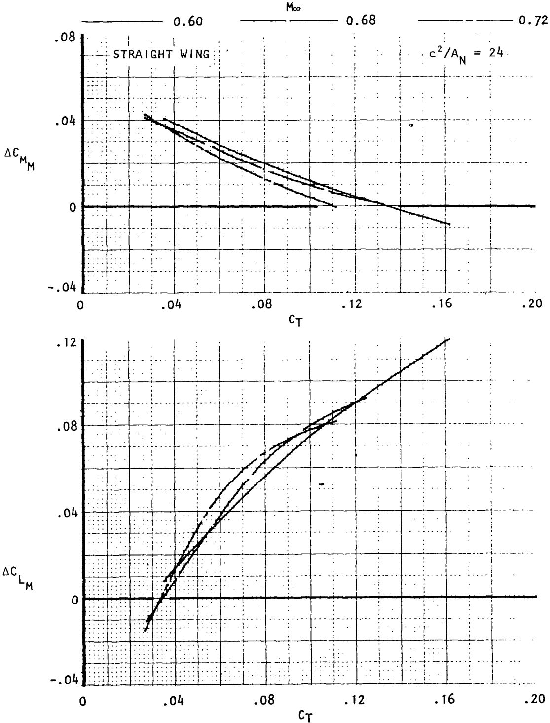
Figure 47. Variation of lift and moment increments due to blowing, noz N_5 , AR = 6.
