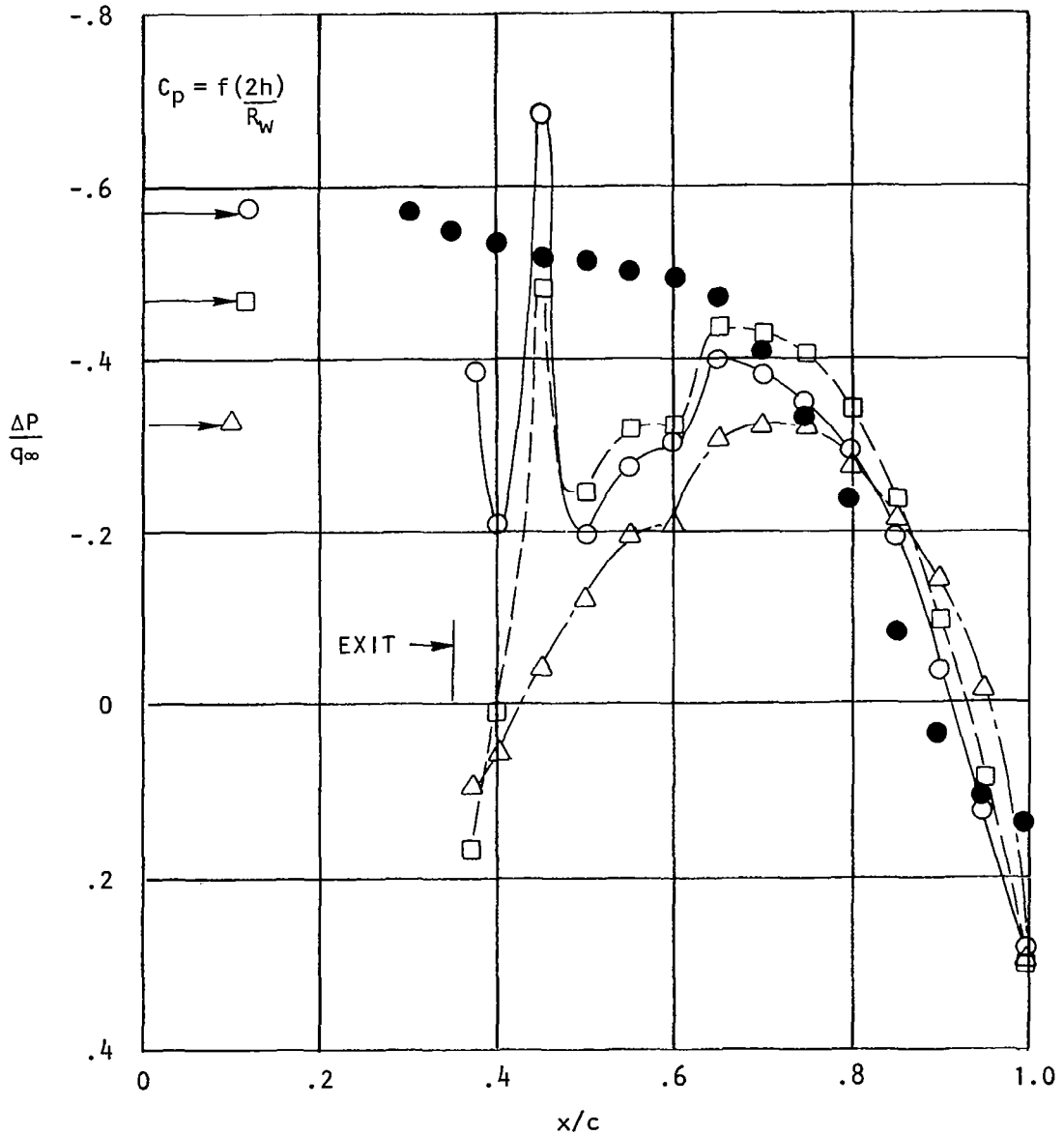
Figure 13 . Effect of nozzle exit shape on jet center-line pressures, \alpha \approx 2^\circ , M_\infty = 0.60 , H_j/p_\infty = 1.4 .
