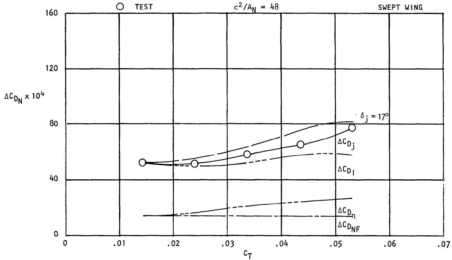
Figure 63. Incremental nacelle drag and component build-up, noz N 13 , AR = 6, M ∞ = 0.73, C LM = 0.40.
