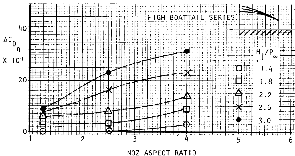
Figure 71. Effect of nozzle exit aspect ratio on scrubbing drag, M_\infty = 0.68
