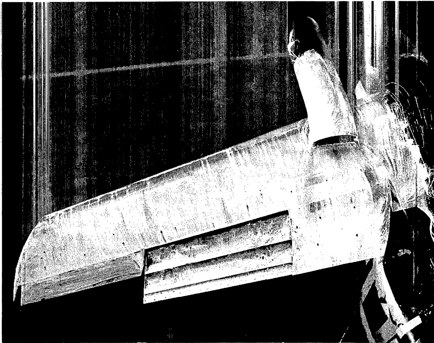
Figure 111. Oil flow photo of nacelle-wing flow pattern, \delta_f = 42.5^\circ , C_T = 0.82 , \alpha = 10^\circ .
