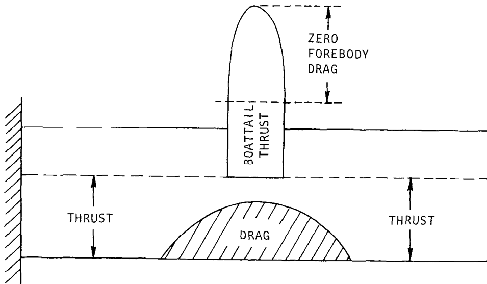
Figure 90. Location of drag-producing and thrust-producing regions due to application of power.
