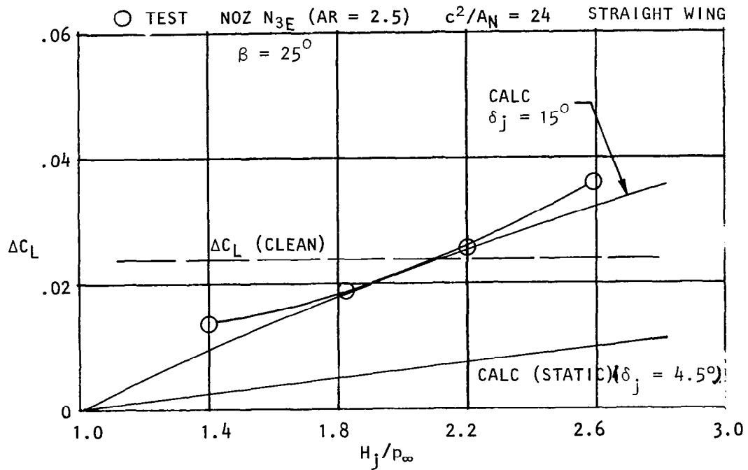
Figure 18. Lift developed in scrubbed area with blowing, \alpha = 2^\circ , M_\infty = 0.70 .
