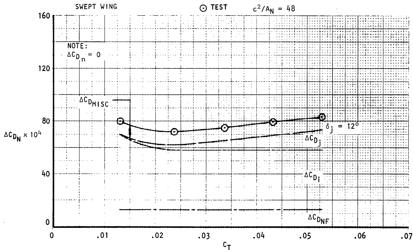
Figure 60. Incremental nacelle drag and component build-up, noz N_{11} , circular, M_\infty = 0.73 , C_{LM} = 0.40 .
