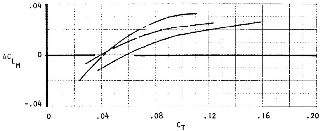
Figure 41. Variation of lift and moment increments due to blowing, nozzle N_2 , circular.
