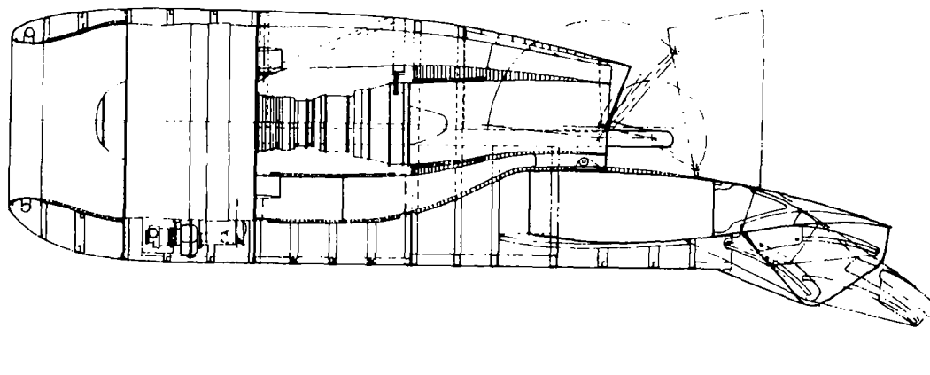
Figure 96. Nacelle inboard profile.
