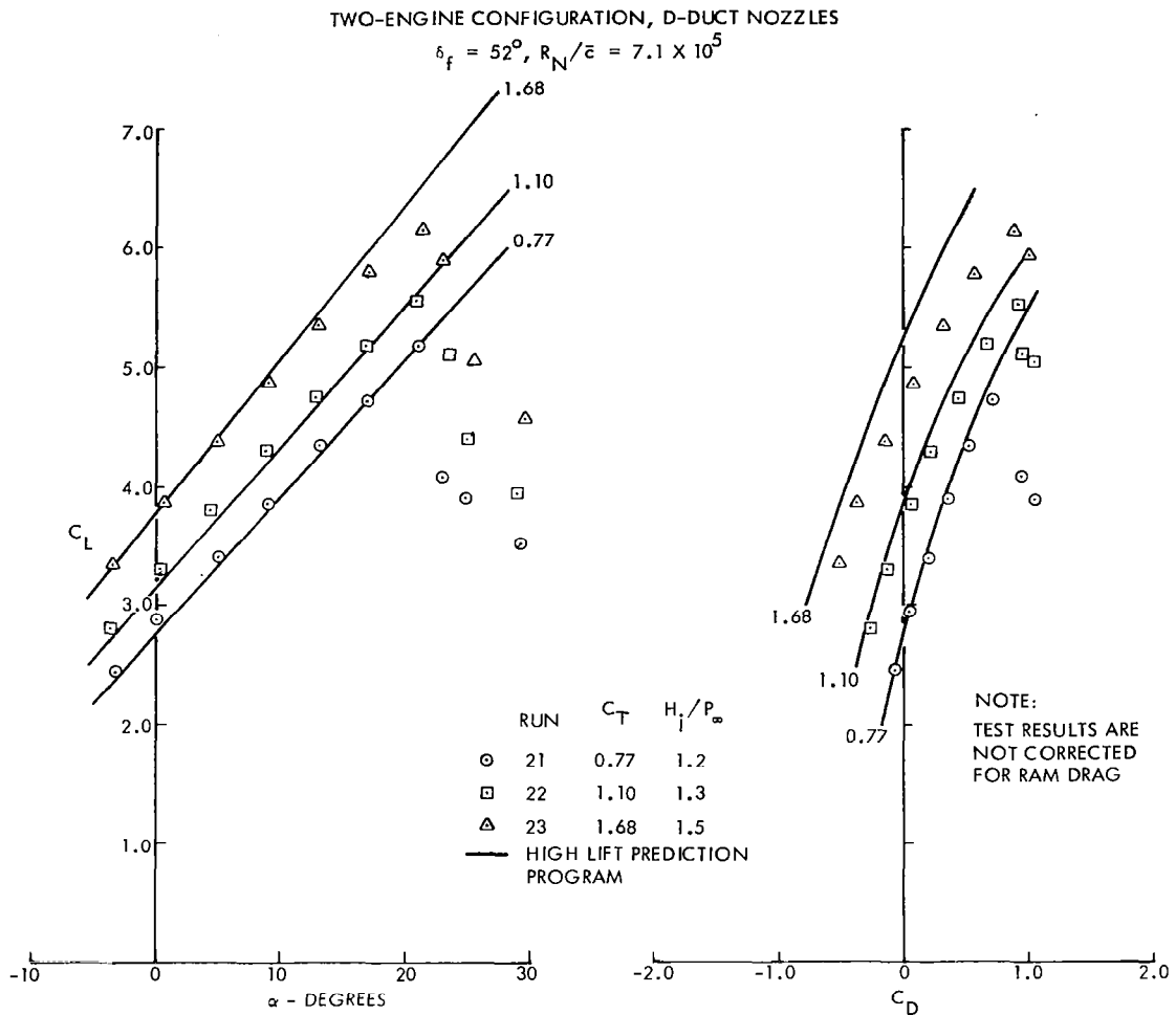
Figure 117. Correlation of theoretical and experimental high-lift performance, USB low speed model, tail off
