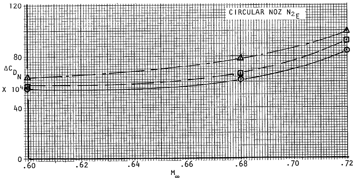
Figure 36. Effect of Mach number on nacelle drag coefficient, C_{LM} = 0.40
