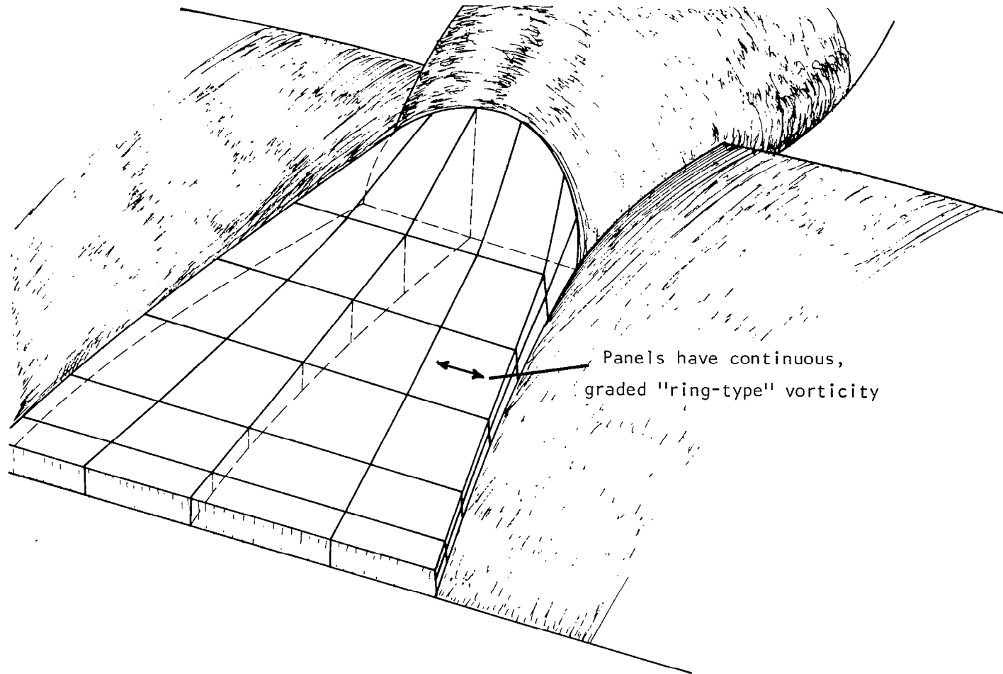
Figure 84. Mathematical model of the USB jet efflux.
