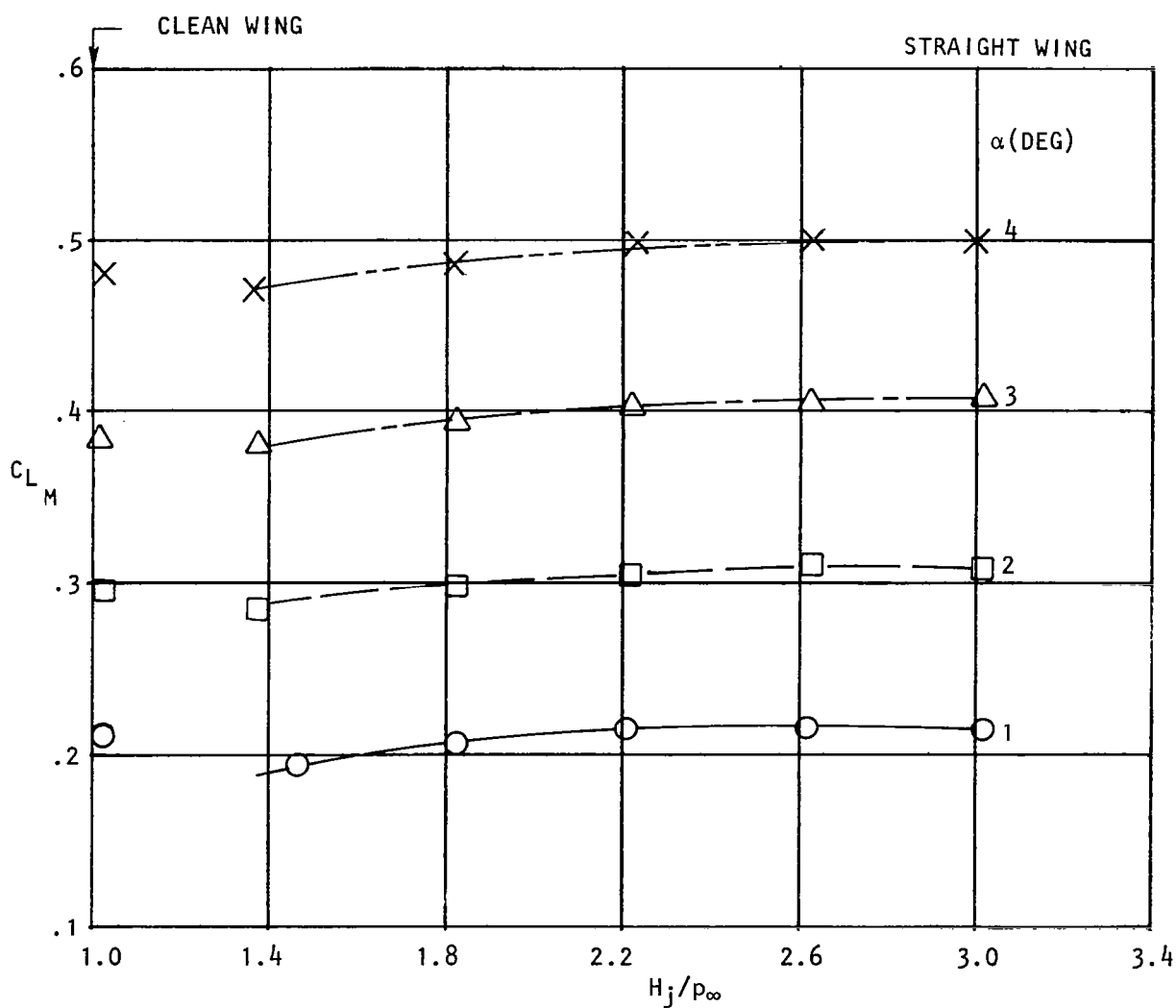
Figure 26. Effect of nozzle pressure ratio on total lift, noz N_2 , circular, M_\infty = 0.68 .
