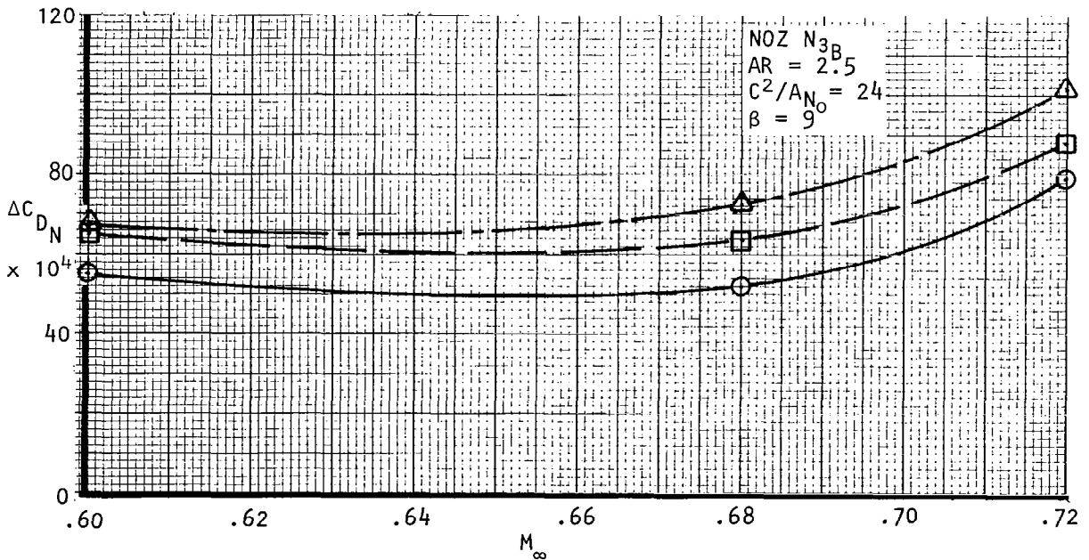
Figure 37. Effect of Mach number on nacelle drag coefficient, C_{LM} = 0.40
