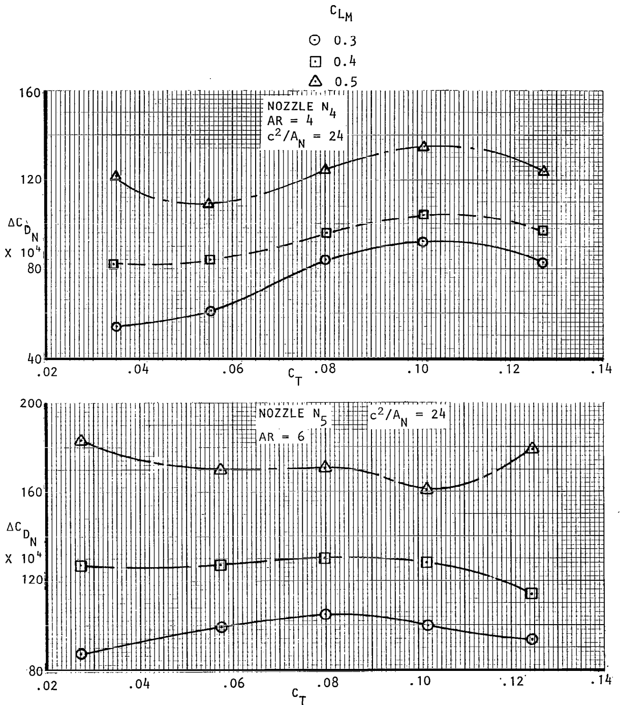
Figure 22 . Effect of lift coefficient on nacelle drag, M_\infty = 0.68
