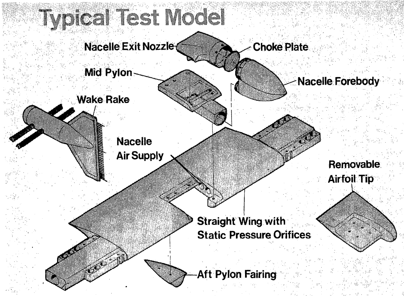
Figure 2. Exploded view of basic test model arrangement.
