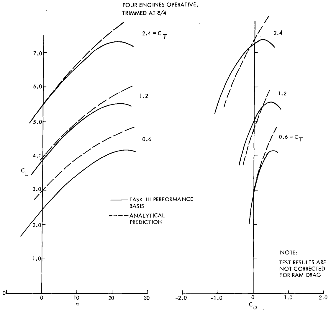
Figure 118. Comparison of Task III USB configuration performance with math model prediction, \eta_t = 0.90 , \delta_f = 45^\circ
