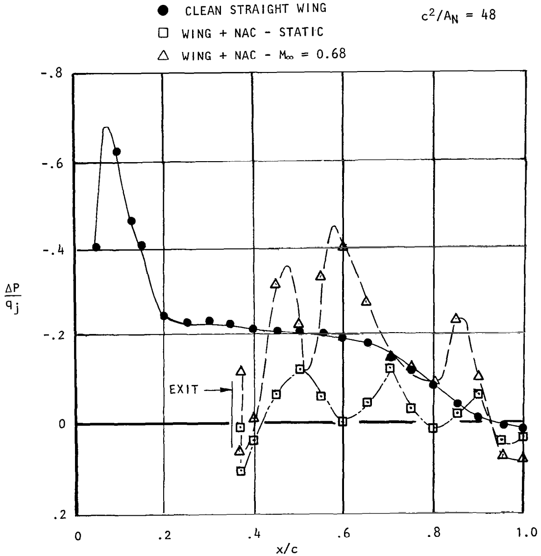
Figure 10. Jet centerline pressure distributions, "D-Duct", noz N_6 , H_j/p_\infty = 2.6 , \alpha = 2.6^\circ .
