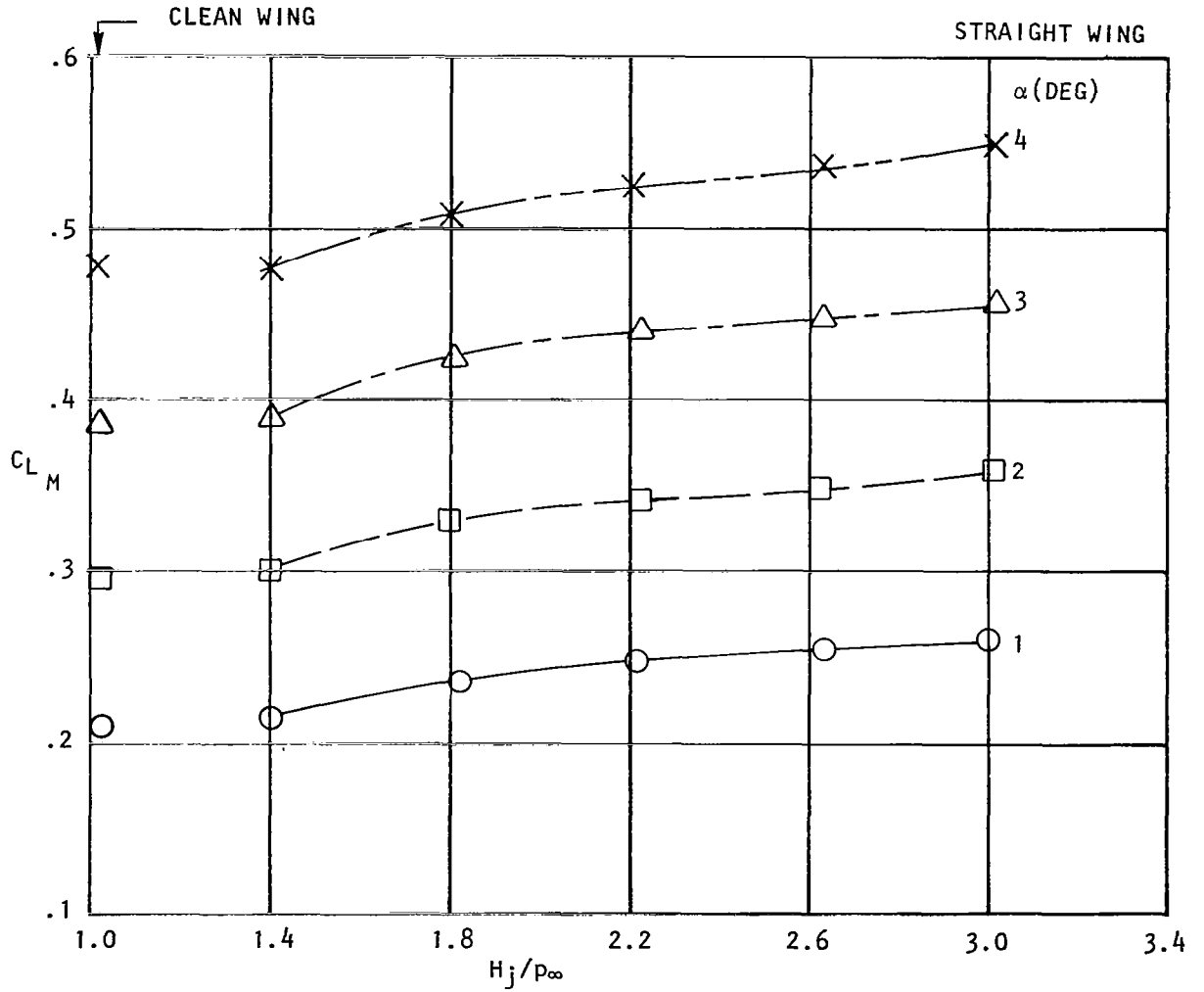
Figure 25. Effect of nozzle pressure ratio on total lift, noz N_{3E} , AR = 2.5 , M_\infty = 0.68 .
