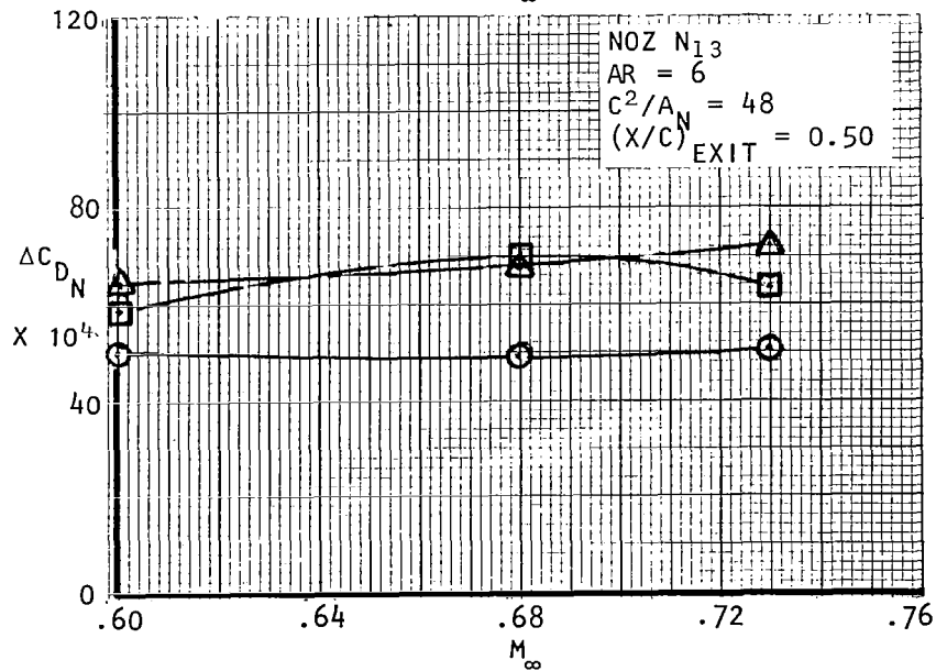
Figure 40. Effect of Mach number on nacelle drag coefficient, C_{L_M} = 0.40
