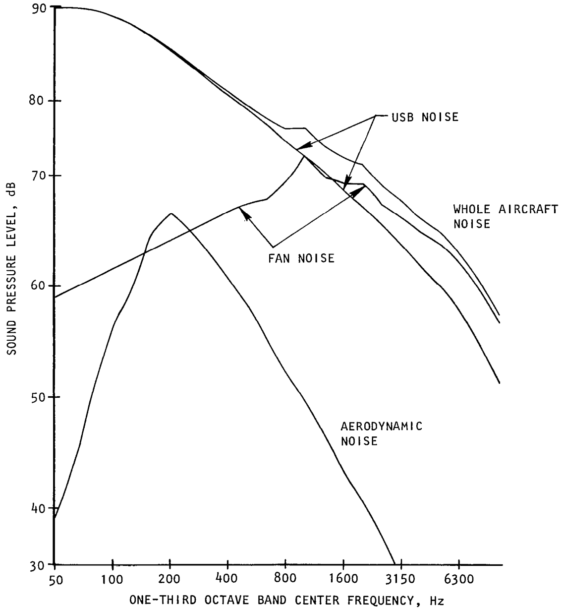
Figure 98. Spectra by source, final design aircraft, takeoff elevation angle = 90°, 152.4 M (500 ft) distance, no ground reflection
