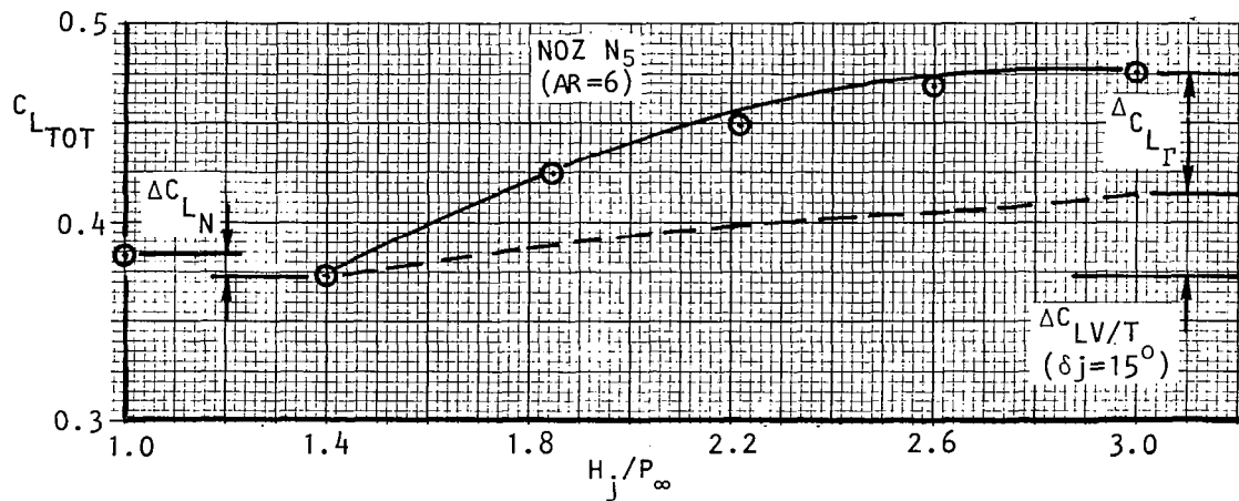
Figure 67, Components of total lift coefficient, M_\infty = 0.68 , \alpha = 3^\circ
