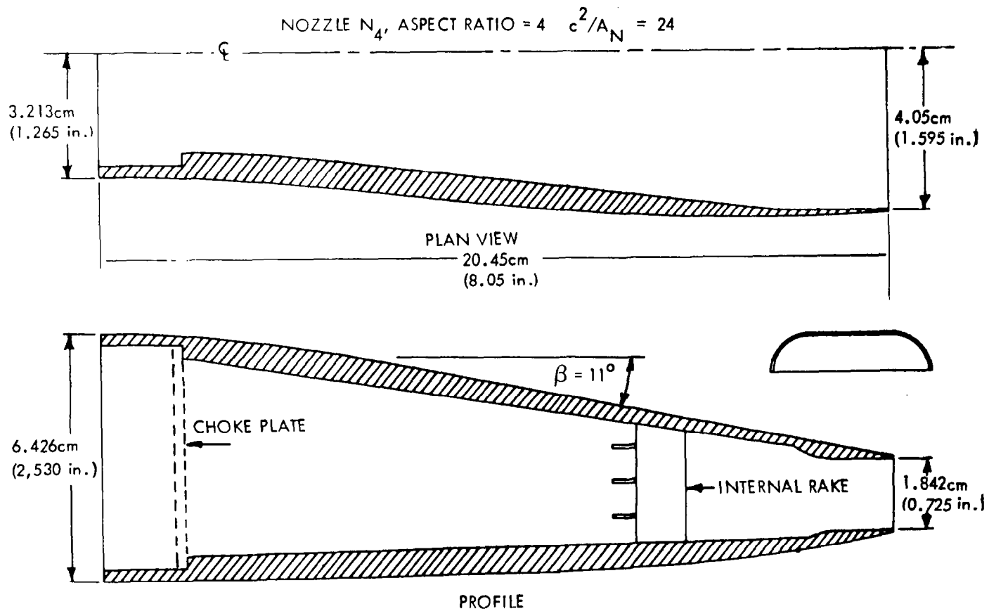
Figure 5. Typical nozzle design
