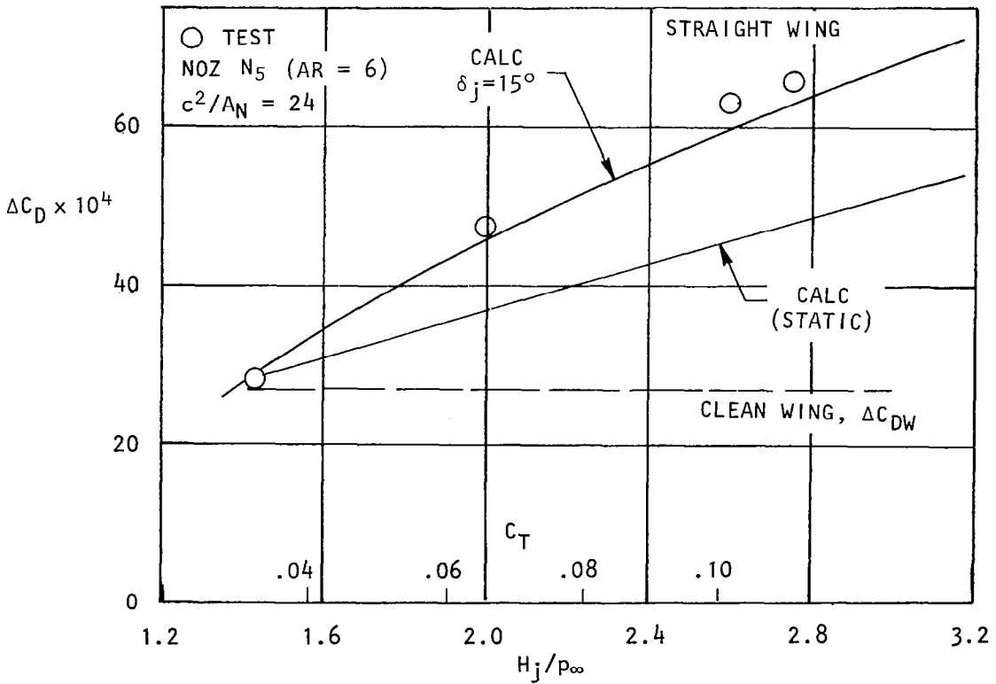
Figure 15. Variation of scrubbed area pressure drag with pressure ratio, \alpha = 2^\circ , M_\infty = 0.68 .
