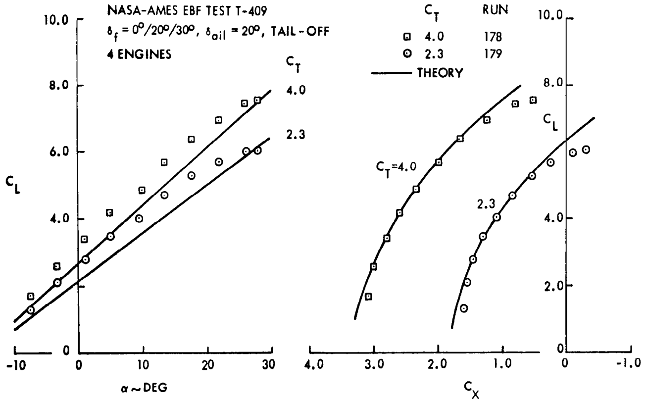
Figure 115. Correlation of theoretical and experimental longitudinal aerodynamic characteristics for a NASA Ames tested high-wing EBF STOL configuration
