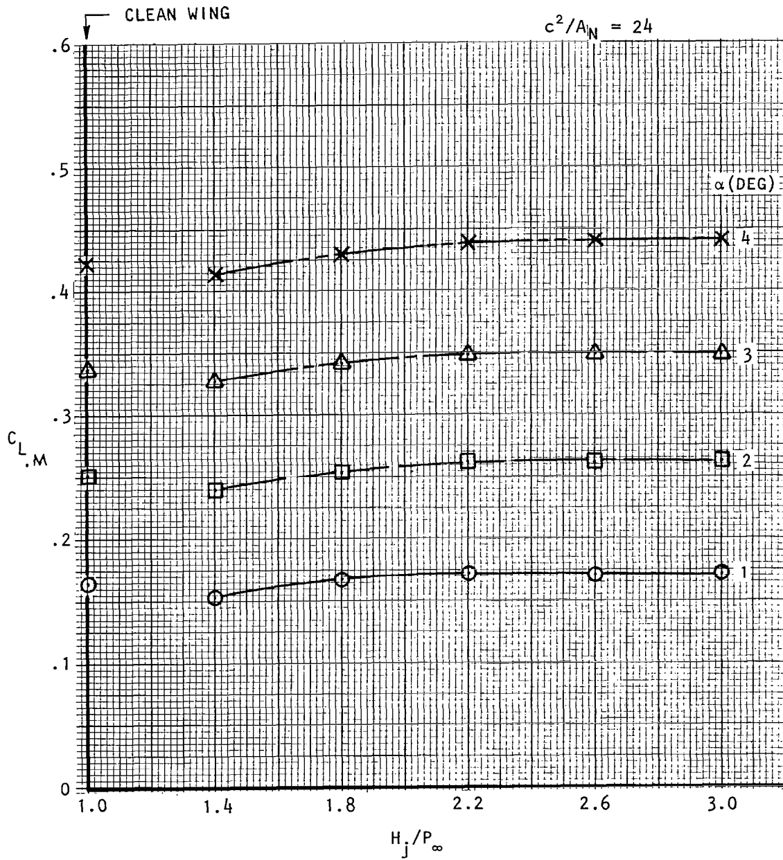
Figure 29 . Effect of nozzle pressure ratio on total lift, noz N_{11} , AR = circular, M_\infty = 0.73
