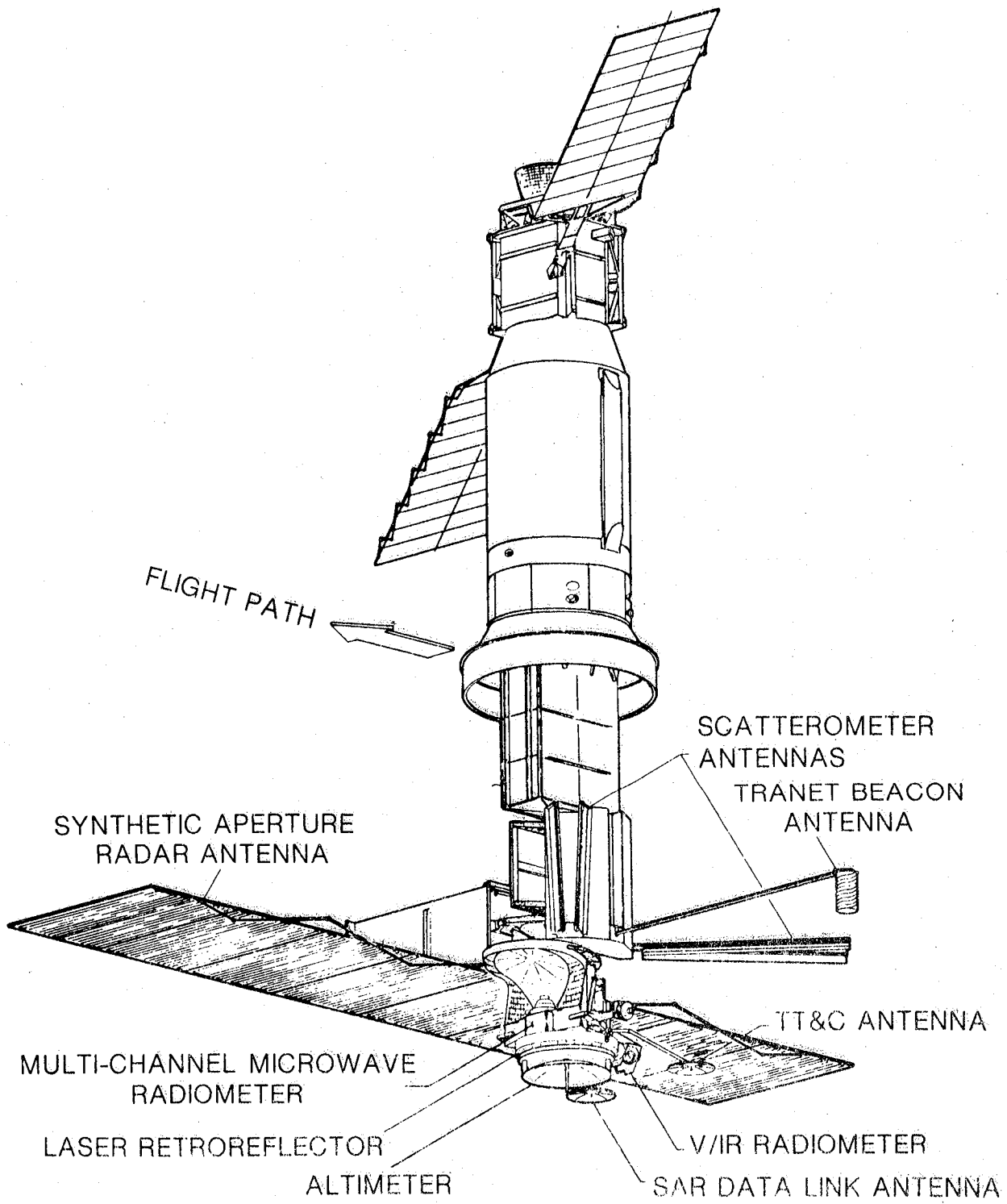
Figure 14. SEASAT-A
