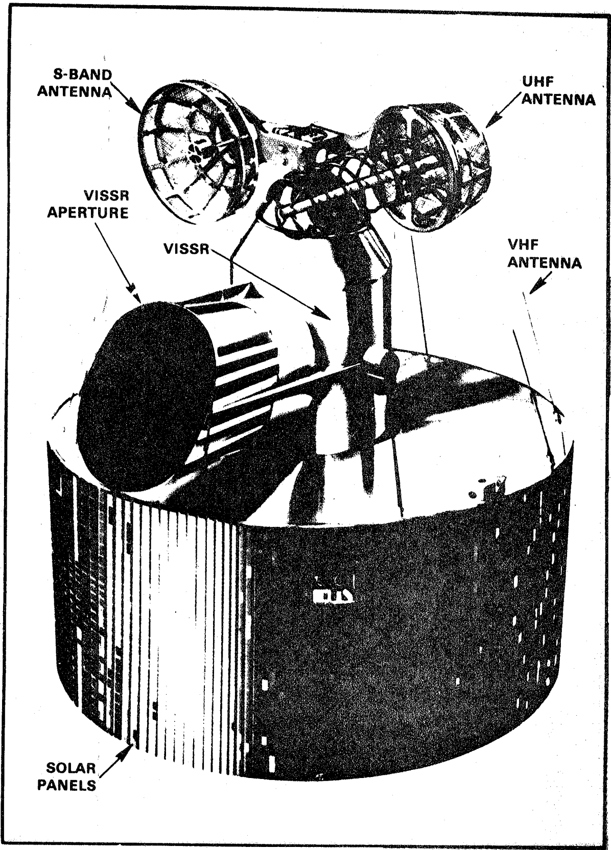
Figure 12. Geostationary Meteorological Satellite (GMS) (Himawari)
