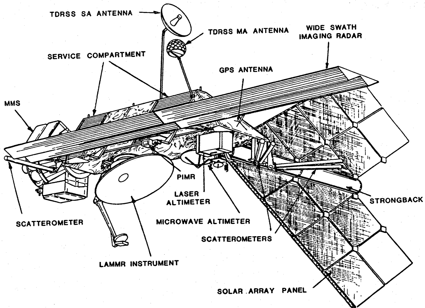
Figure 17. ICESat Spacecraft
