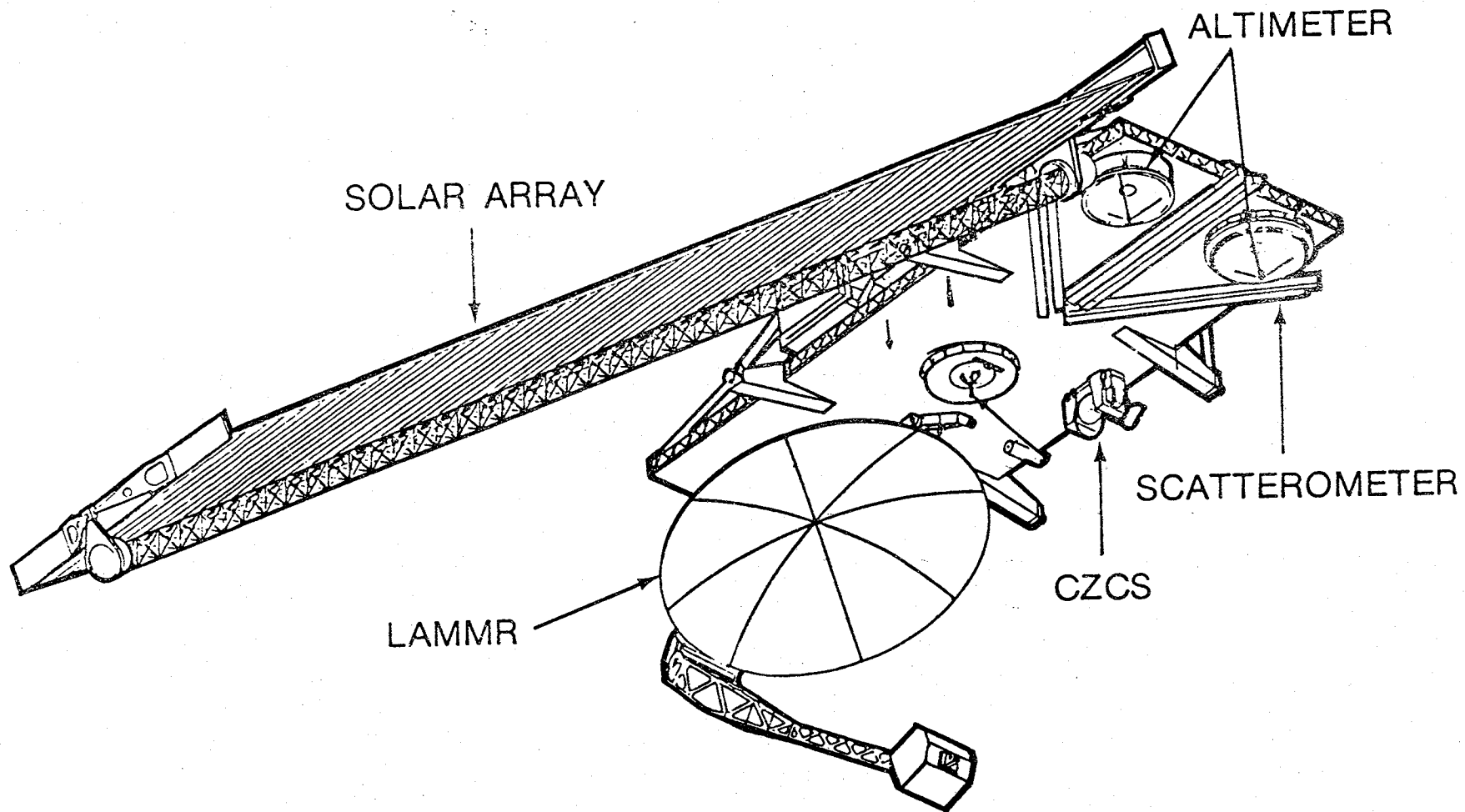
Figure 15. NOSS Spacecraft
