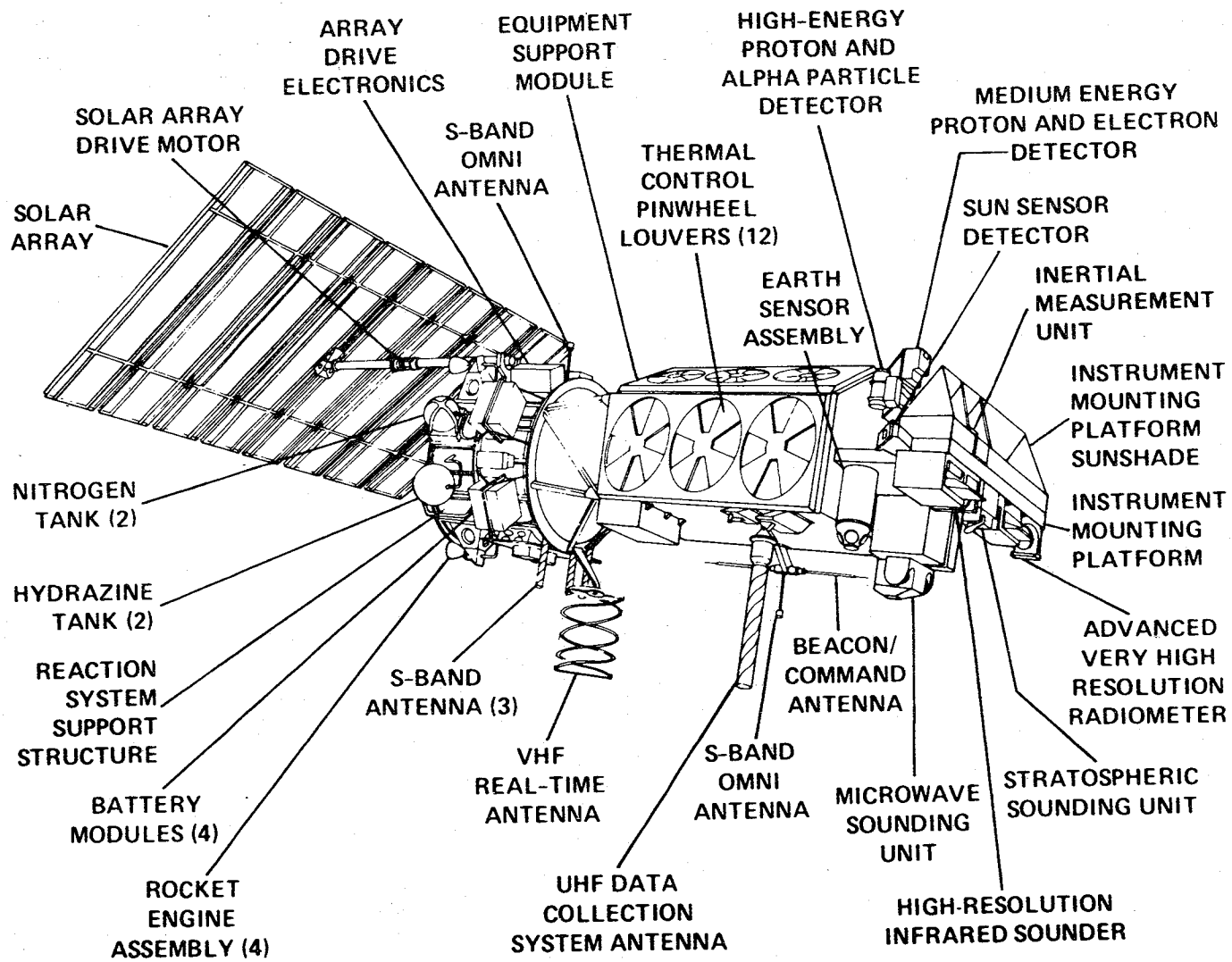
Figure 6. TIROS-N Spacecraft
