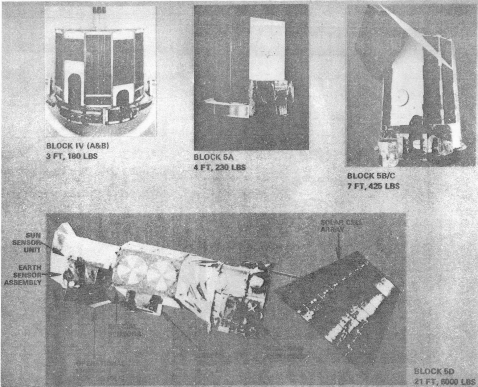
Figure 10(a). Evolution of the DMSP Space Segment
