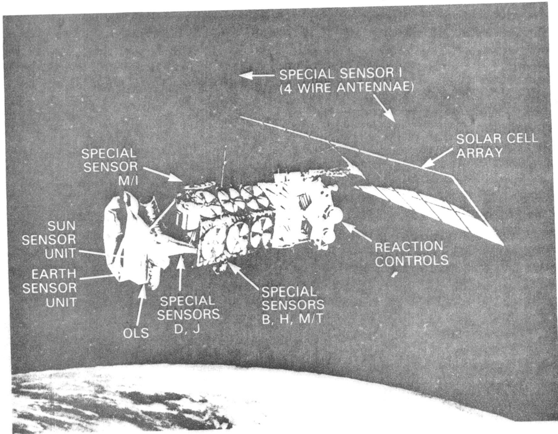
Figure 10(b). DMSP 5D-2 In Orbit
