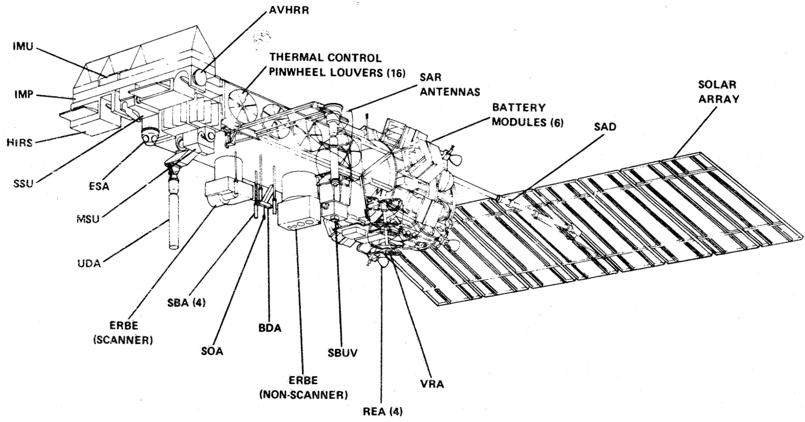
Figure 7. Advanced TIROS-N Spacecraft
