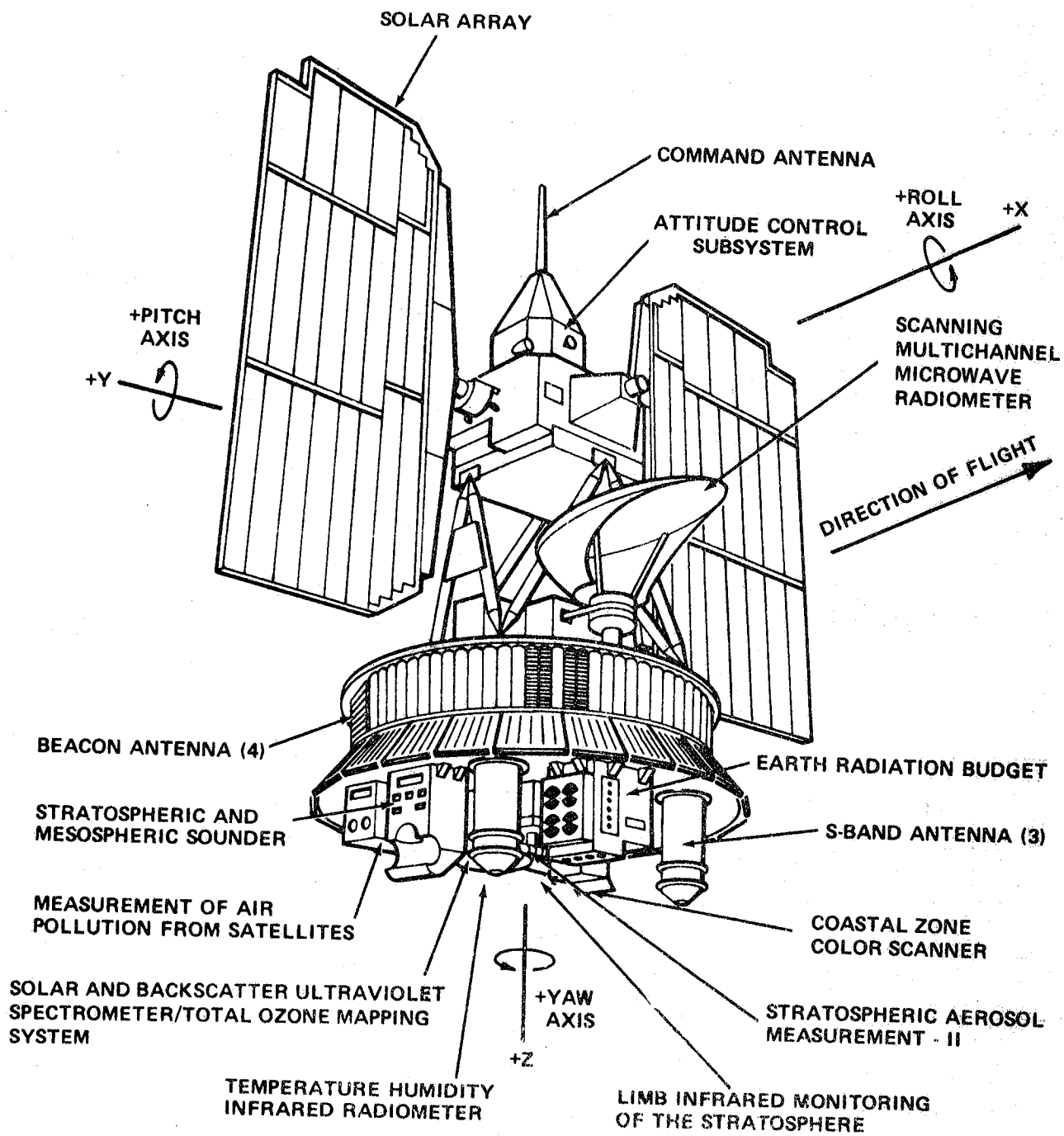
Figure 3. NIMBUS-7 Spacecraft
