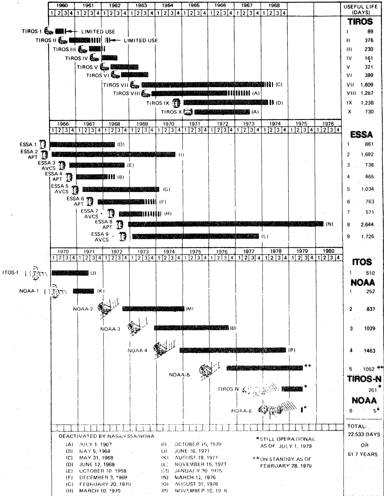
Figure 1. TIROS/ESSA/ITOS/NOAA Program Summary
