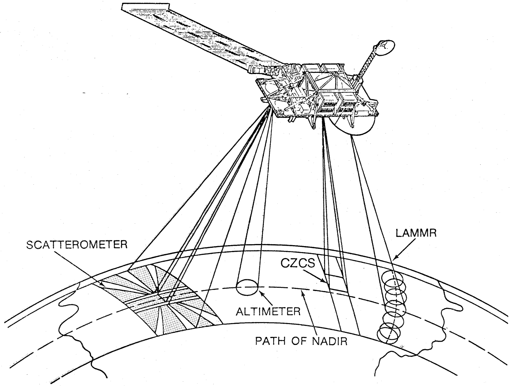
Figure 16. NOSS Sensor Coverage
