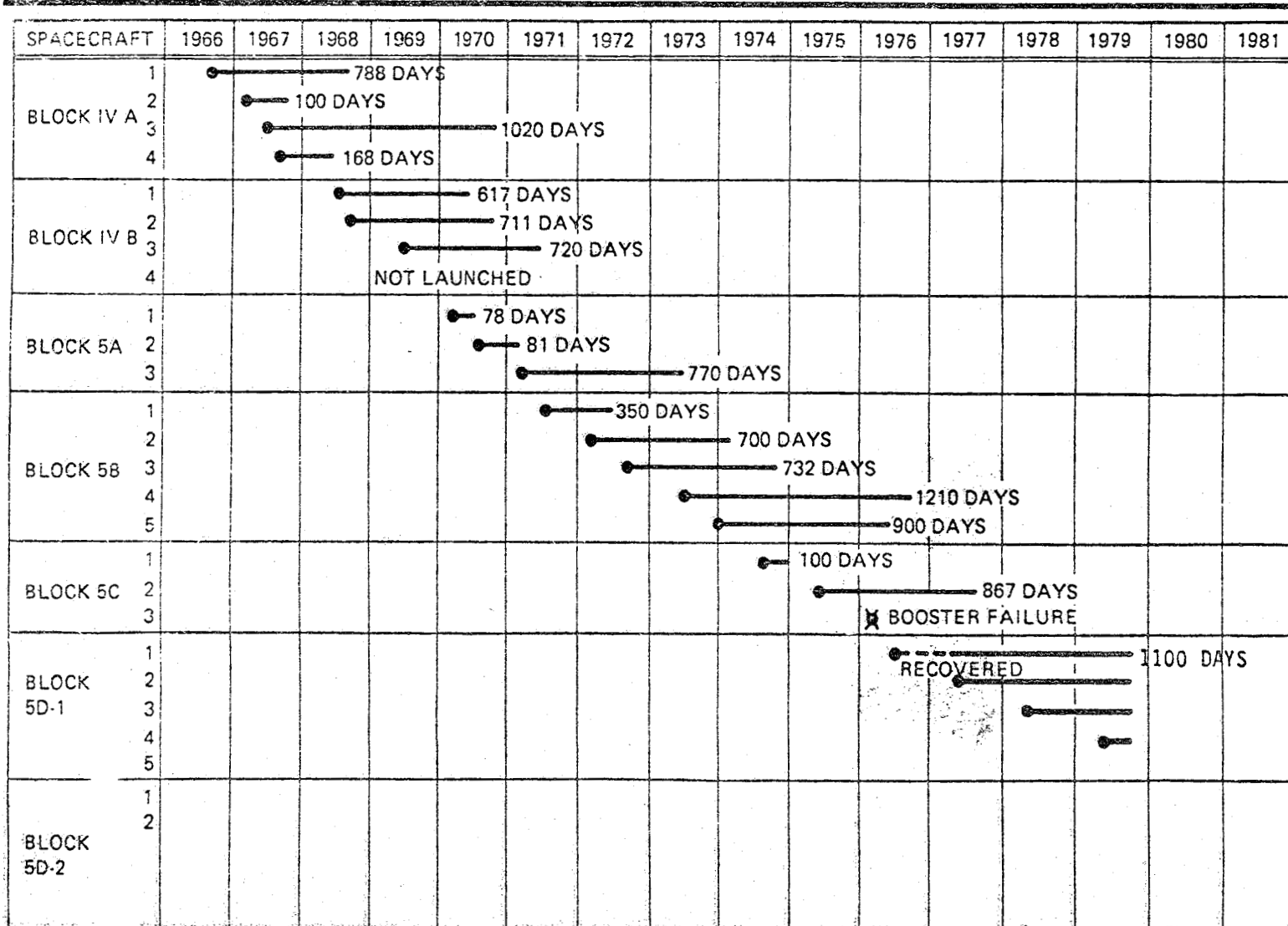
Figure 9. DMSP On-Orbit Performance
