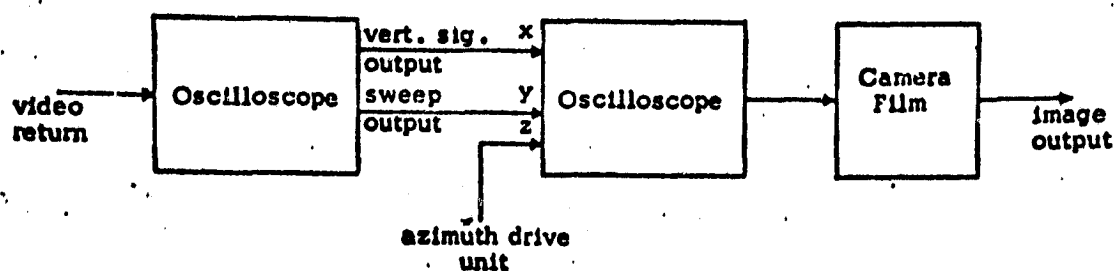
Figure 6. Component arrangement for imagery operation (ref. 1).
