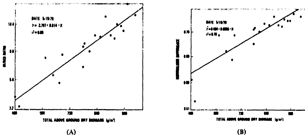
Figure 3. The IR/red radiance ratio and normalized difference plotted against total above-ground dry matter accumulation on May 19, 1978 (Julian date 139). The total dry matter accumulations were sampled at the end of the growing season.
