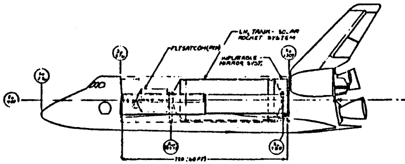
SIDE VIEW
