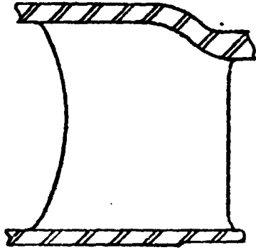
Meridional View
