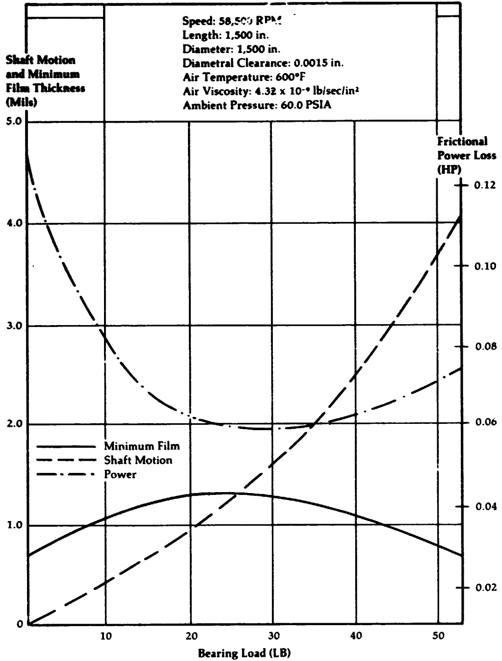
Bearing Load vs Shaft Motion, Minimum Film Thickness, And Frictional Power Loss (No End Leakage Correction Factors Applied)
