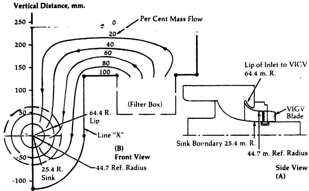
Calculated Streamline Pattern for Original Upgraded Engine Intake Design
