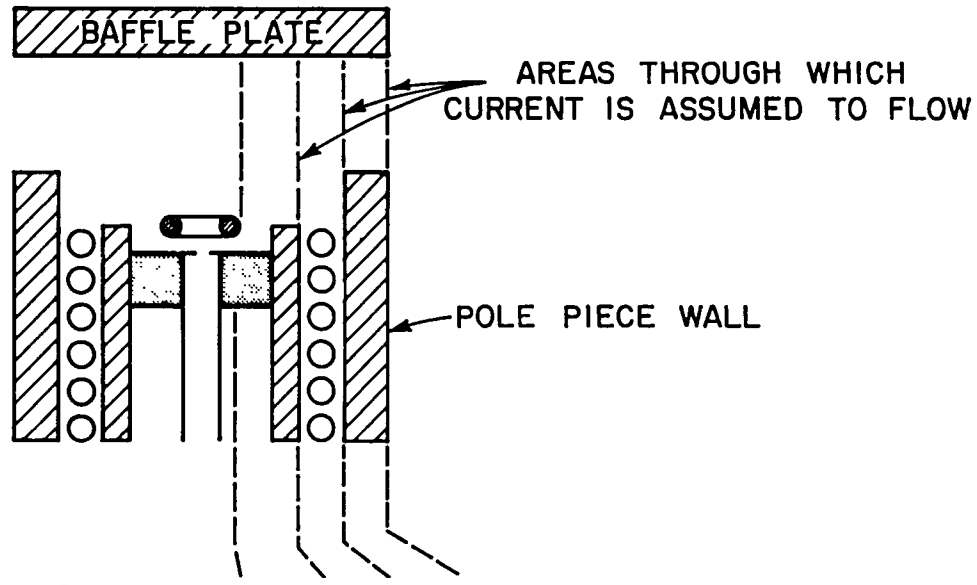
Fig. E-1a Radial Field Cathode Pole Piece Baffle Aperture Region Showing Area Through which the Electron Current is Assumed to Flow
