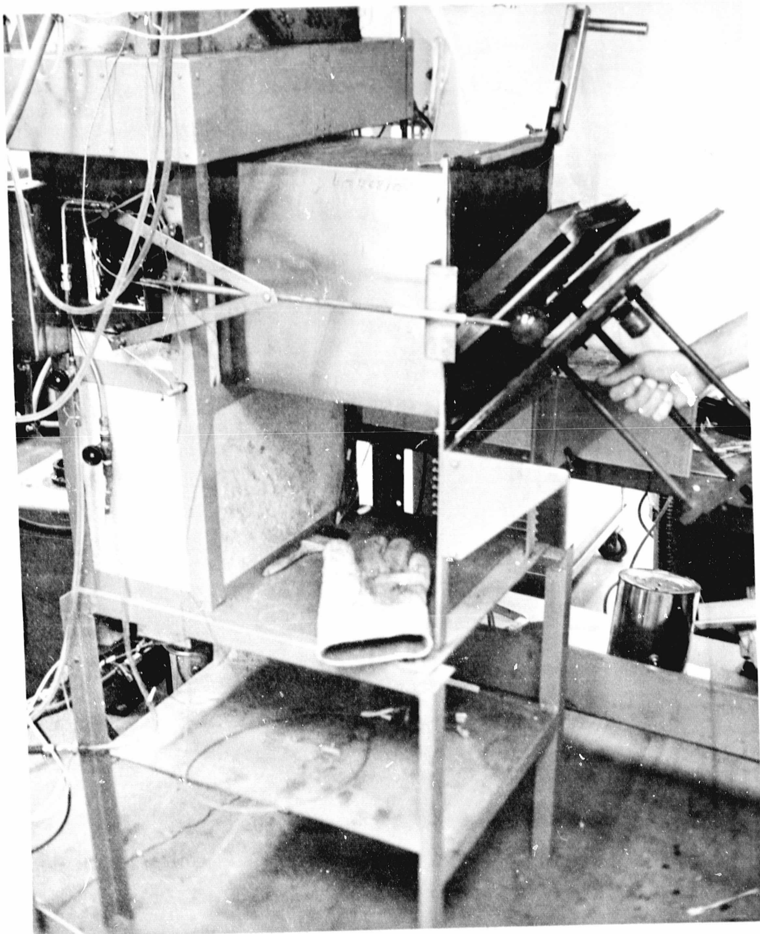
Figure 2 Laminate Being Inserted Into the OSU Apparatus
