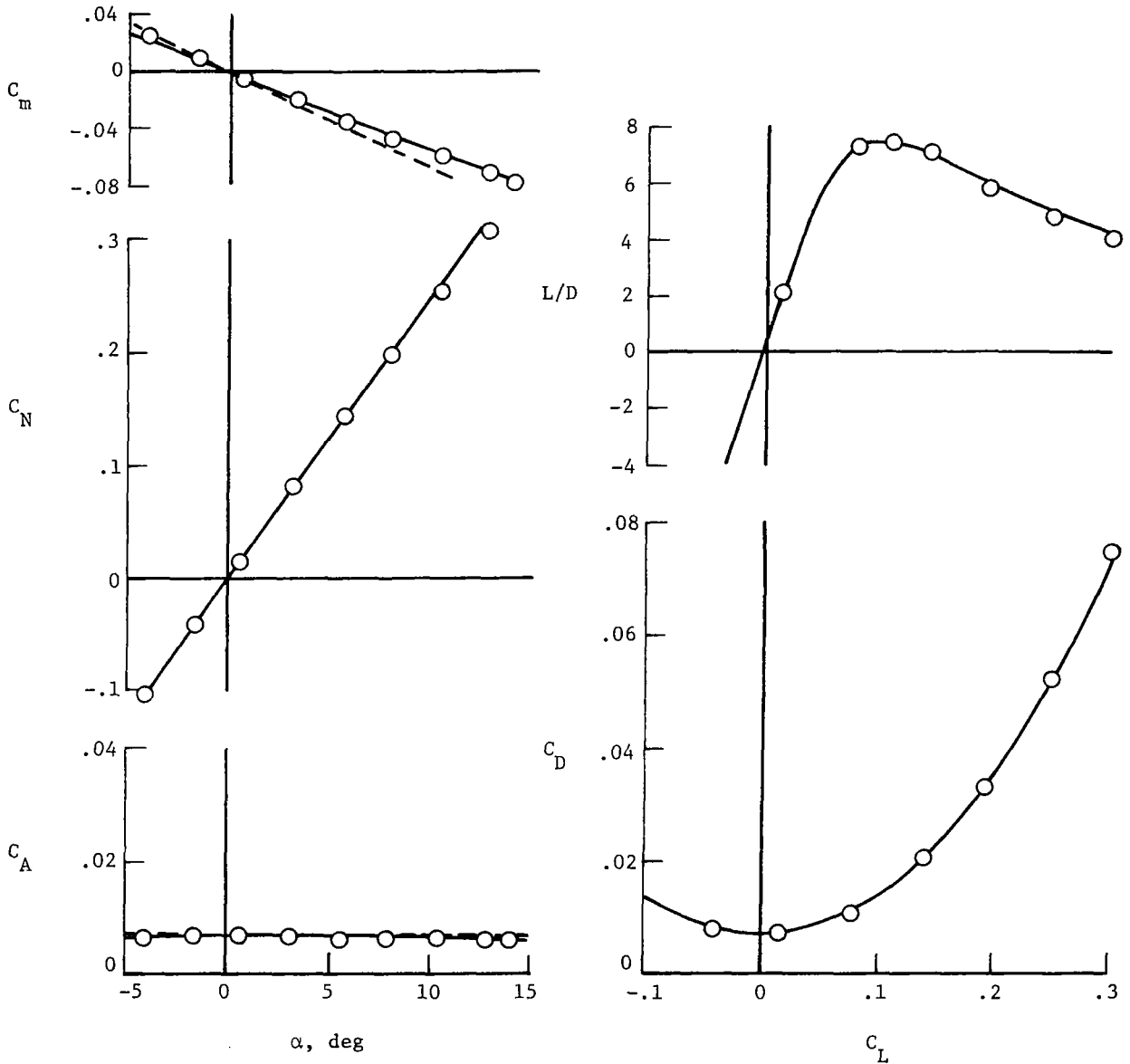
(a) C_{L,D} = 0 .
