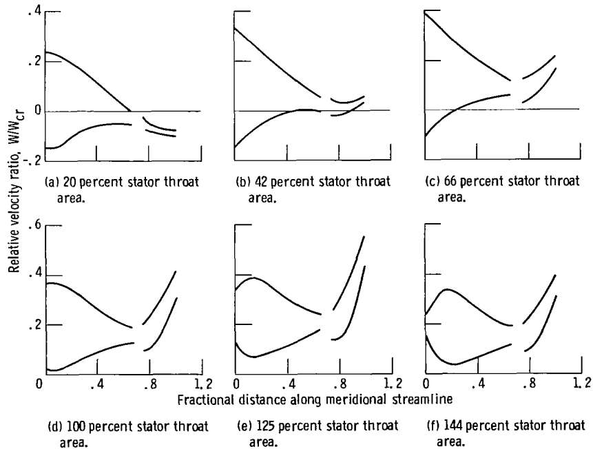
Figure 5. - Blade surface velocities at equivalent design speed and pressure ratio - design-rotor hub section. (From ref. 3.)
