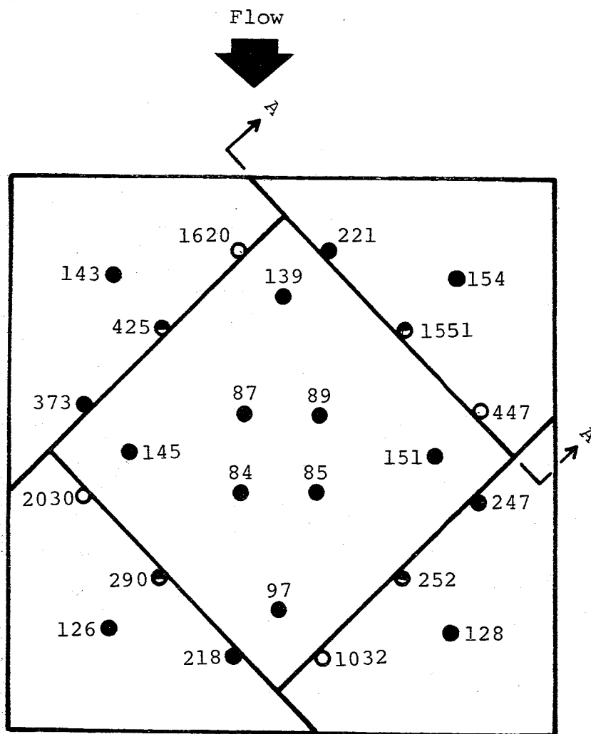
(e) Panel no. 5, ESA-3560 400s reentry at 20 Btu/ft 2 s
