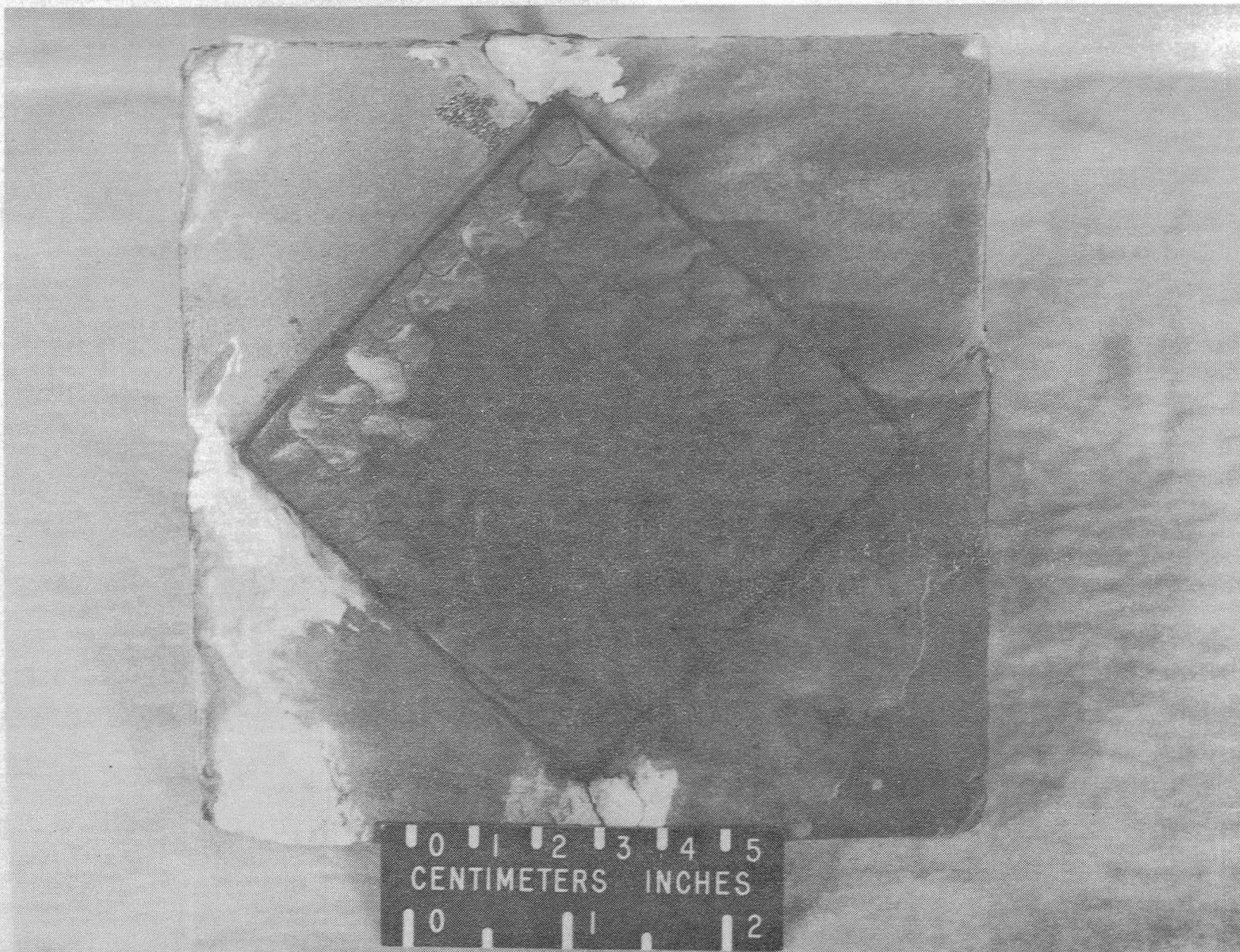
Figure 9.- Panel no. 5, ESA-3560 after 400s entry test at 20 Btu/ft 2 s.
