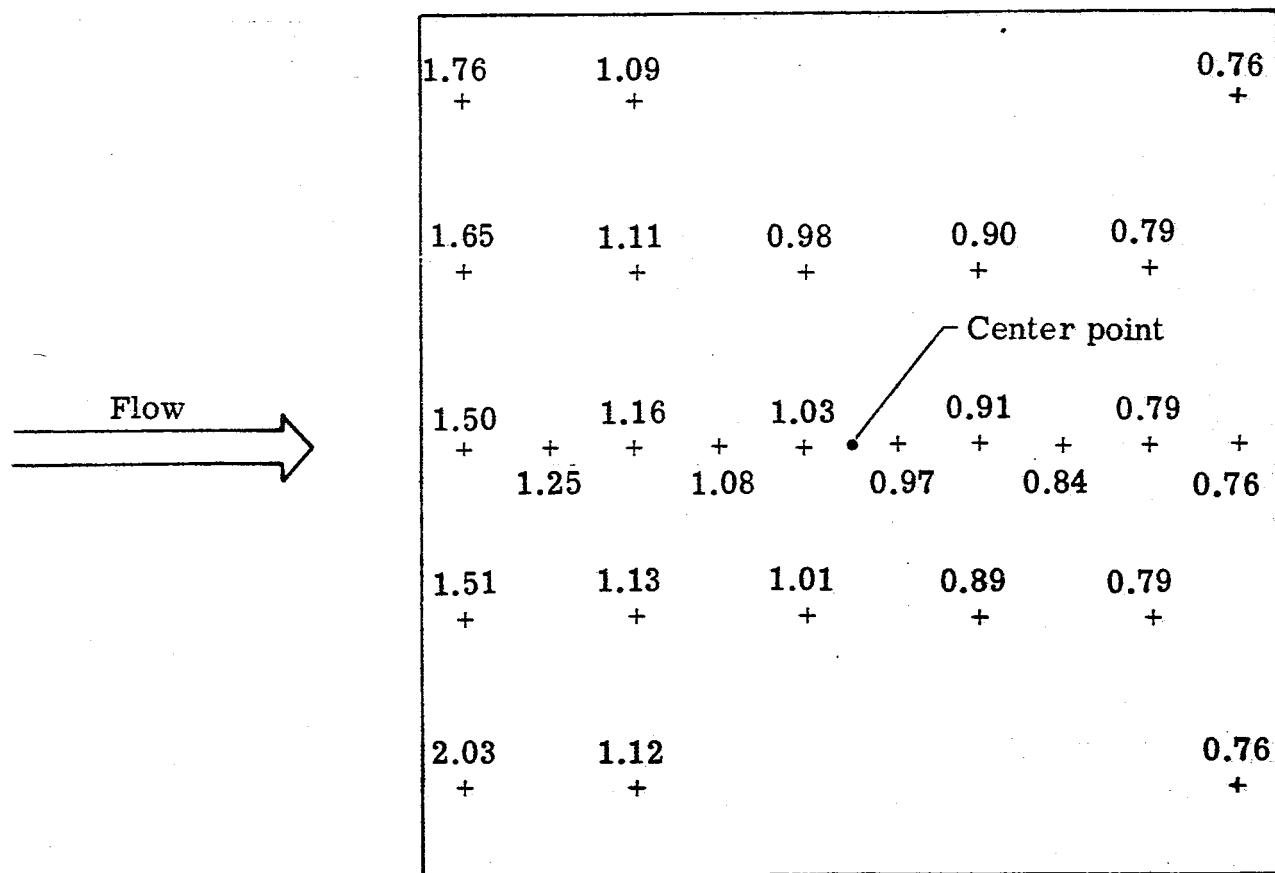
Figure 4.- Typical heating rate distribution normalized to center point.
