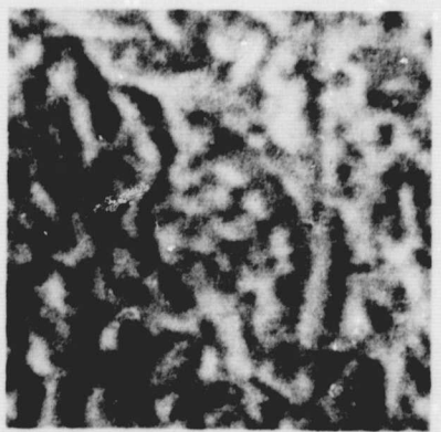
c) 1-91-1 9000X T_D = 630^\circ\text{C}
