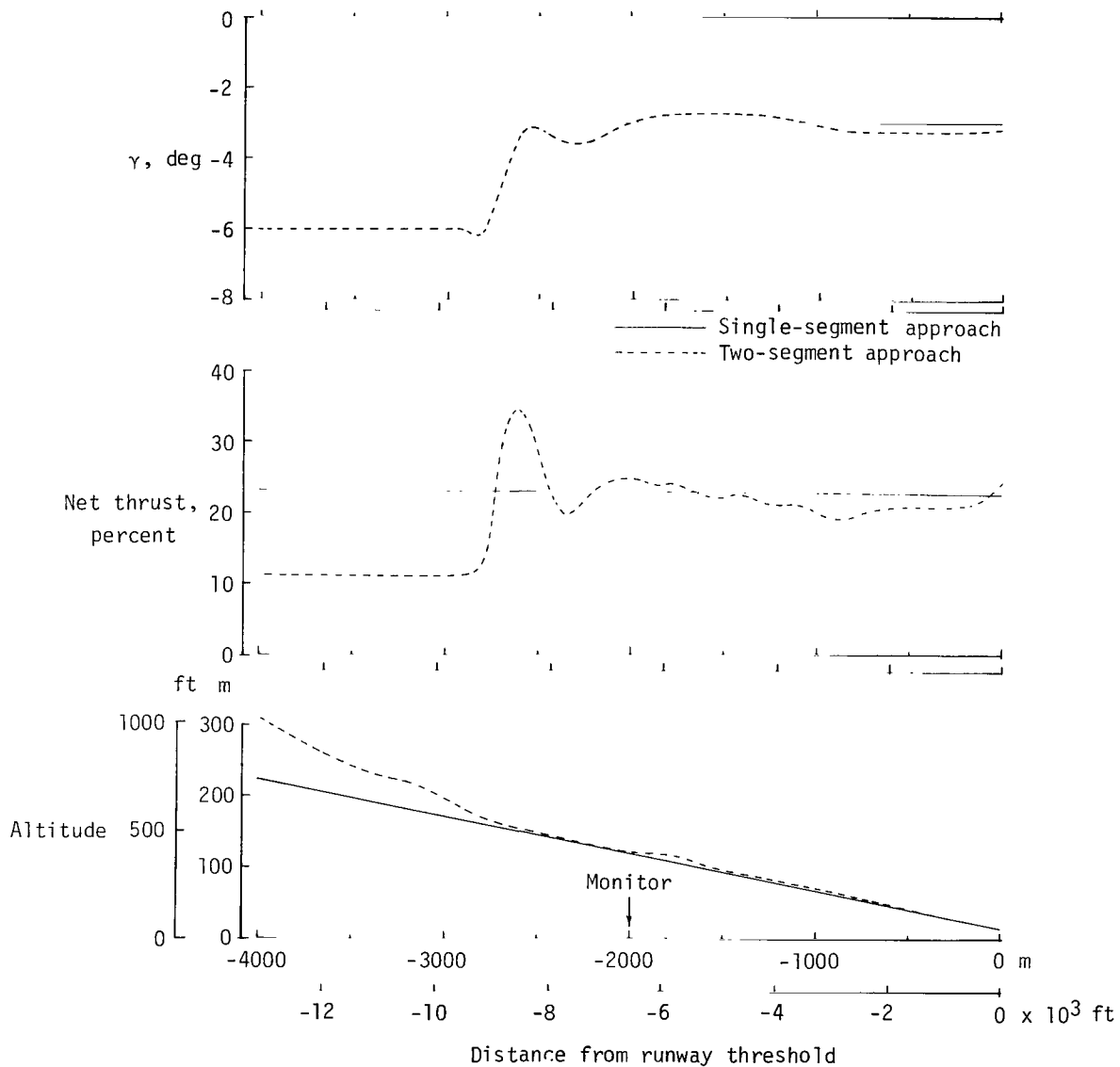
Figure 26.- Comparison of approach profiles for 6°/3° and constant 3° approaches. (V = 158 knots of IAS).
