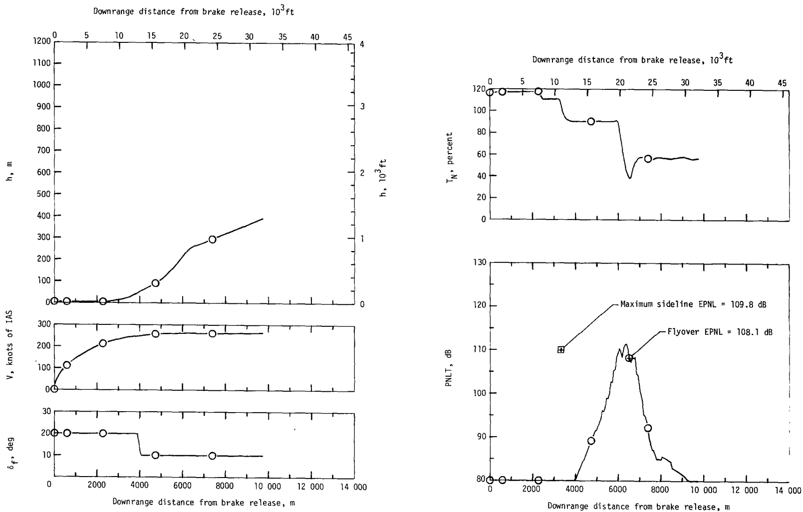
Figure 19.- Advanced-procedure-I takeoff profile and corresponding calculated sideline and flyover noise. (Noise levels indicated for jet noise only; symbols with +'s indicate values at measuring stations.)
