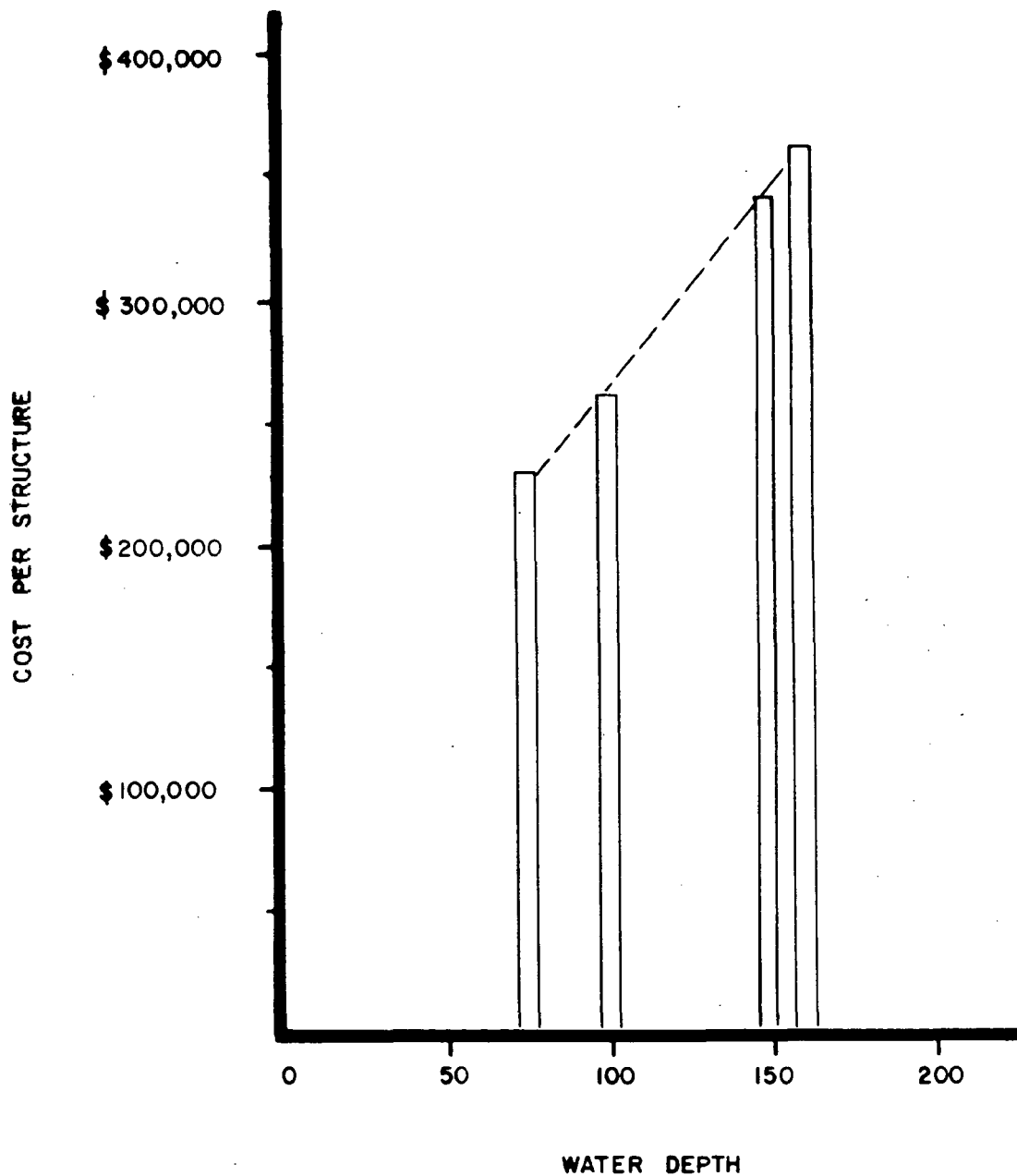
FIGURE 4.2-1 COST VS WATER DEPTH FOR PILED GUYED TOWER WITH PANELS
