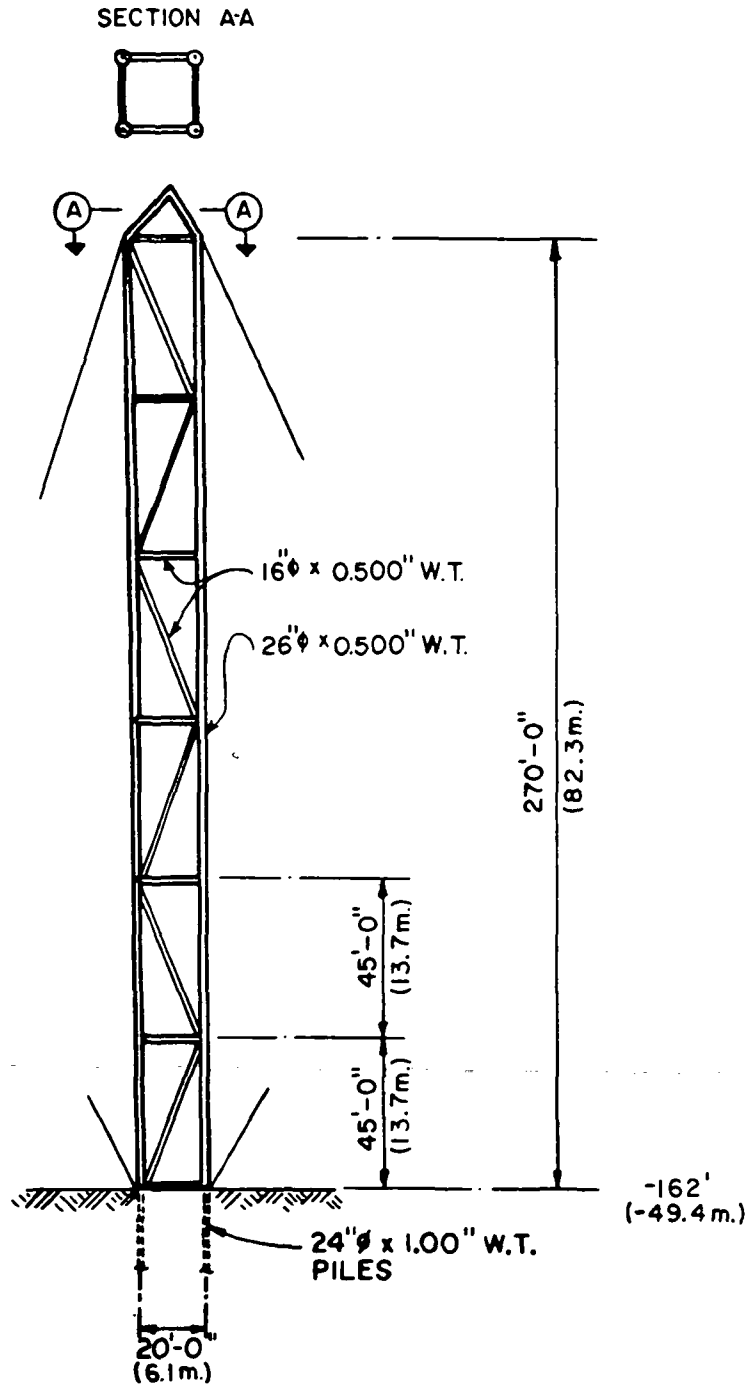
FIGURE 5.1.1 PRIME SITE GUYED TOWER STRUCTURE
