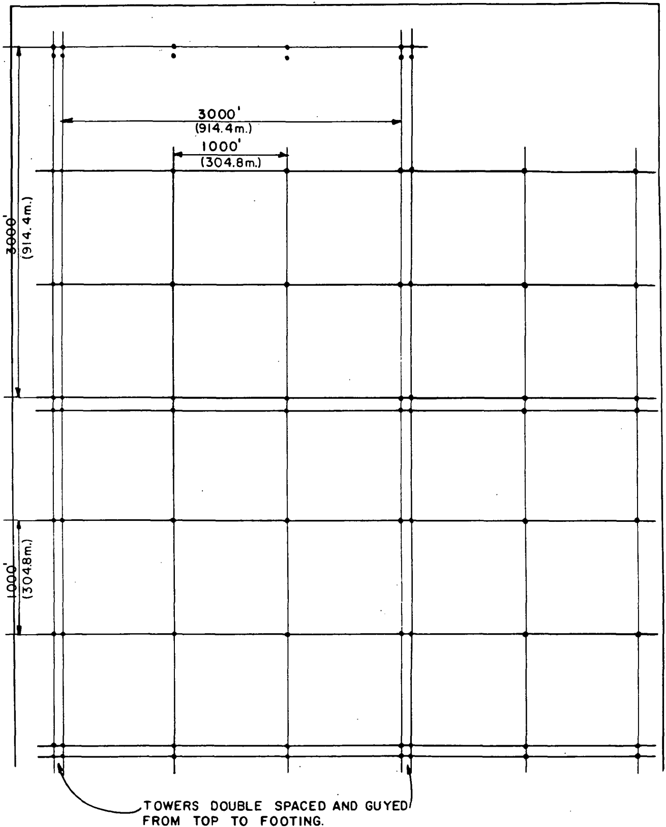
FIGURE 6.1.2 CONFIGURATION OF SUPPORT TOWERS AND PERIMETER TAUT LINE CABLES IN PREFERRED DESIGN.
