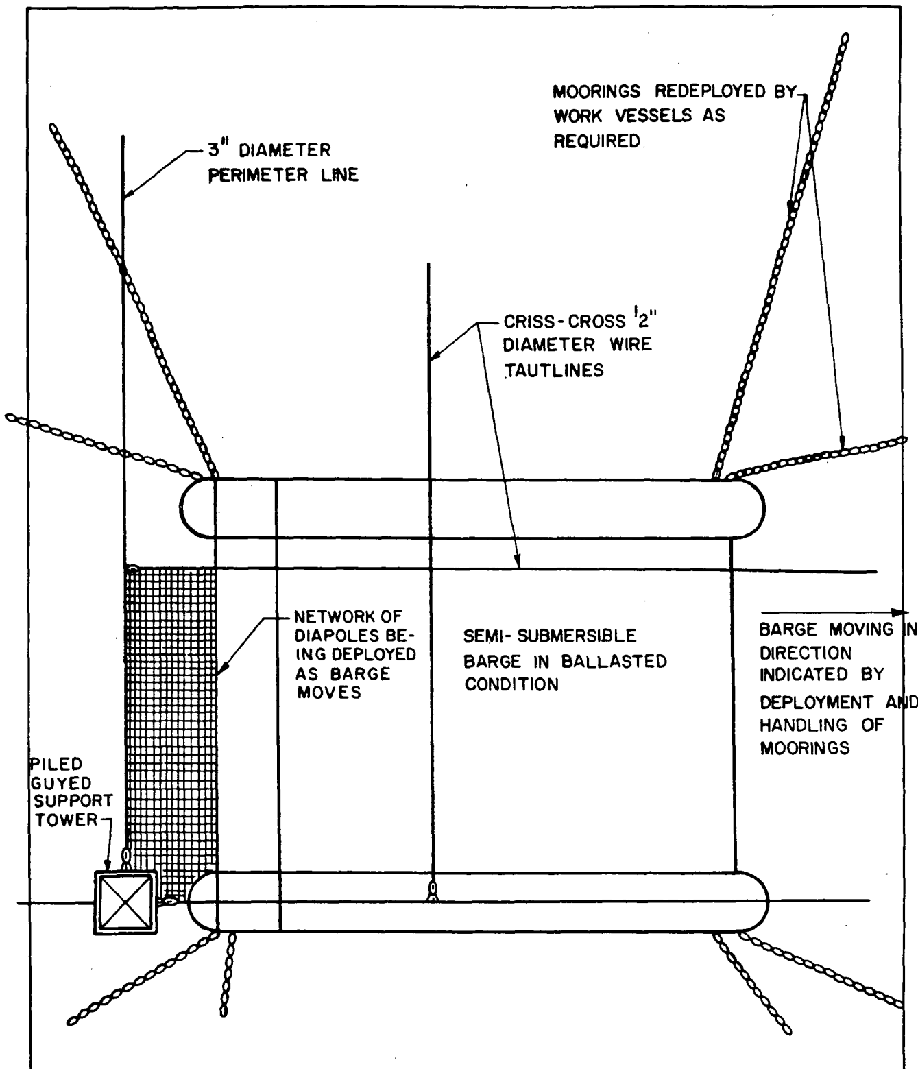
FIGURE 6.2.2 DIPOLE NETWORK INSTALLATION ON TAUTLINES
