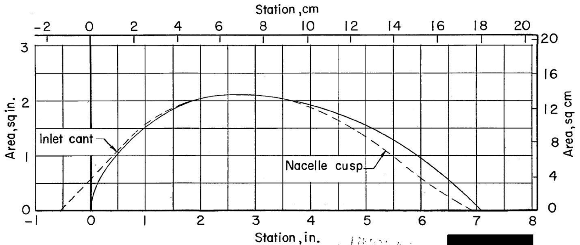
Figure 3.- Flow-through nacelle area distribution (stream tube area removed).
