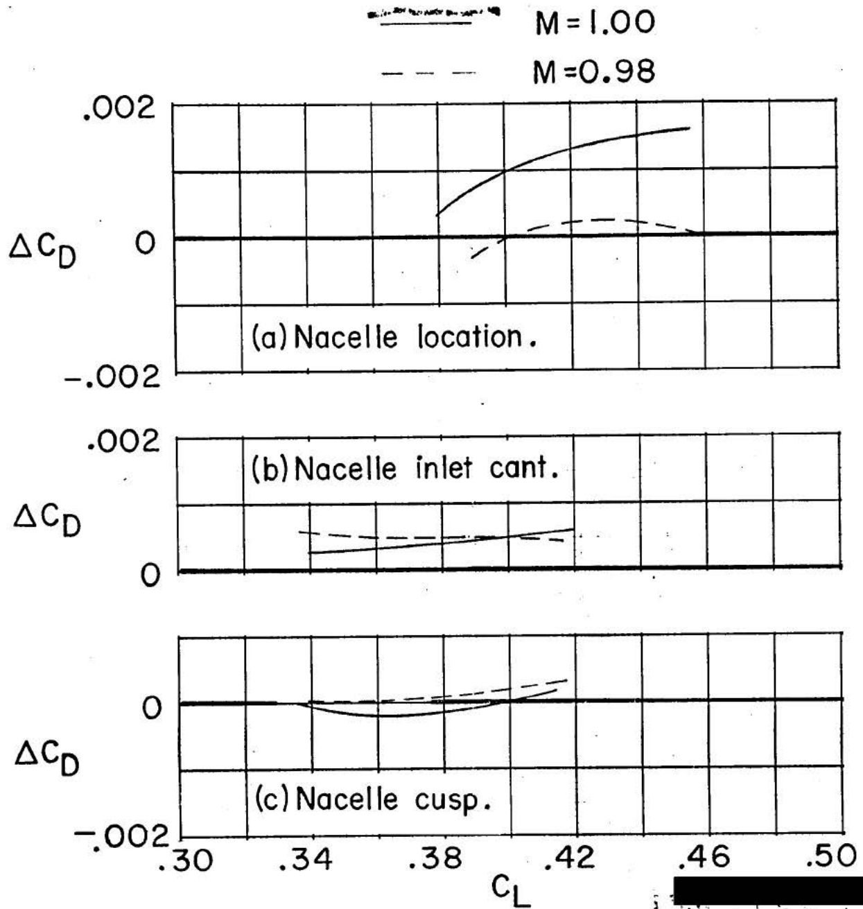
Figure 4.- Variation of drag differential with lift coefficient.
