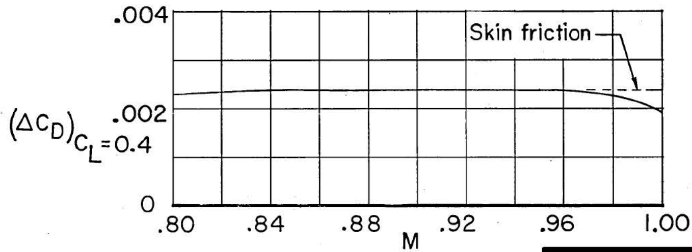
Figure 6.- Variation of drag differential with Mach number at 0.4 lift coefficient. Equivalent body.
