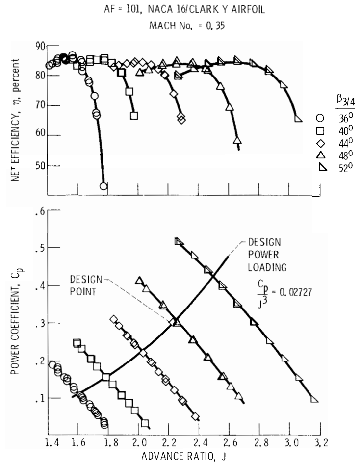
Figure 8. - Typical low speed propeller test results.
