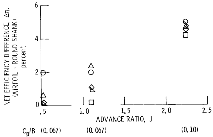
Figure 11. - Performance effect of improved blade shank design.
