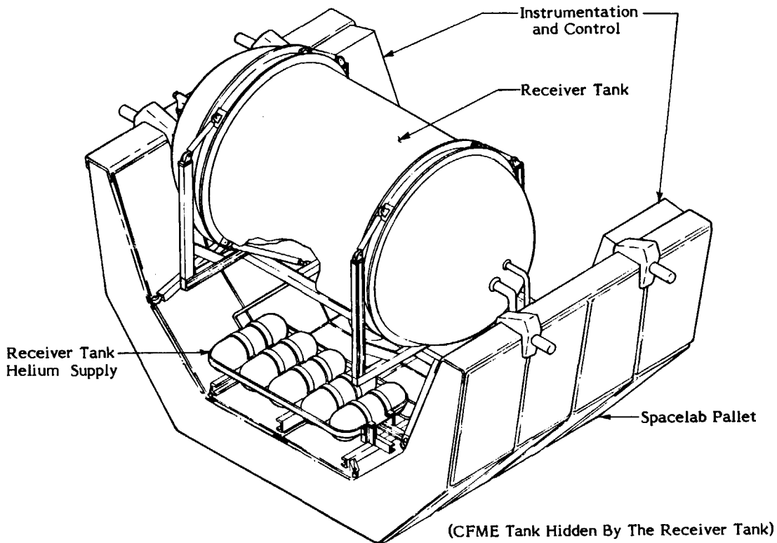
Figure 2-17 CFMF PHASE I SPACELAB PALLET
