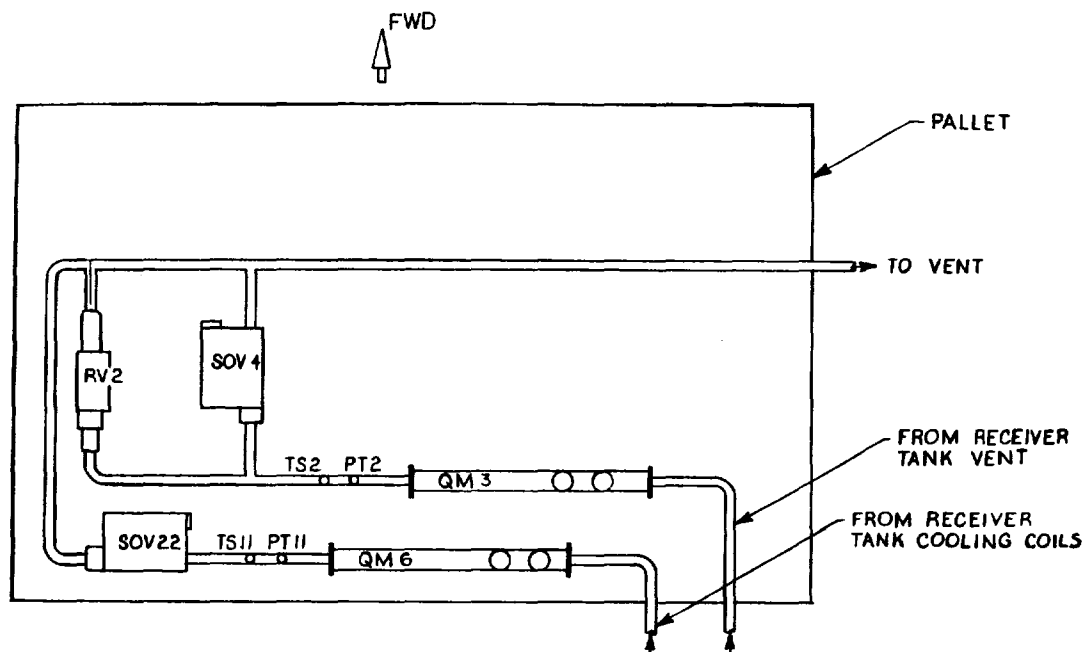
Figure 3-25 PHASE II INSTRUMENTATION AND CONTROL PALLET B
