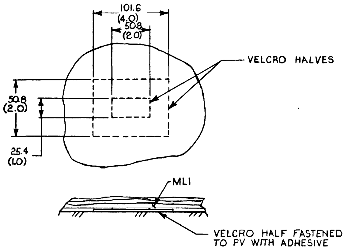
Figure 3-5 INSULATION ATTACHMENT
