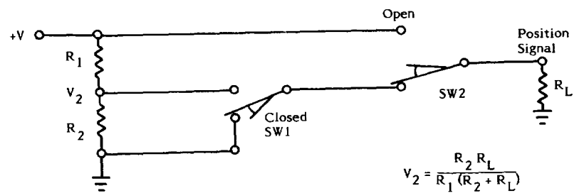
Figure 3-29 SOLENOID VALVE POSITION INDICATOR
