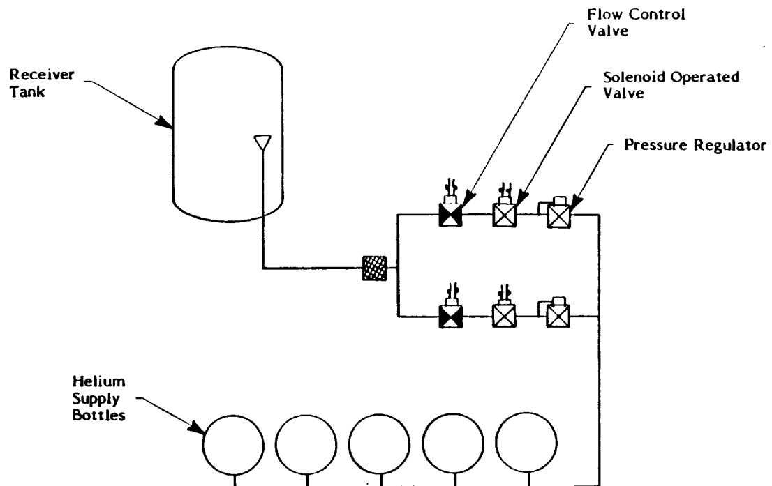
Figure 3-19 ALTERNATE PRESSURIZATION SYSTEM
