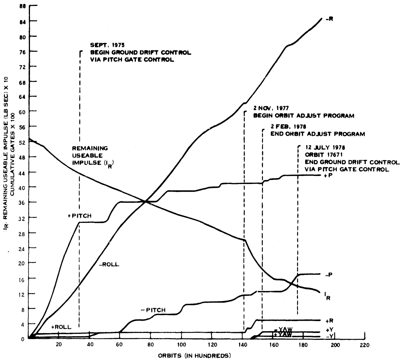
Figure 4-4. Landsat-2 Gating History
