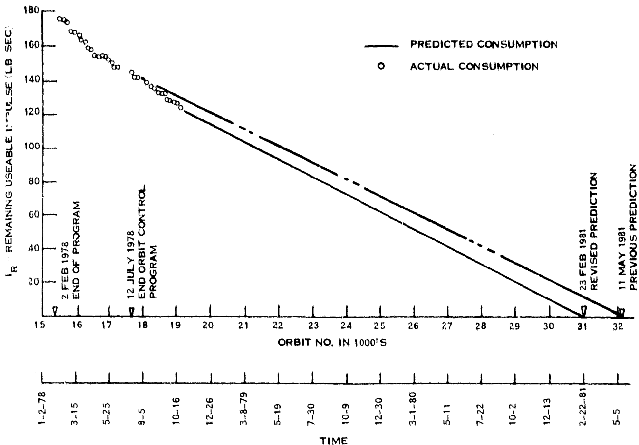
Figure 4-1. Landsat-2 Freon Status - Long Term Predicted Freon Life vs Current Freon Remaining Useable Impulse
