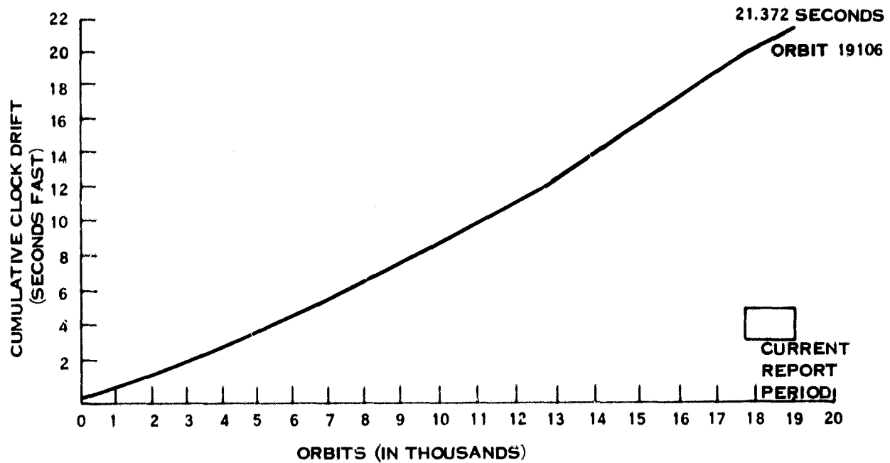
Figure 5-2, Cumulative Clock Drift
