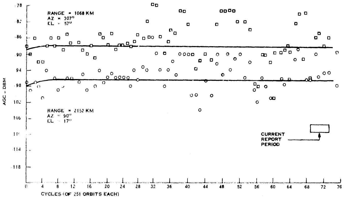
Figure 9-1. USB (Link 4) AGC Readings at Goldstone with 30' Antenna - Landsat-2
