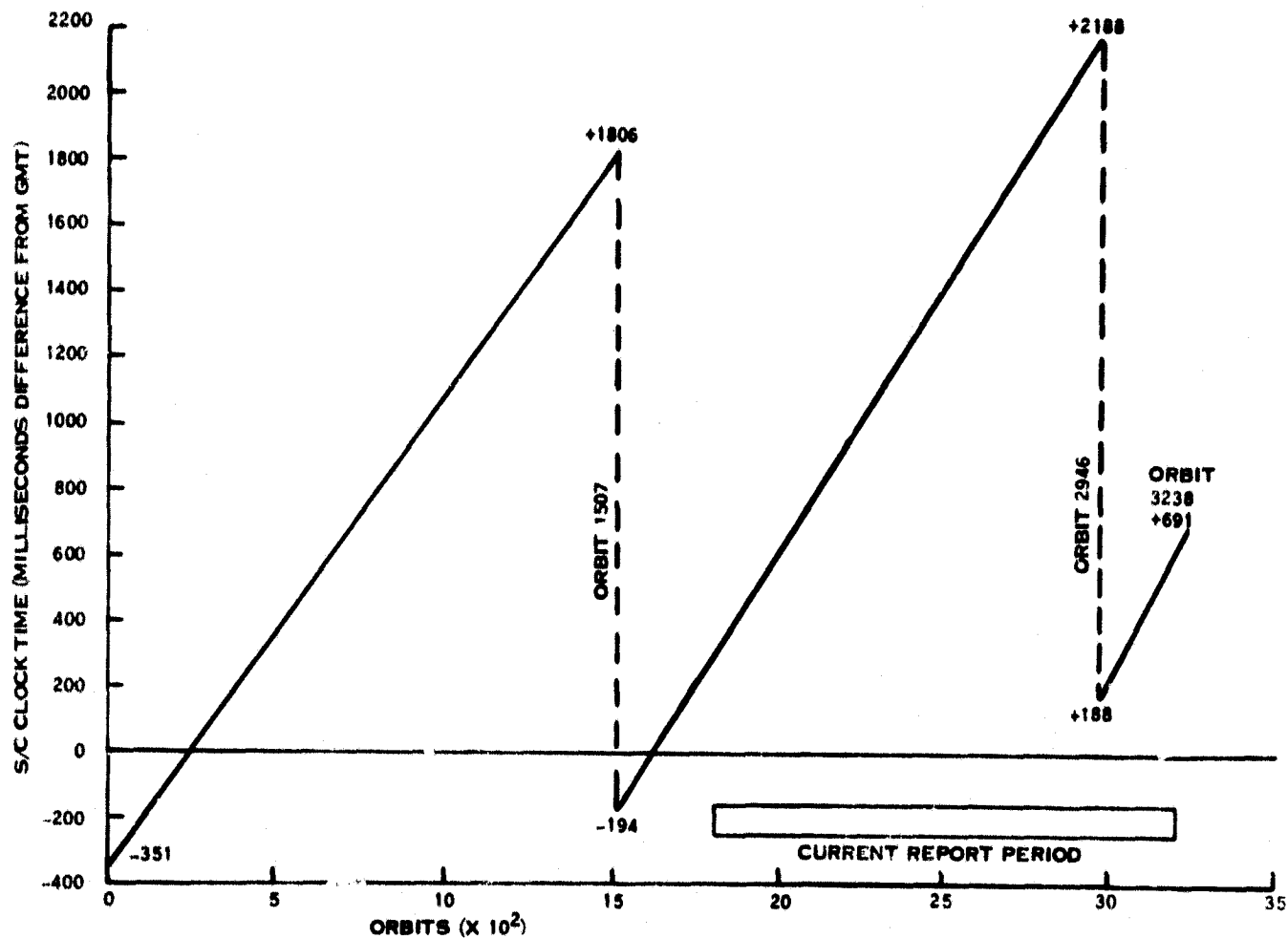
Figure 5-1. Landsat-3 Drift History
