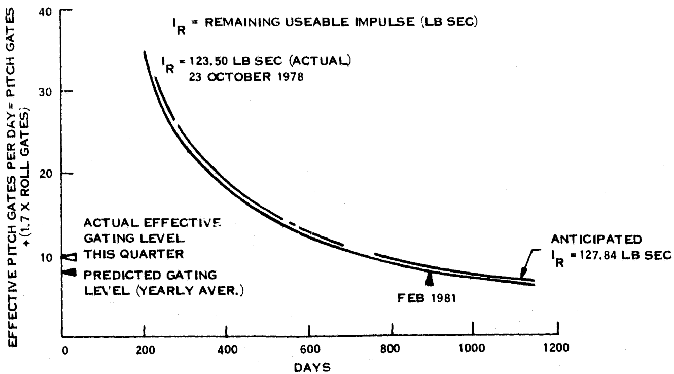
Figure 4-2. Landsat-2 Freon Life Expectancy Based on this Period's Consumption - Ref. 23 October 1978
