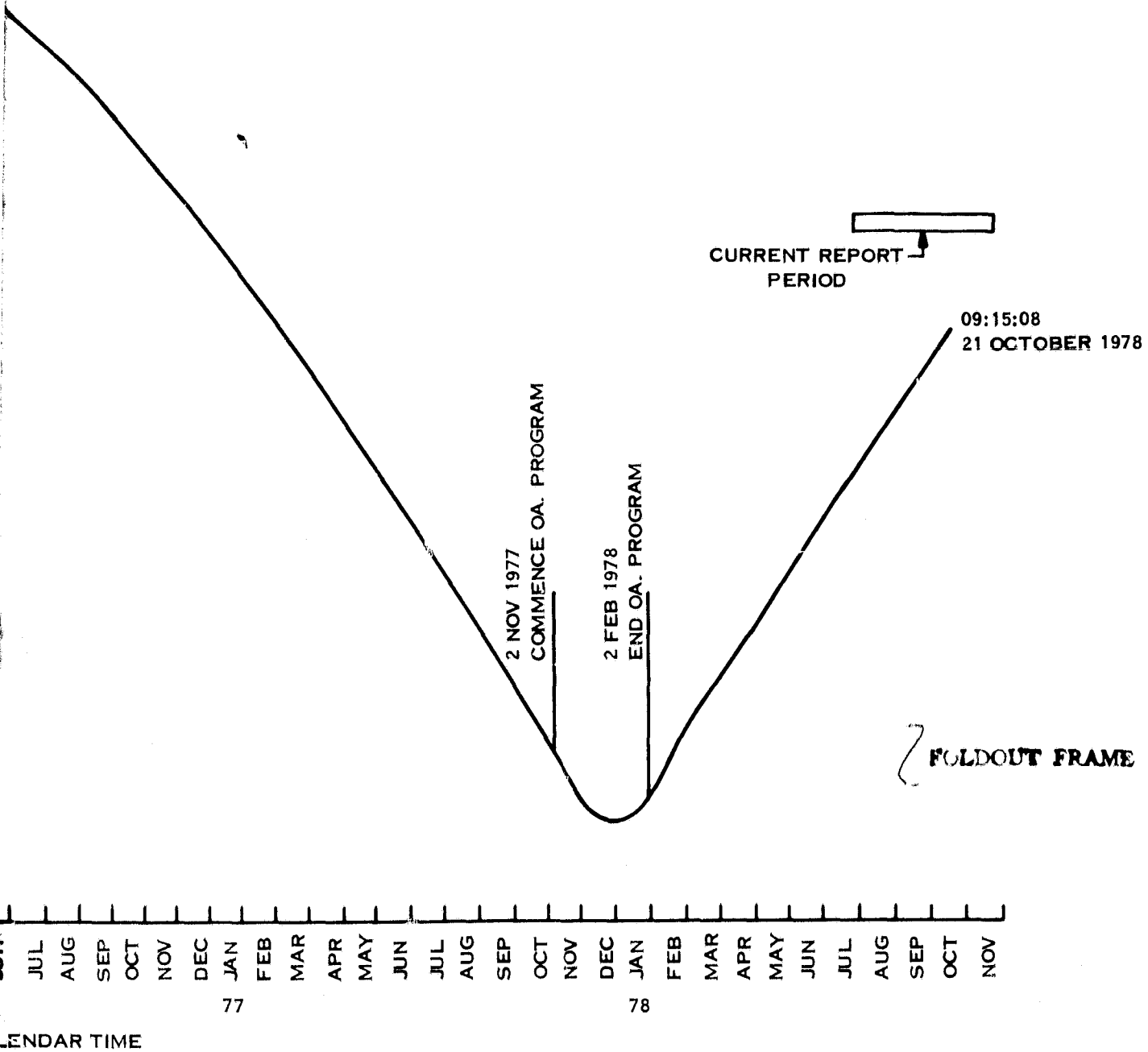
Figure 2-2. Local Mean Time of Descending Node - Landsat-2
