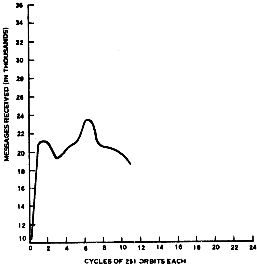
Figure 18-1. Landsat-3 Number of DCS Messages for an 18-Day Cycle
