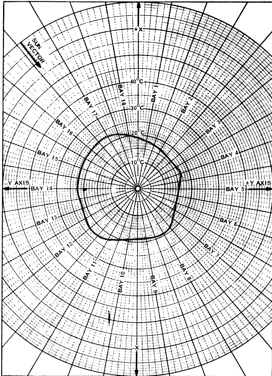
Figure 11-1. Landsat-2 Sensor Ring Average Temperatures Orbit 19001, 6 October 1978
