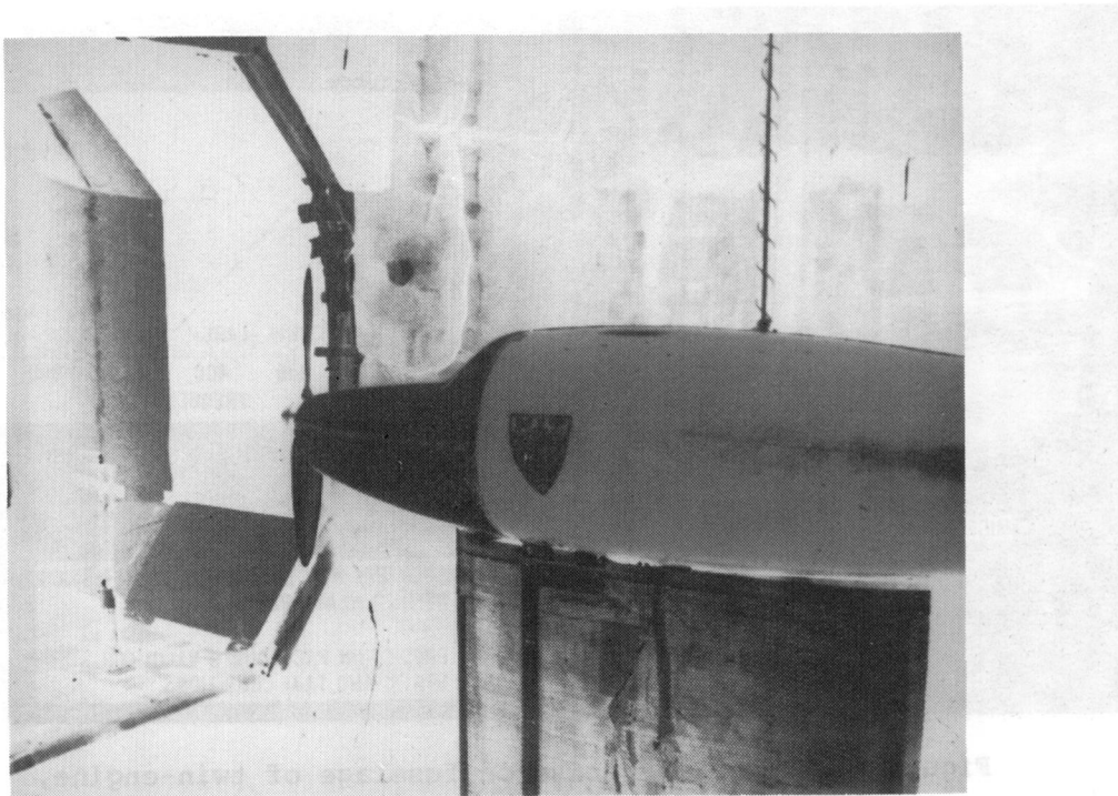
Figure 7.- Acoustic tests of quiet general aviation propellers in anechoic wind tunnel.
