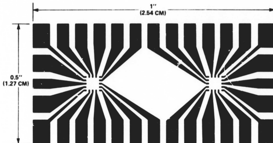
TWO-CHIP SUBSTRATE METALLIZATION PATTERN
