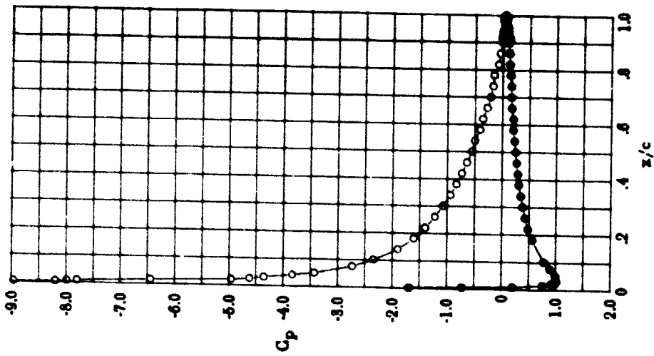
(m) M=0.300 ; \alpha=14.06
