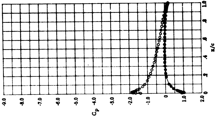
(e) M=0.300 ; c_u = 0.577 ; \alpha = 6.66
