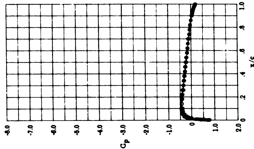
(c) M=0.361 ; c_{x_0}=1.067 ; \alpha=10.86
