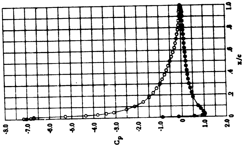
(k) M=0.349 ; \alpha=13.86
