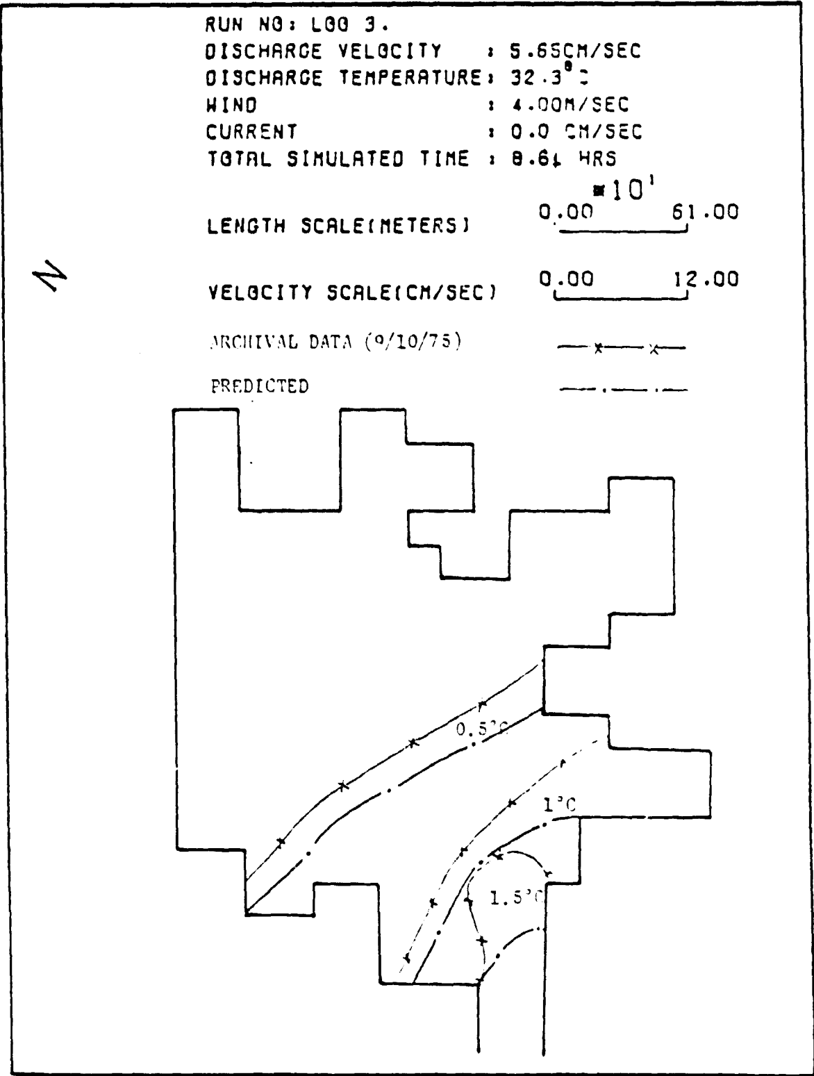
Figure 26. Isotherms: measured and predicted (temperatures above ambient)
