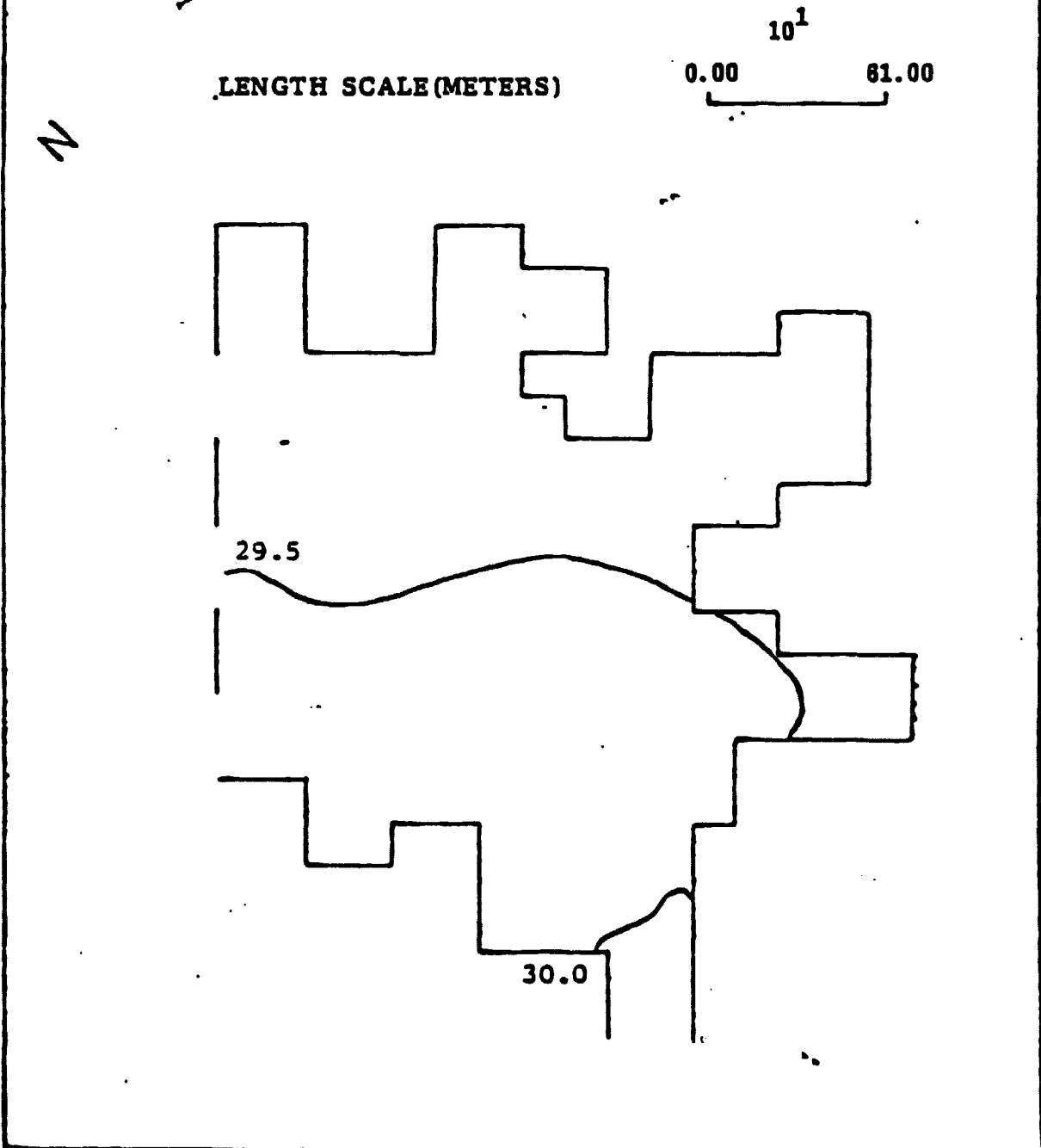
Figure 38. Isotherms at K = 1 , Lake Keowee (rigid-lid model), simulations for August 25, 1978
