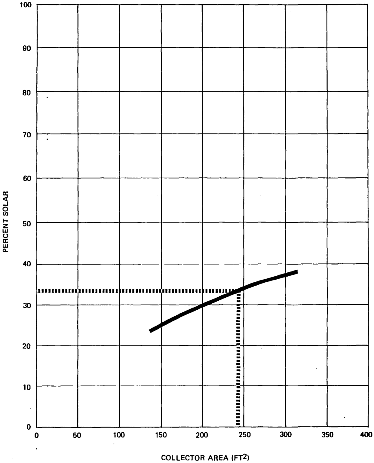
Figure 5.1-1 (a) Solar Fraction vs Collector Area for Solar Energy System at Tunkhannock, Pennsylvania
