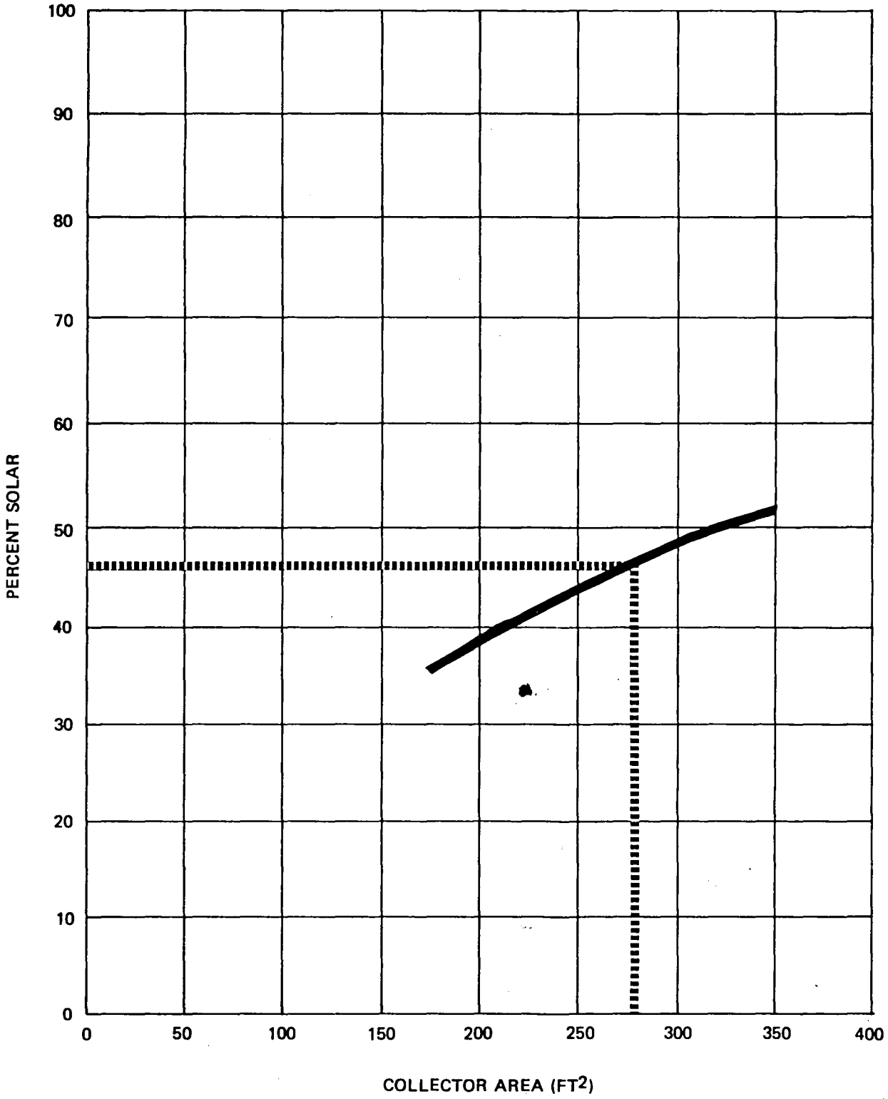
Figure 5.1-1 (e) Solar Fraction vs Collector Area for Solar Energy System at Washington, D. C.
