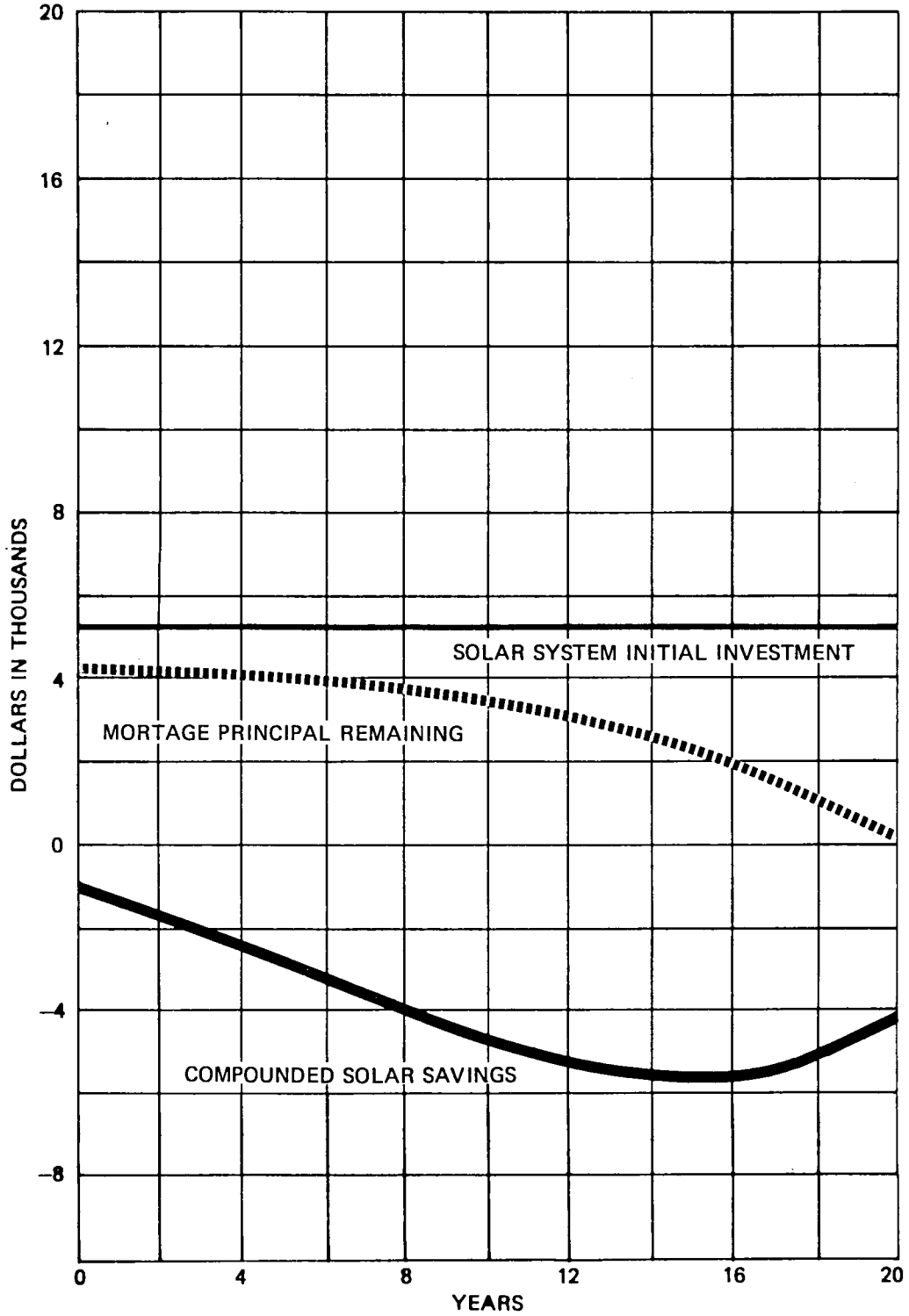
Figure 5.2-3 (d) Payback for Solar Energy System for Madison, Wisconsin
