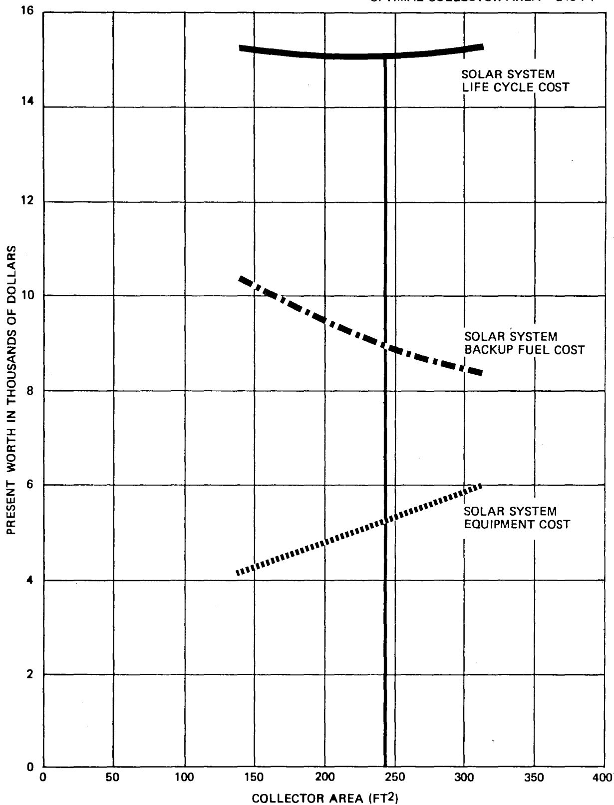
Figure 5.2-1 (a) Optimization of Collector Area for Tunkhannock, Pennsylvania
