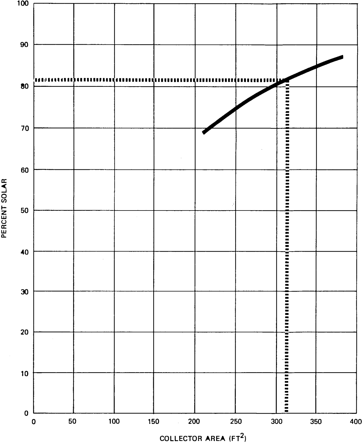
Figure 5.1-1 (b) Solar Fraction vs Collector Area for Solar Energy System at Albuquerque, New Mexico
