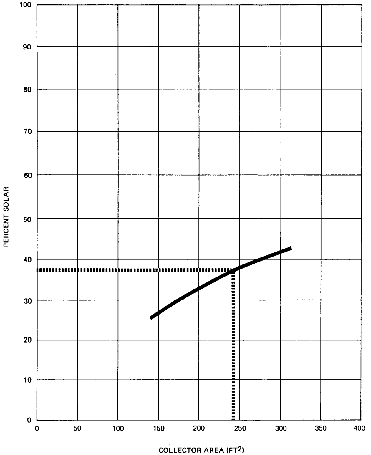
Figure 5.1-1 (d) Solar Fraction vs Collector Area for Solar Energy System at Madison, Wisconsin
