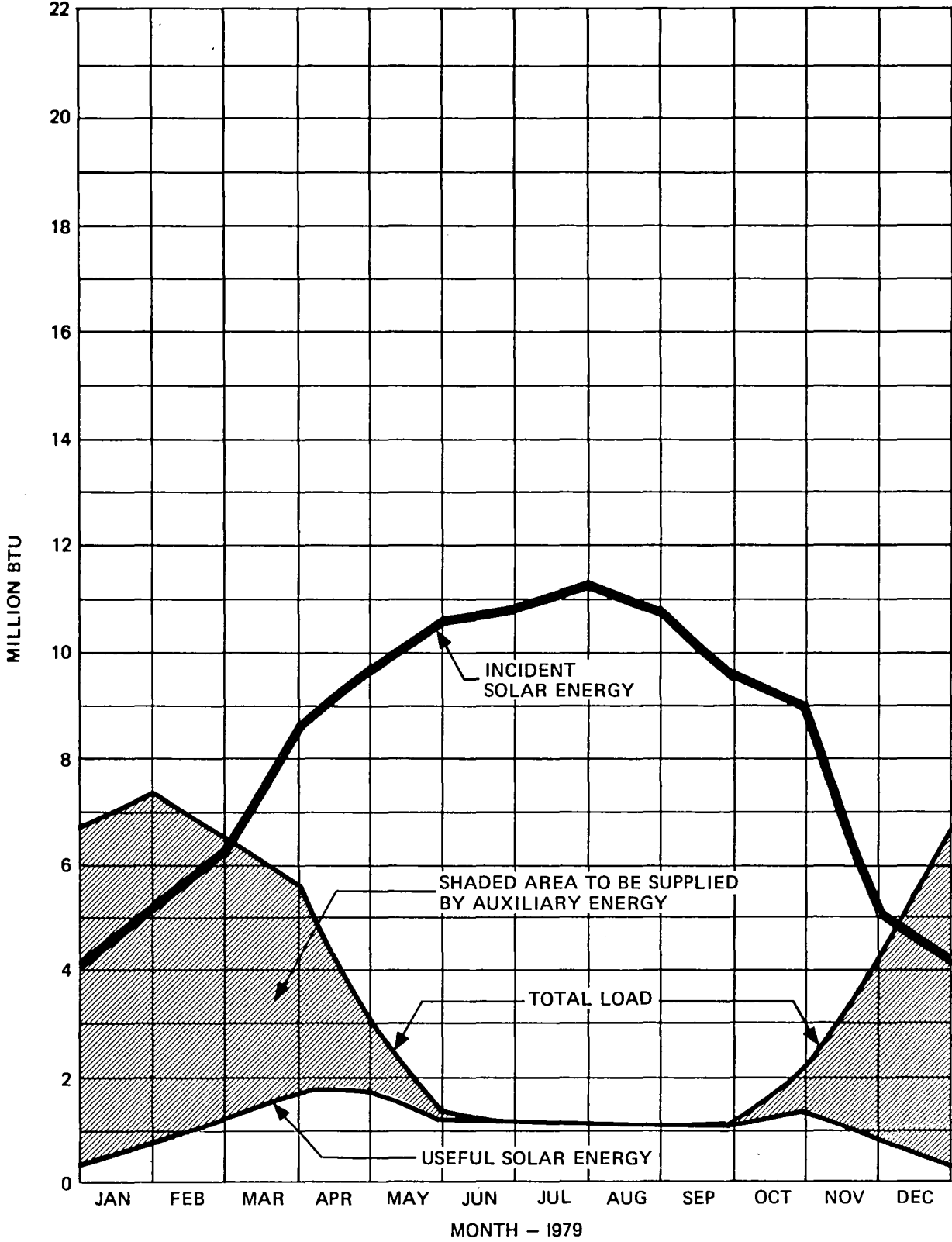
Figure 5.1-2 (a) Thermal Performance of Solar Energy System with Optimized Collector Area for Tunkhannock, Pennsylvania
