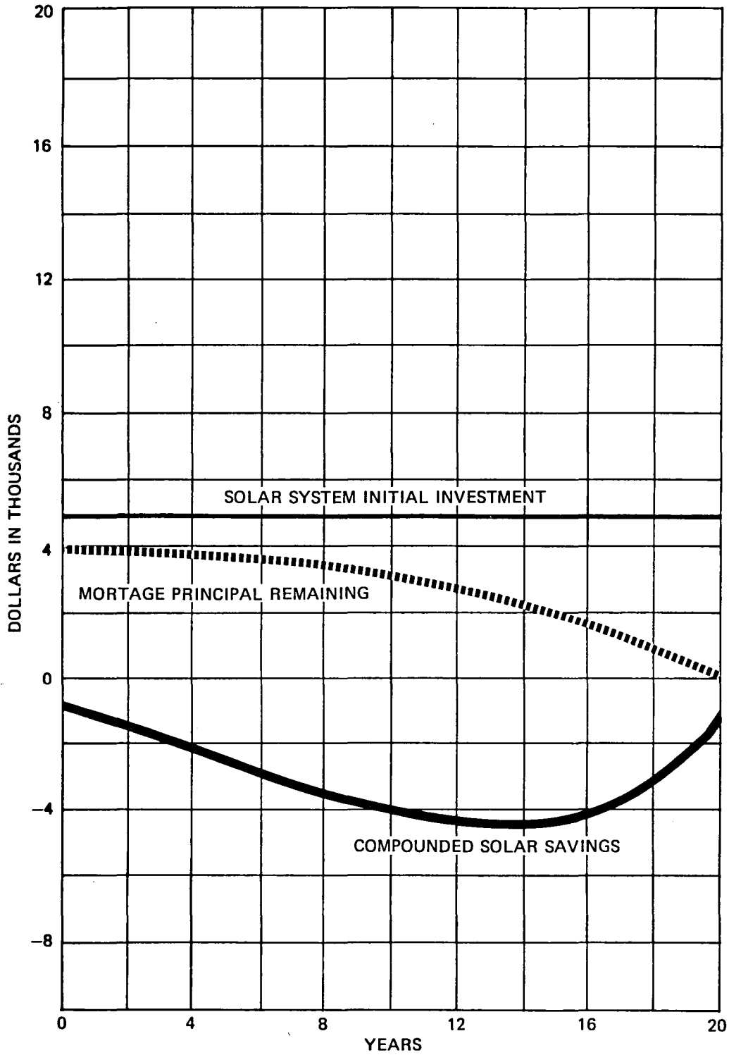
Figure 5.2-3 (c) Payback for Solar Energy System for Fort Worth, Texas
