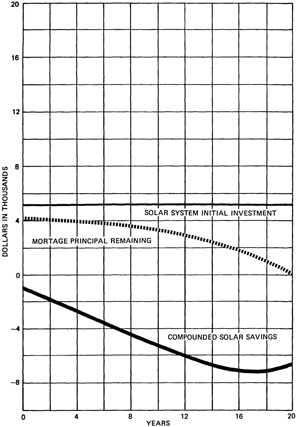
Figure 5.2-3 (a) Payback for Solar Energy System for Tunkhannock, Pennsylvania
