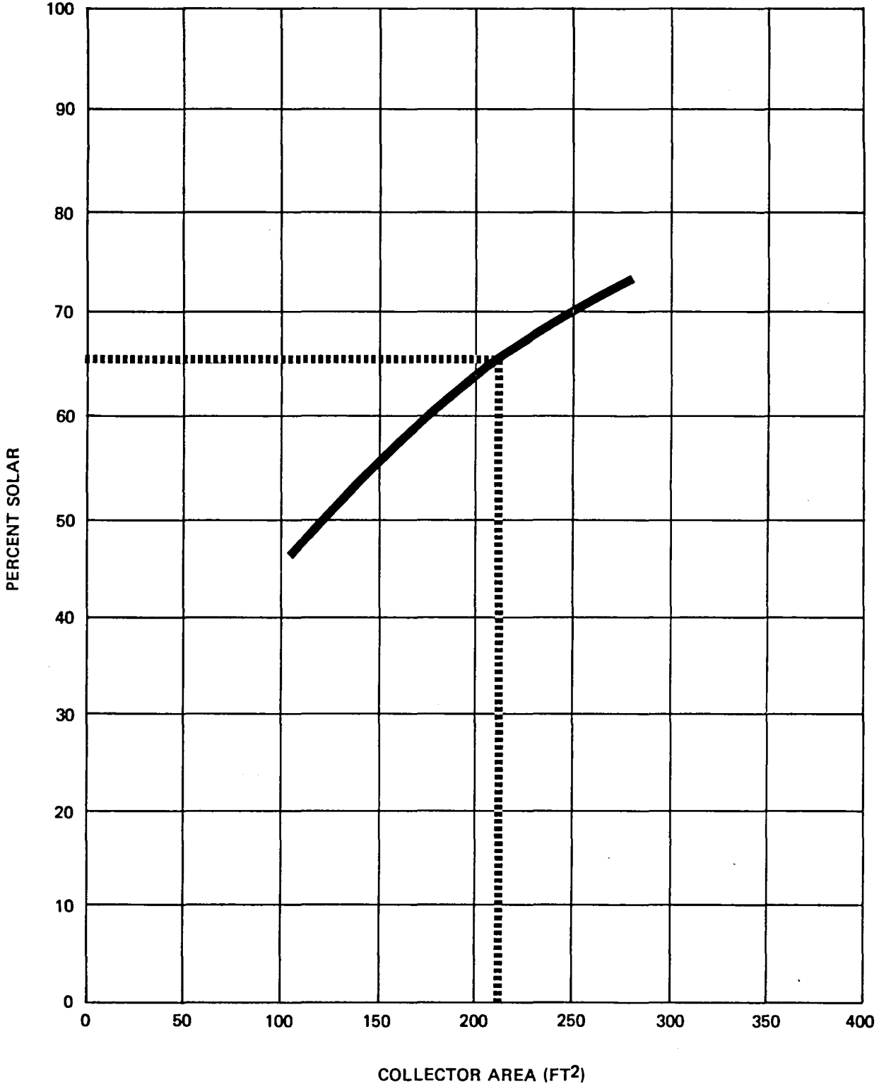
Figure 5.1-1 (c) Solar Fraction vs Collector Area for Solar Energy System at Fort Worth, Texas
