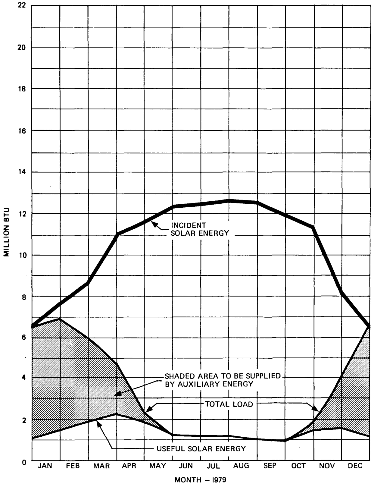
Figure 5.1-2 (e) Thermal Performance of Solar Energy System with Optimized Collector Area for Washington, D.C.
