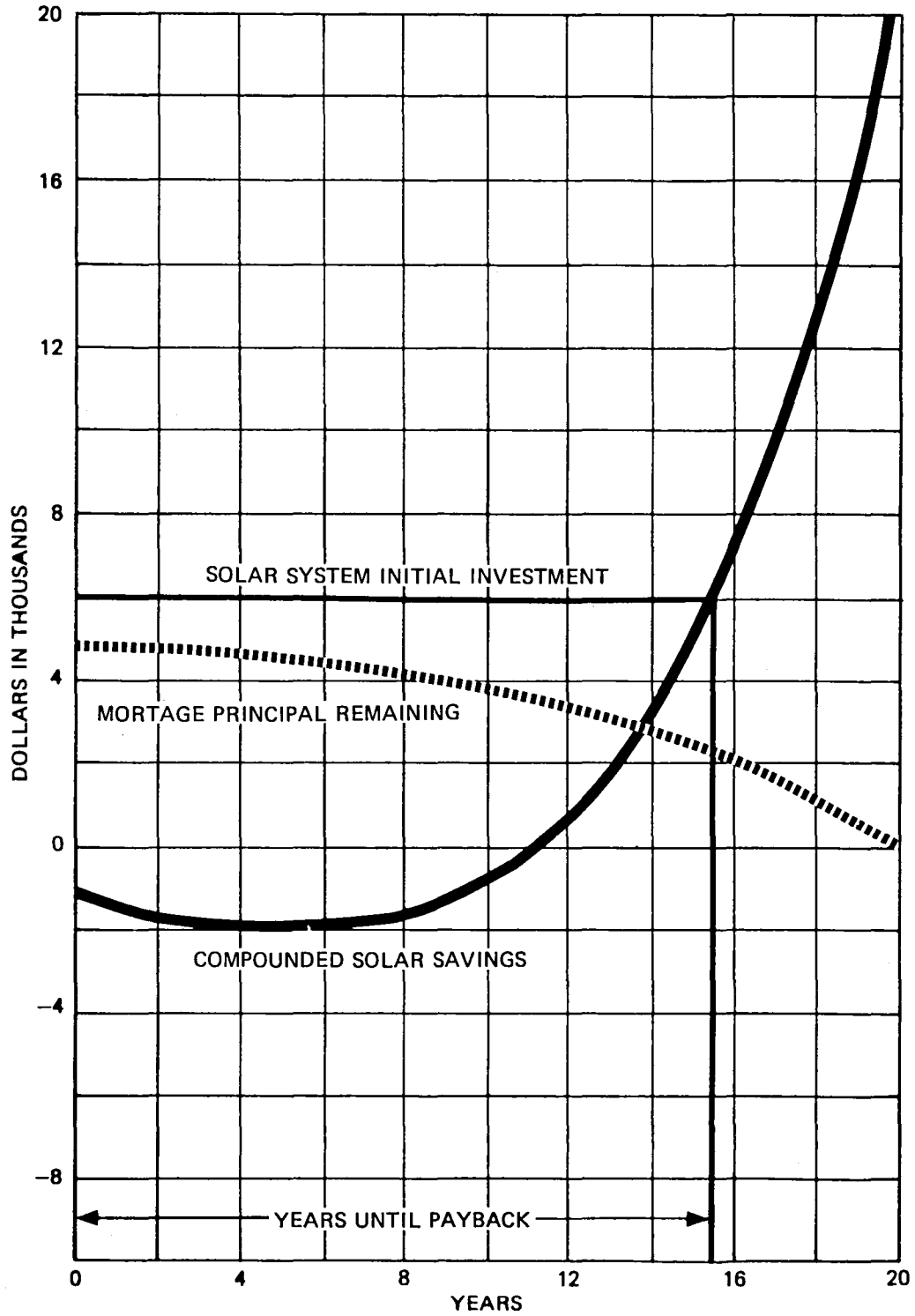
Figure 5.2-3 (b) Payback for Solar Energy System for Albuquerque, New Mexico
