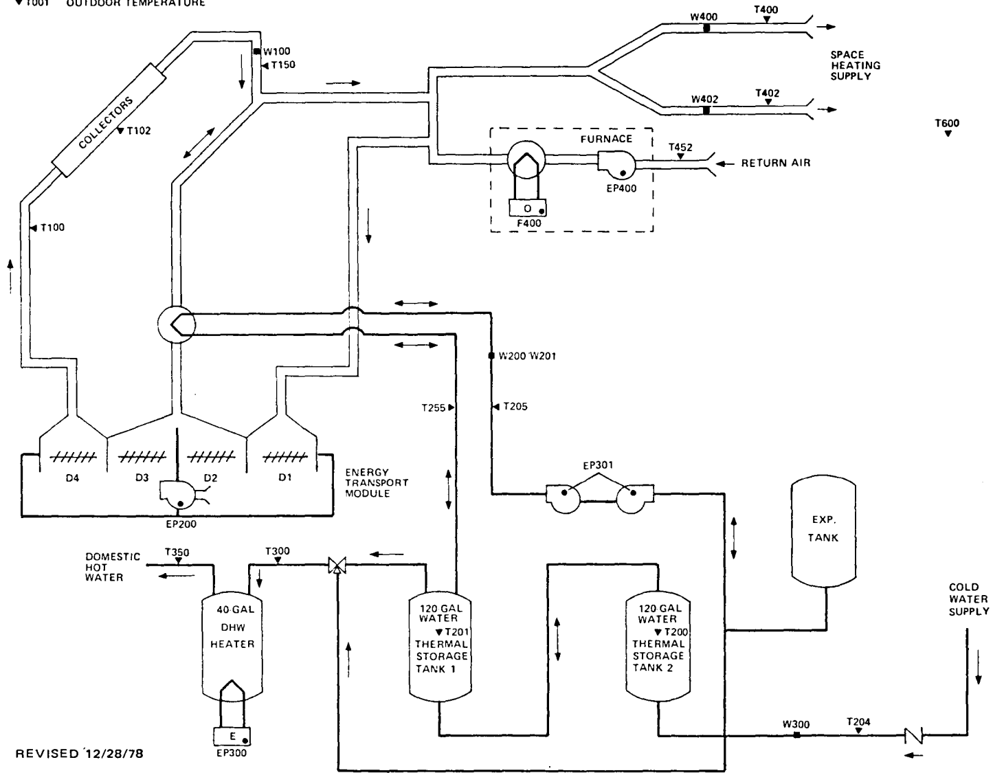
Figure 2-1 Fern Tunkhannock Solar Energy System Schematic
