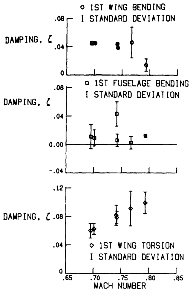
(a) Damping
