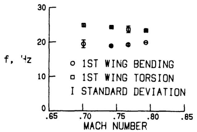
(b) Frequency
