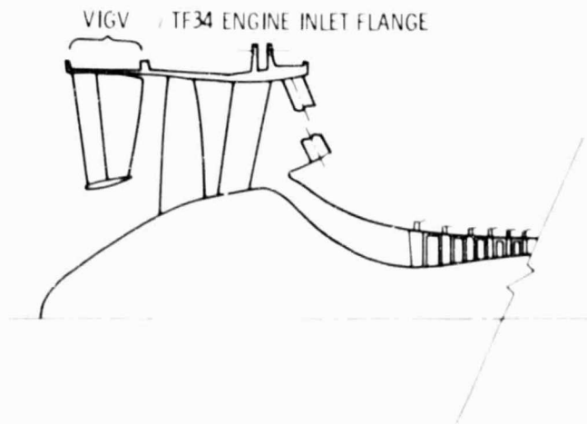
Figure 4. - Cross-section of VIGV installed ahead of TF34 turbfan engine.
