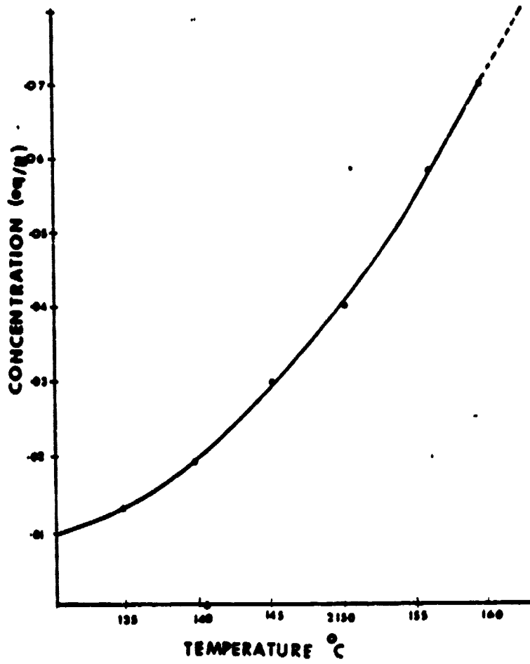
FIGURE 18. CONCENTRATION OF TOTAL BASE AS A FUNCTION OF TEMPERATURE IN DMAC/TOLUENE SYSTEM
