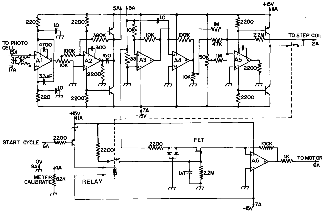
Figure 4.- Wiring diagram of the electronic circuit.
