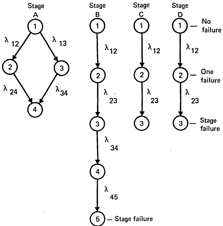
MARKOV MODELS
