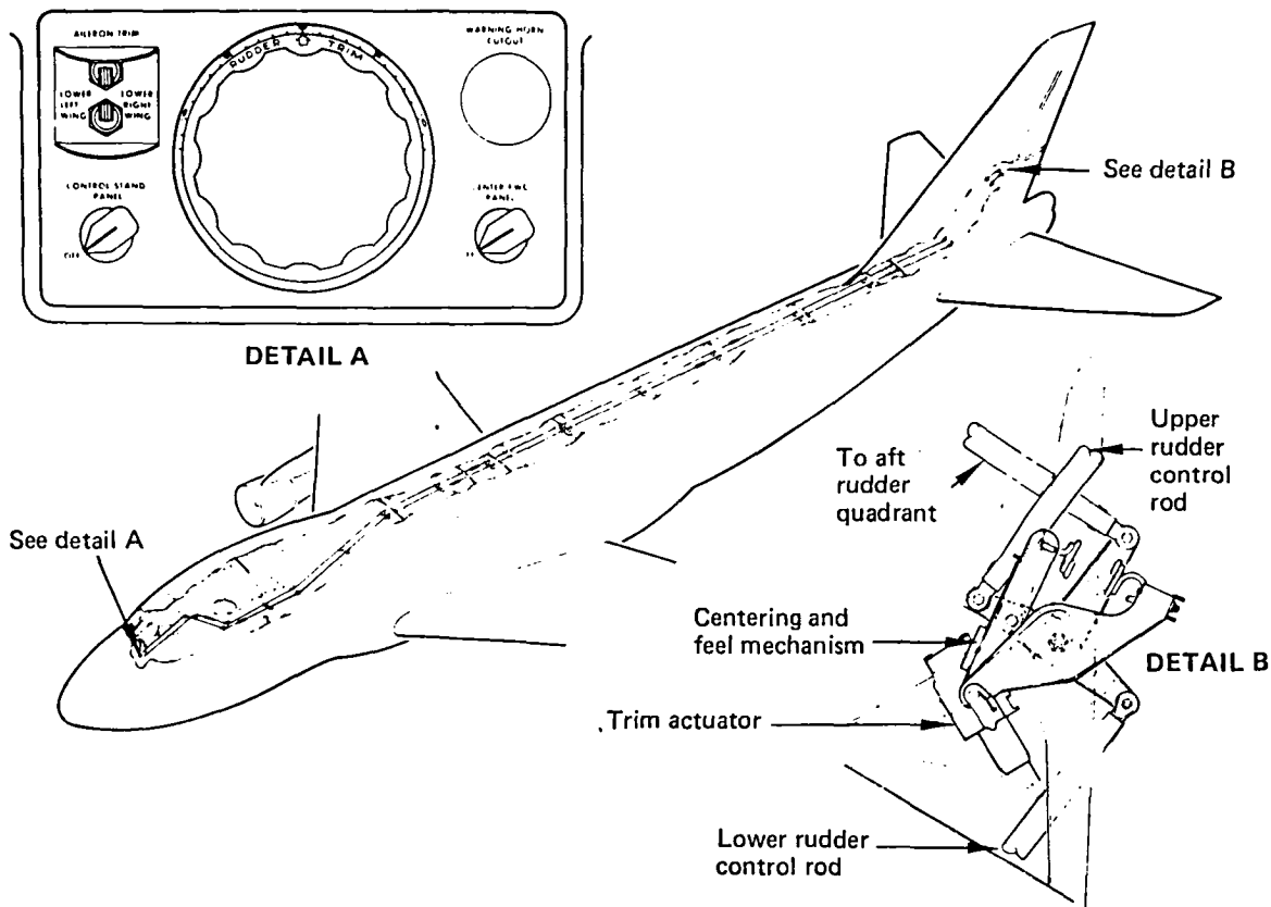
Figure 20. Rudder Trim System
