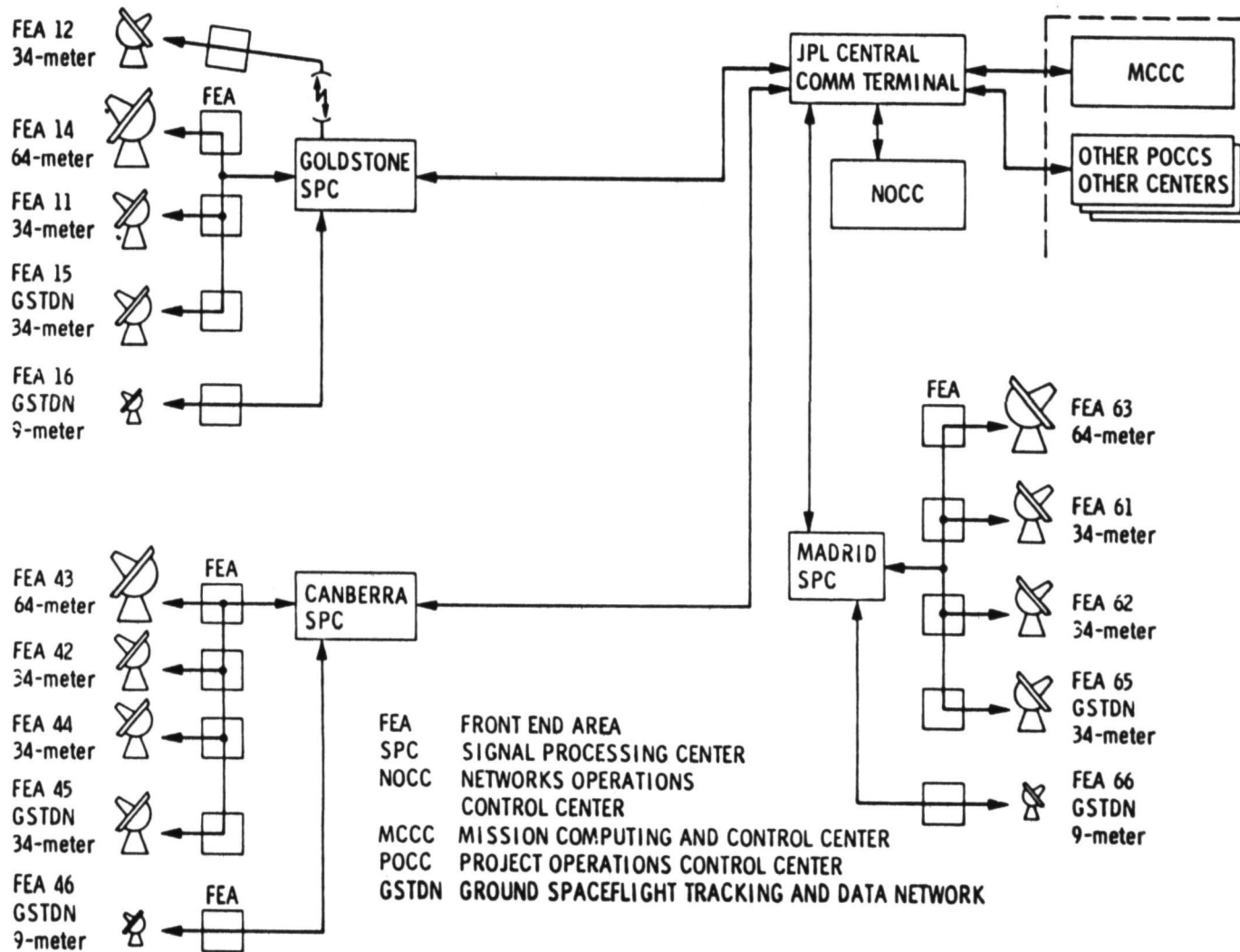
Fig. 2—Consolidated Network Configuration - 1986
