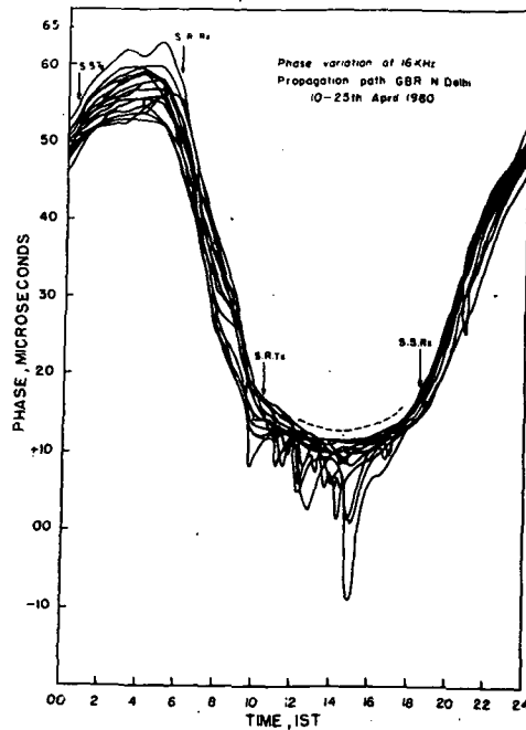
Fig. 2 Diurnal variation of GBR phase for 15 days in April 1980 compared with the variation of M(1-\overline{\cos\chi}) (dotted line) around midday.
