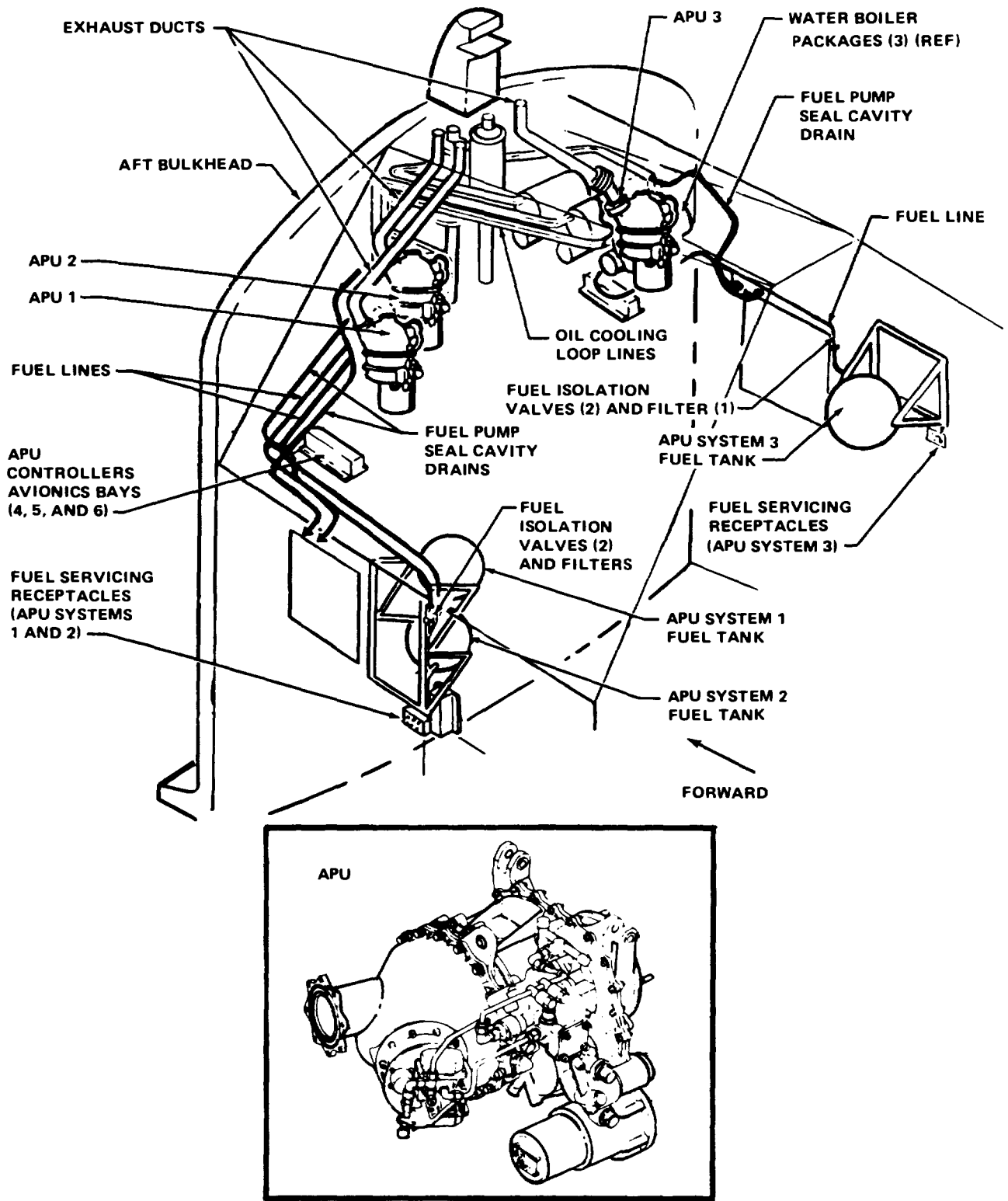
Figure 4-5.—Orbiter auxiliary power unit system.
