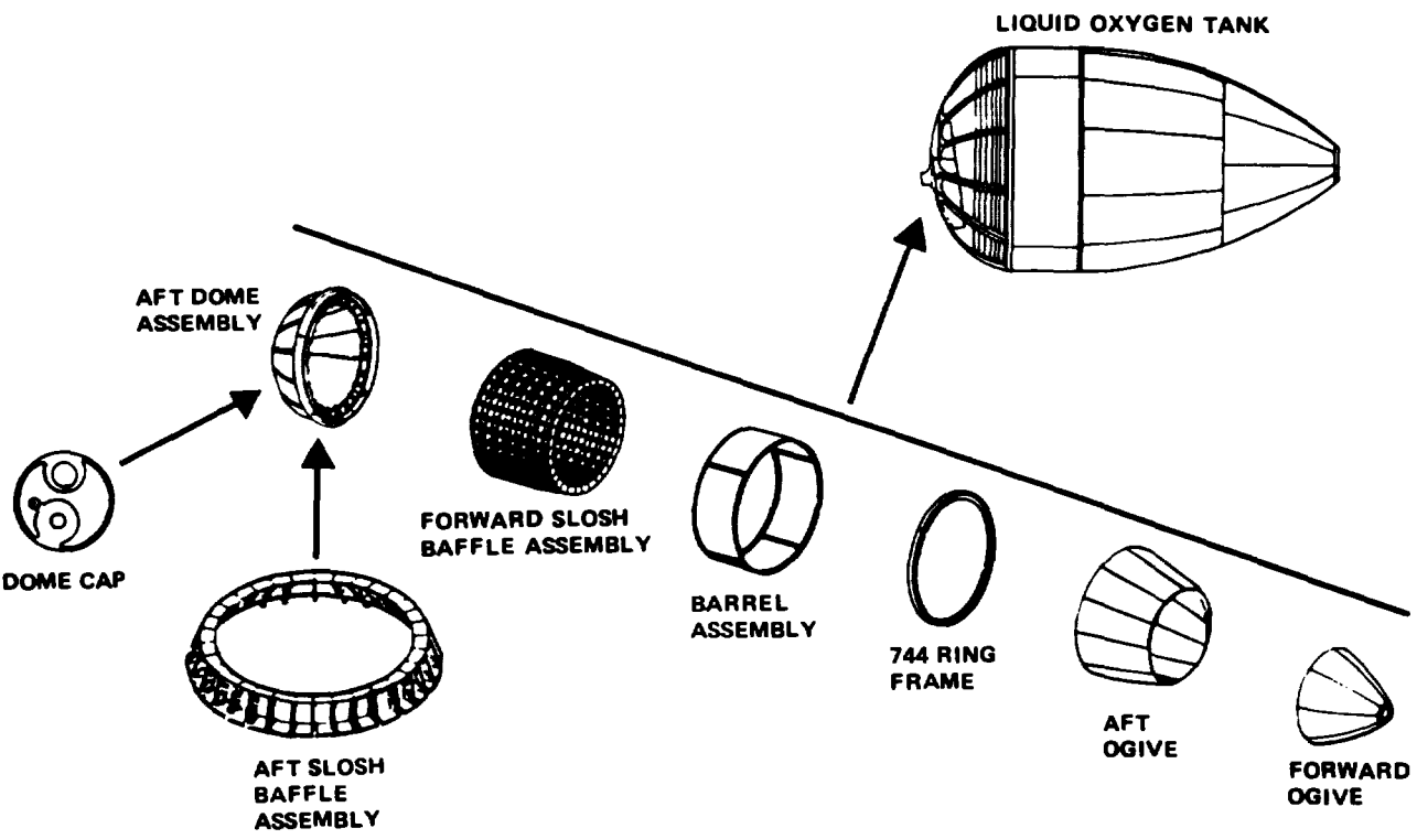
Figure 2-18.—ET liquid oxygen tank structural assembly.
