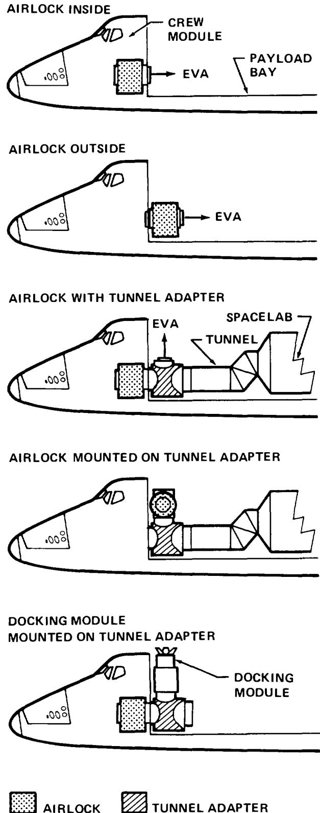
Figure 5-16.—Airlock/tunnel adapter configurations.
