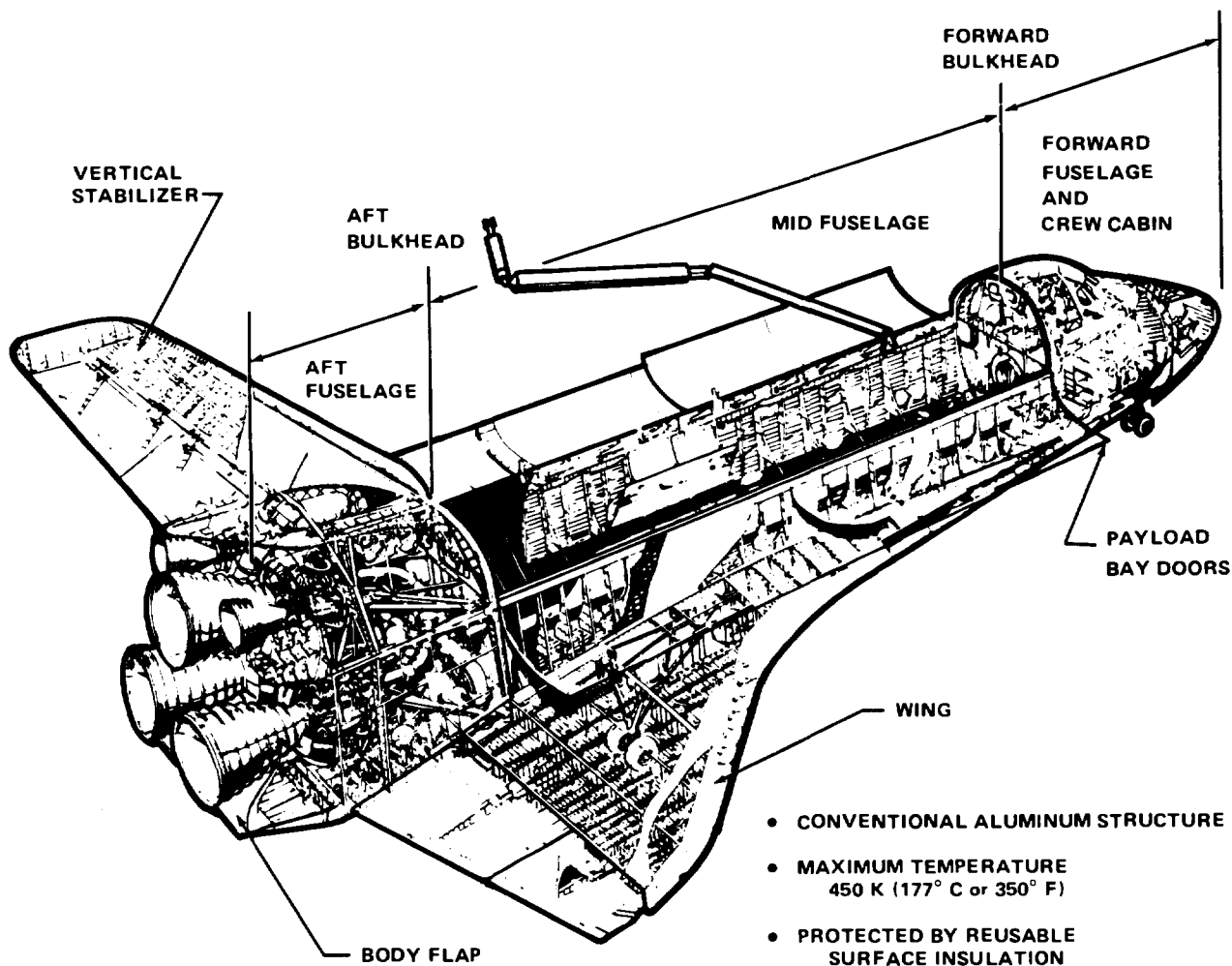
Figure 3-1.—Orbiter structures.
