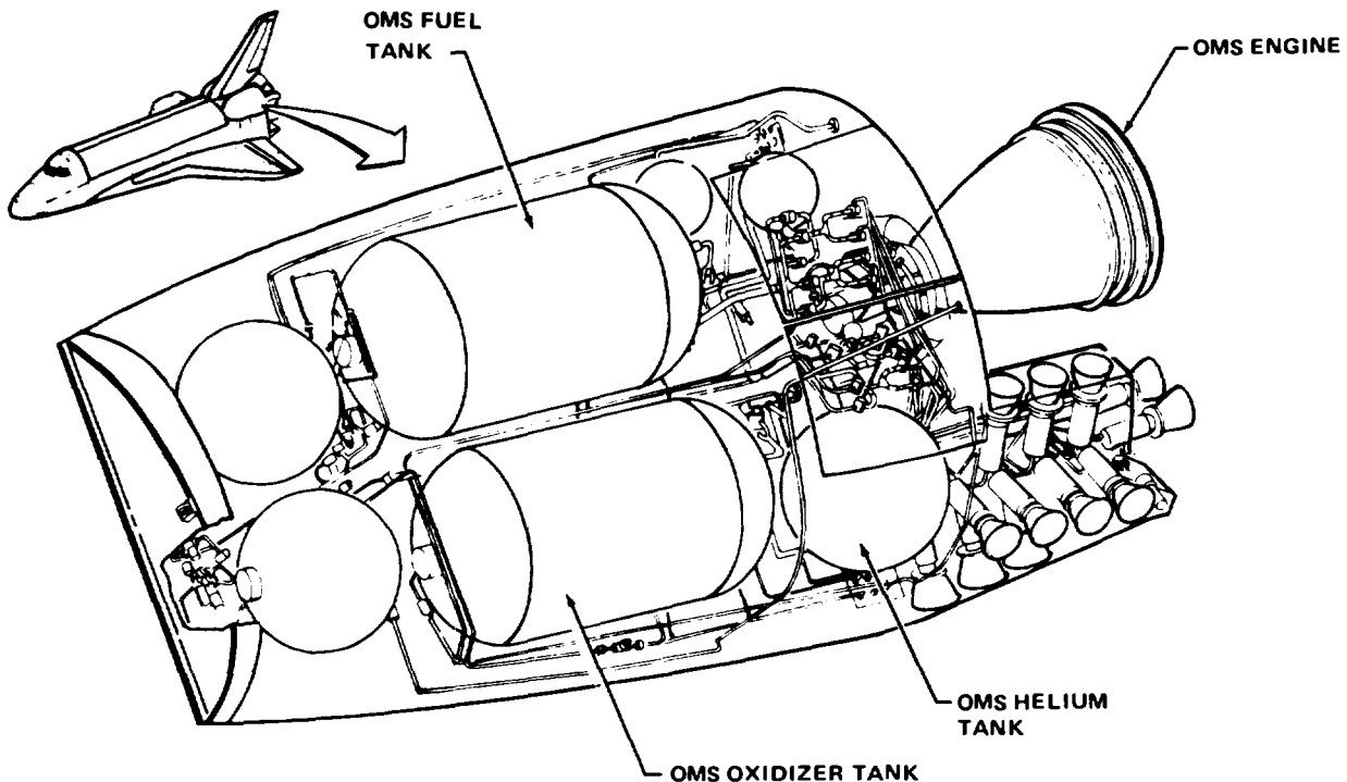
Figure 4-1.— Orbital maneuvering system.
