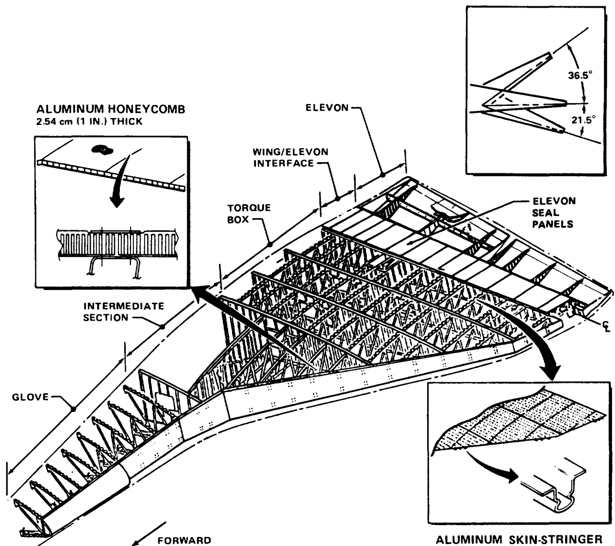
Figure 3-18.—Wing.
