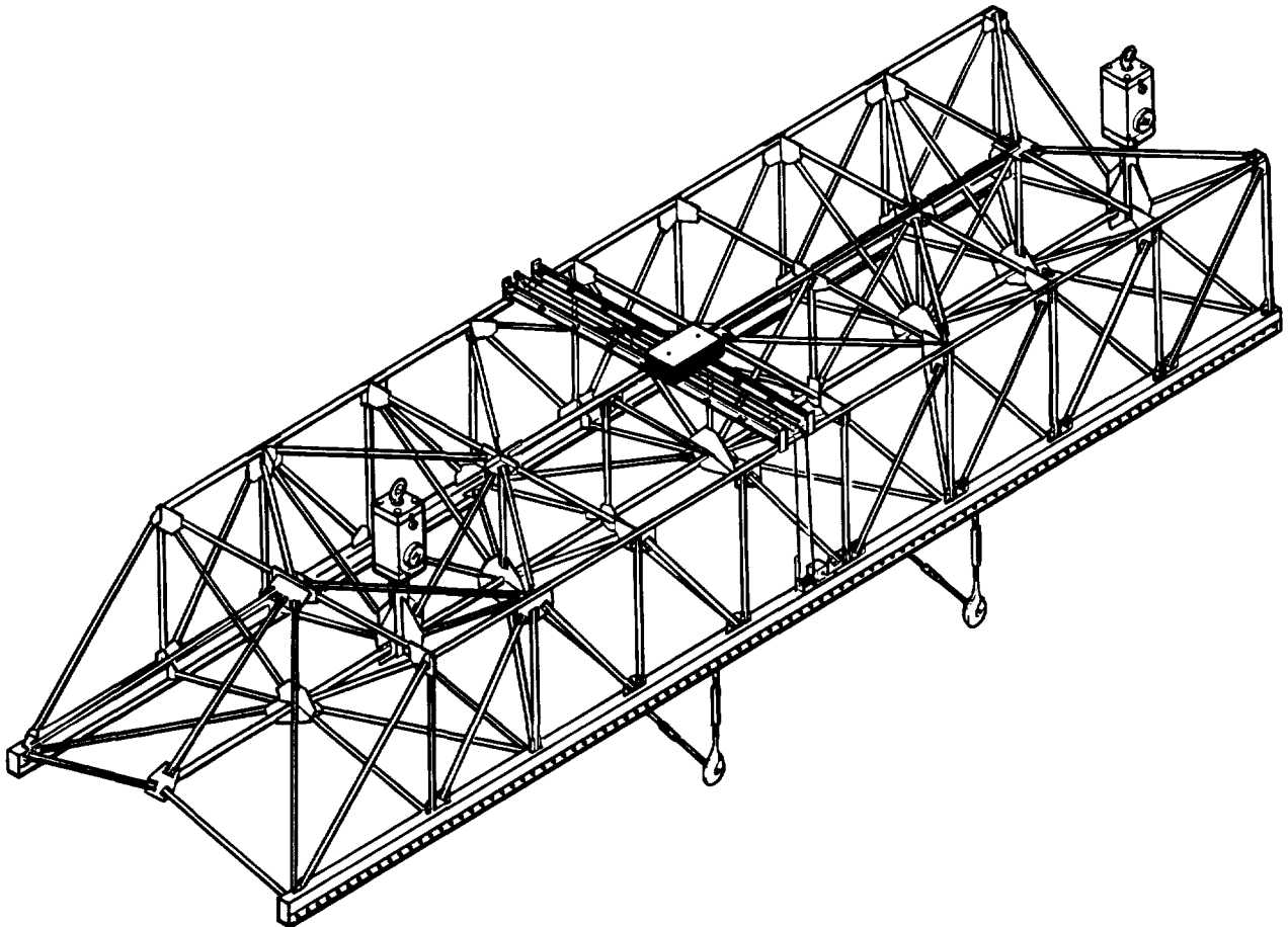
Figure 6-14.—Payload strongback.
