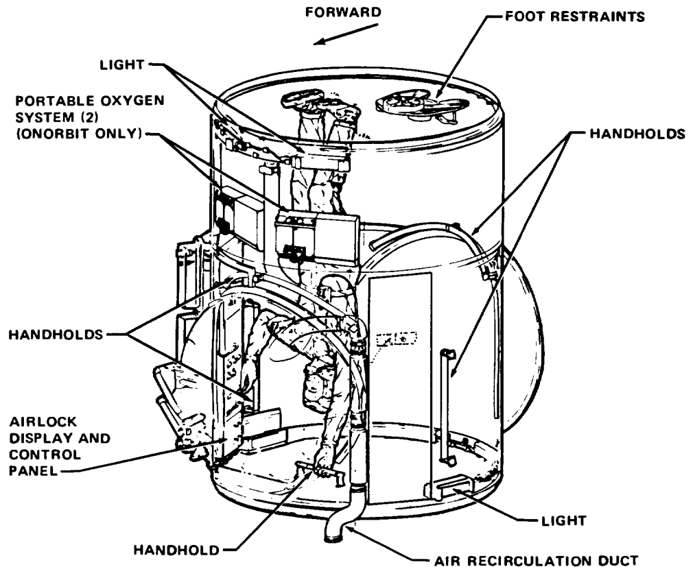
Figure 3-8.—Orbiter airlock.
