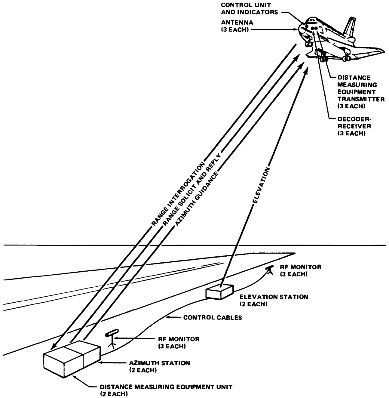
Figure 6-18.—Microwave scanning beam landing system.
