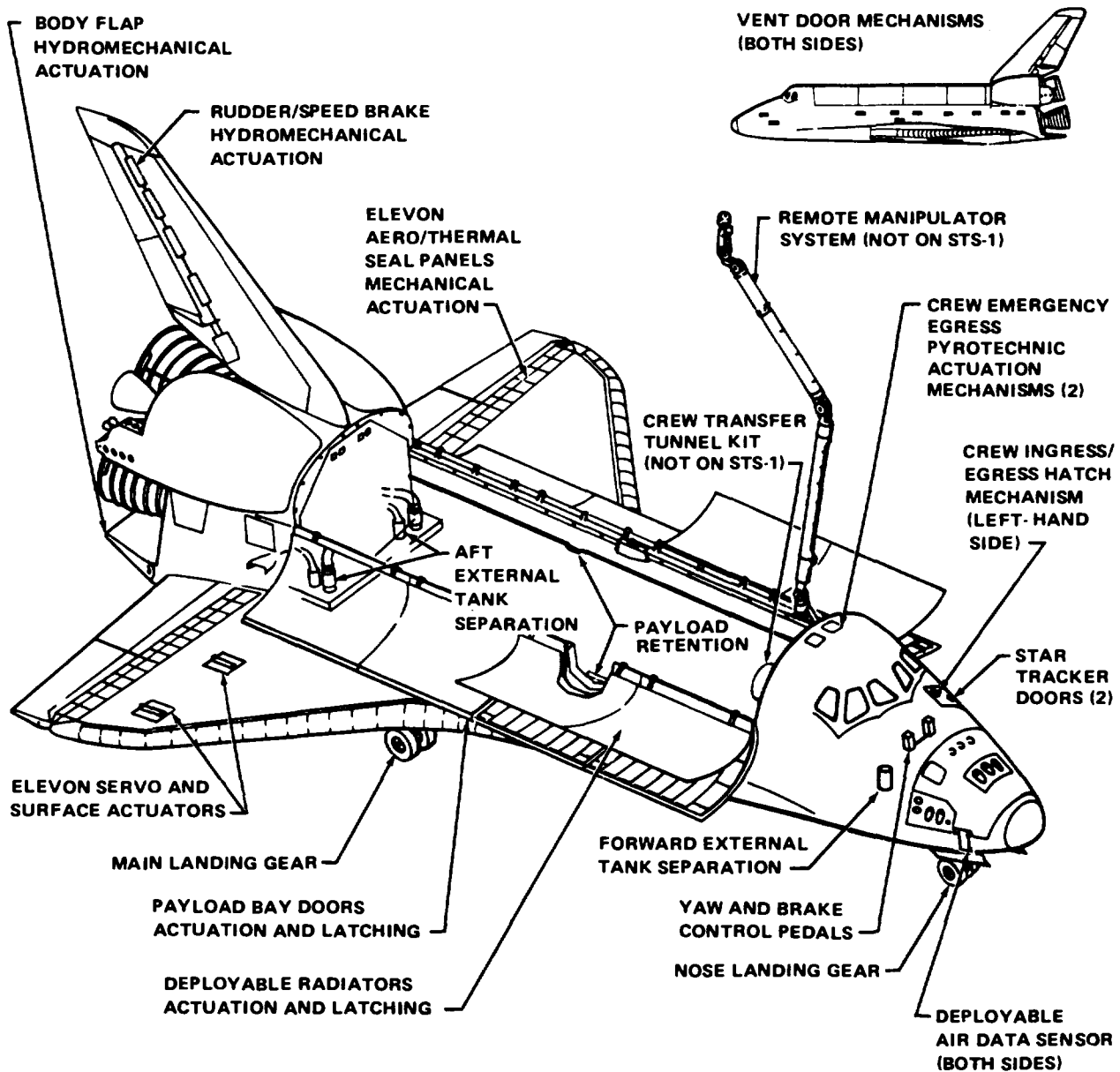
Figure 3-20.—Mechanical subsystems.
