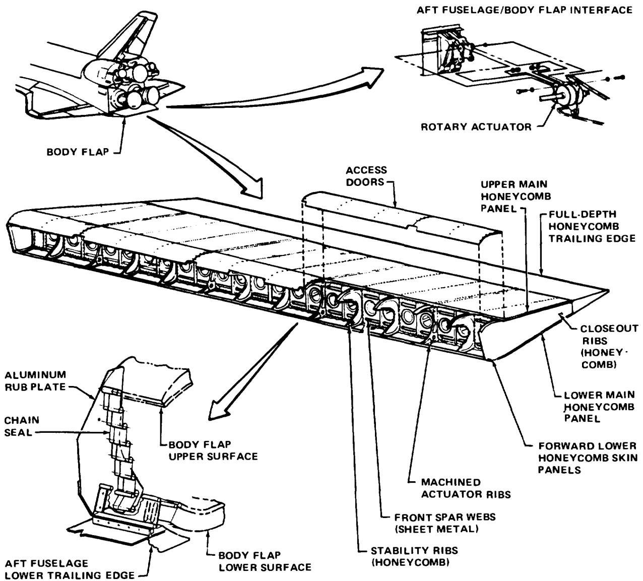
Figure 3-17.— Body flap.
