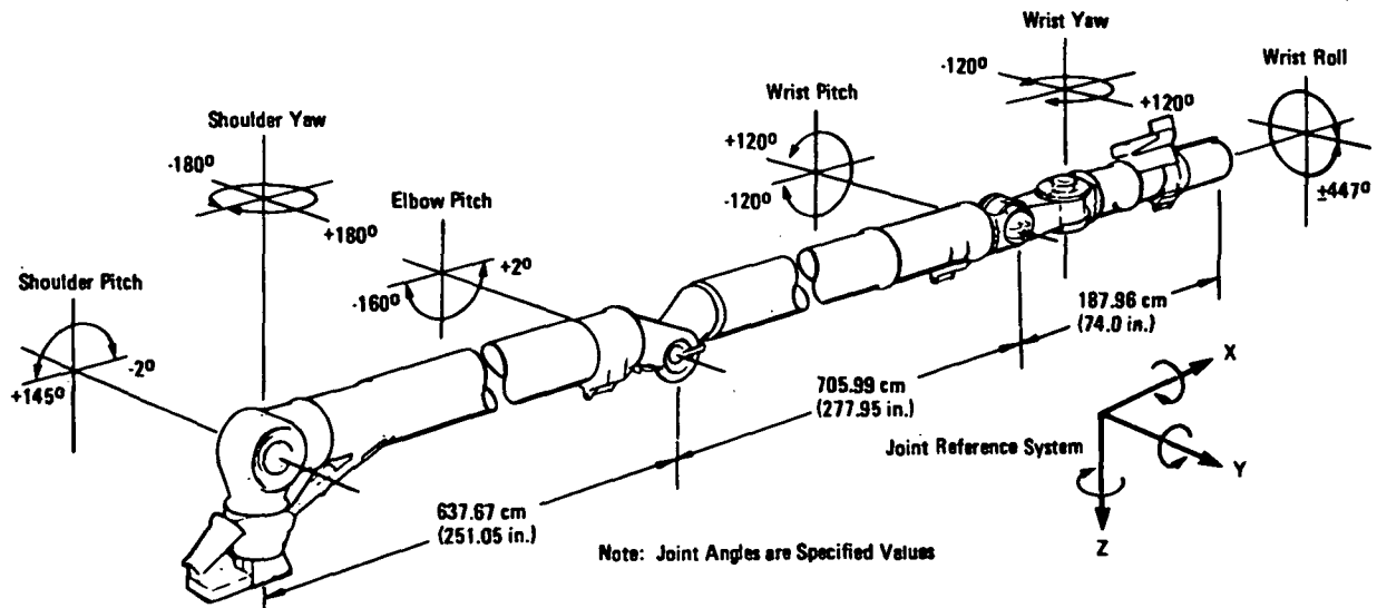
Mechanical Arm-Stowed Position and Movement Configuration
