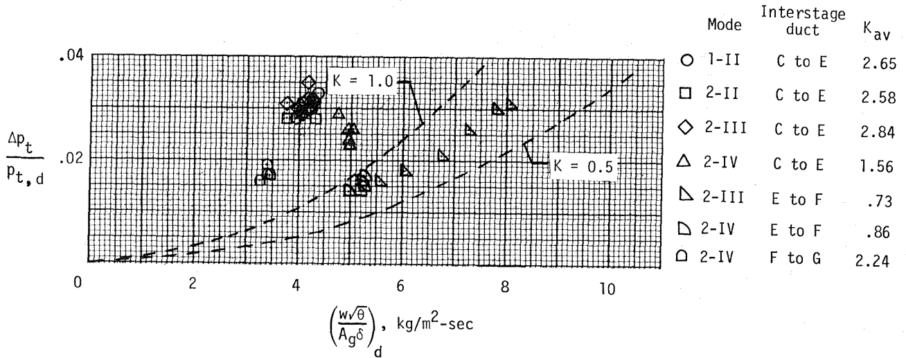
(c) Interstage pressure losses.
