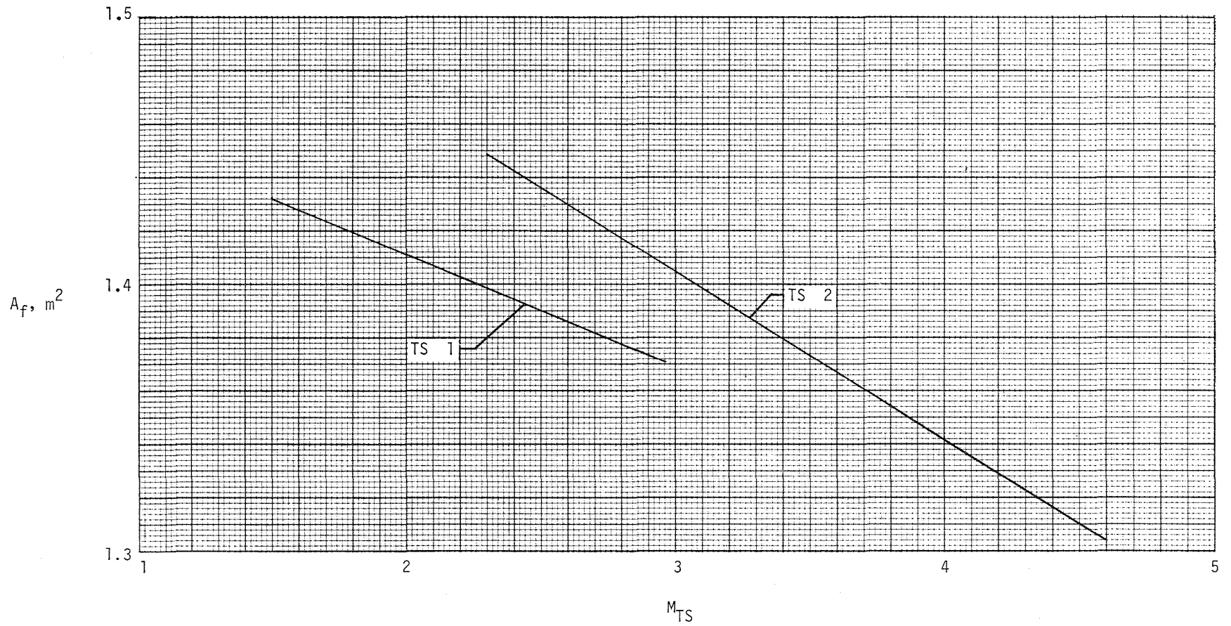
Figure 10.- Variation of test-section effective flow area with Mach number.
