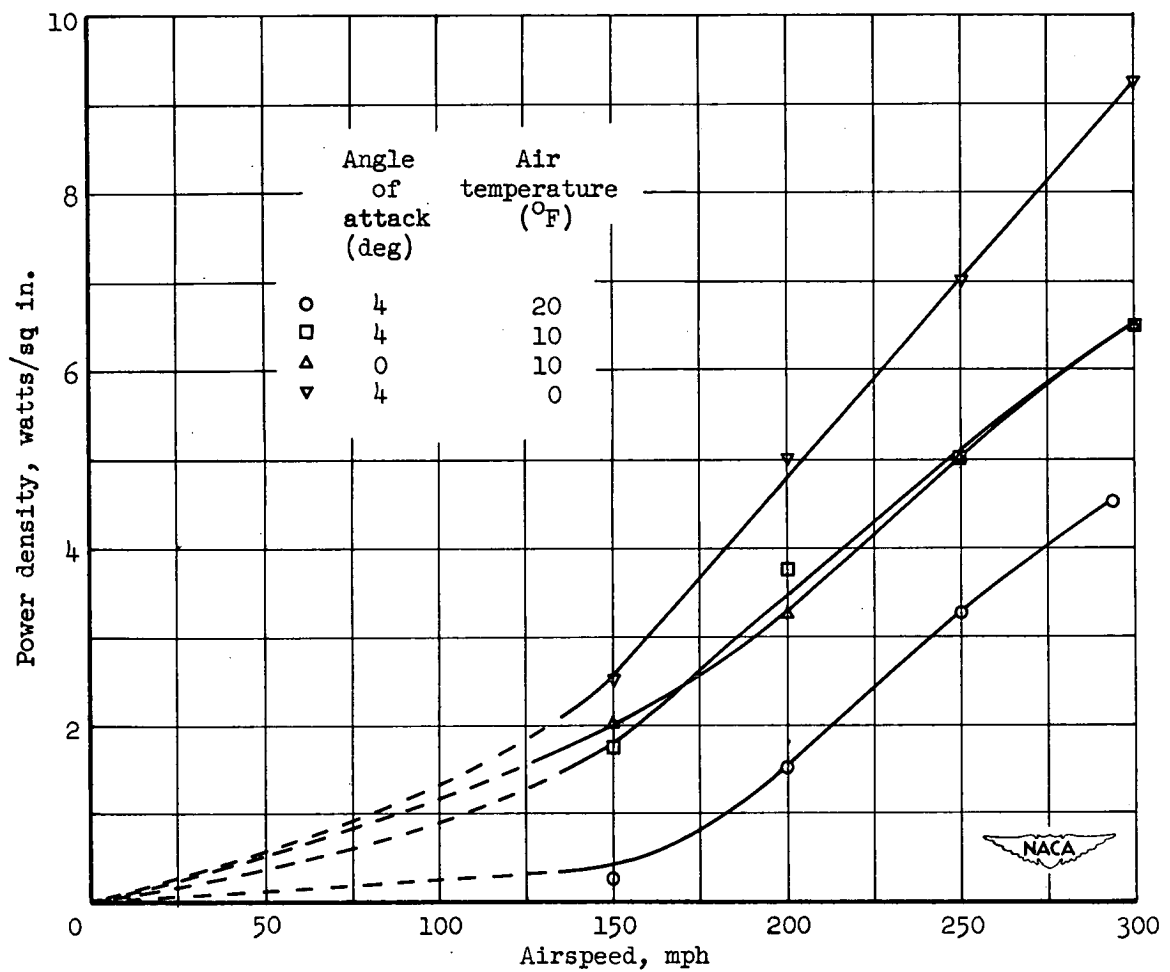
Figure 5. - Marginal power requirements for icing protection on leading edge of NACA 0018 airfoil section equipped with thermal-pneumatic de-icer.
