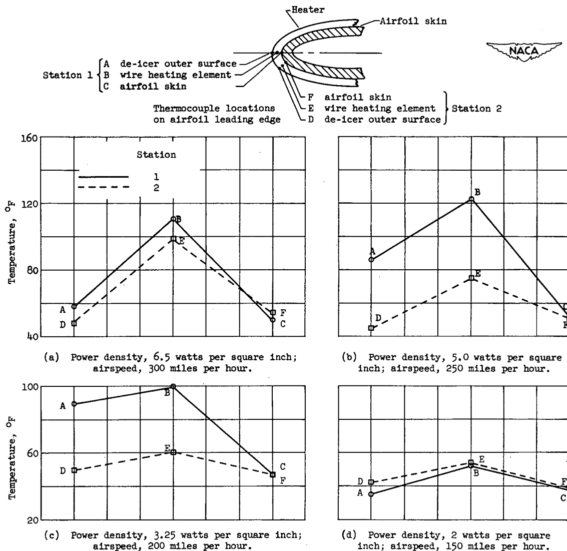
Figure 6. - Temperature pattern for thermal area of thermal-pneumatic de-icer at marginal power densities during icing. Air temperature, 10° F; angle of attack, 0°; liquid-water content, 2 grams per cubic meter; mean effective droplet size, 35 microns.
