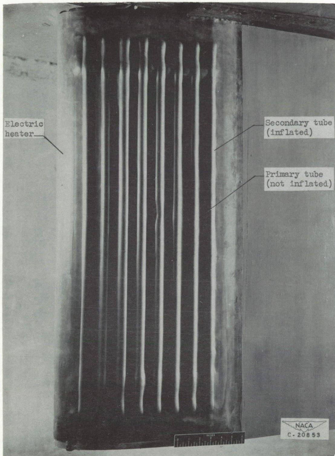
Figure 1. - Tunnel installation of thermal-pneumatic de-icer mounted on NACA 0018 airfoil showing secondary tubes inflated.
