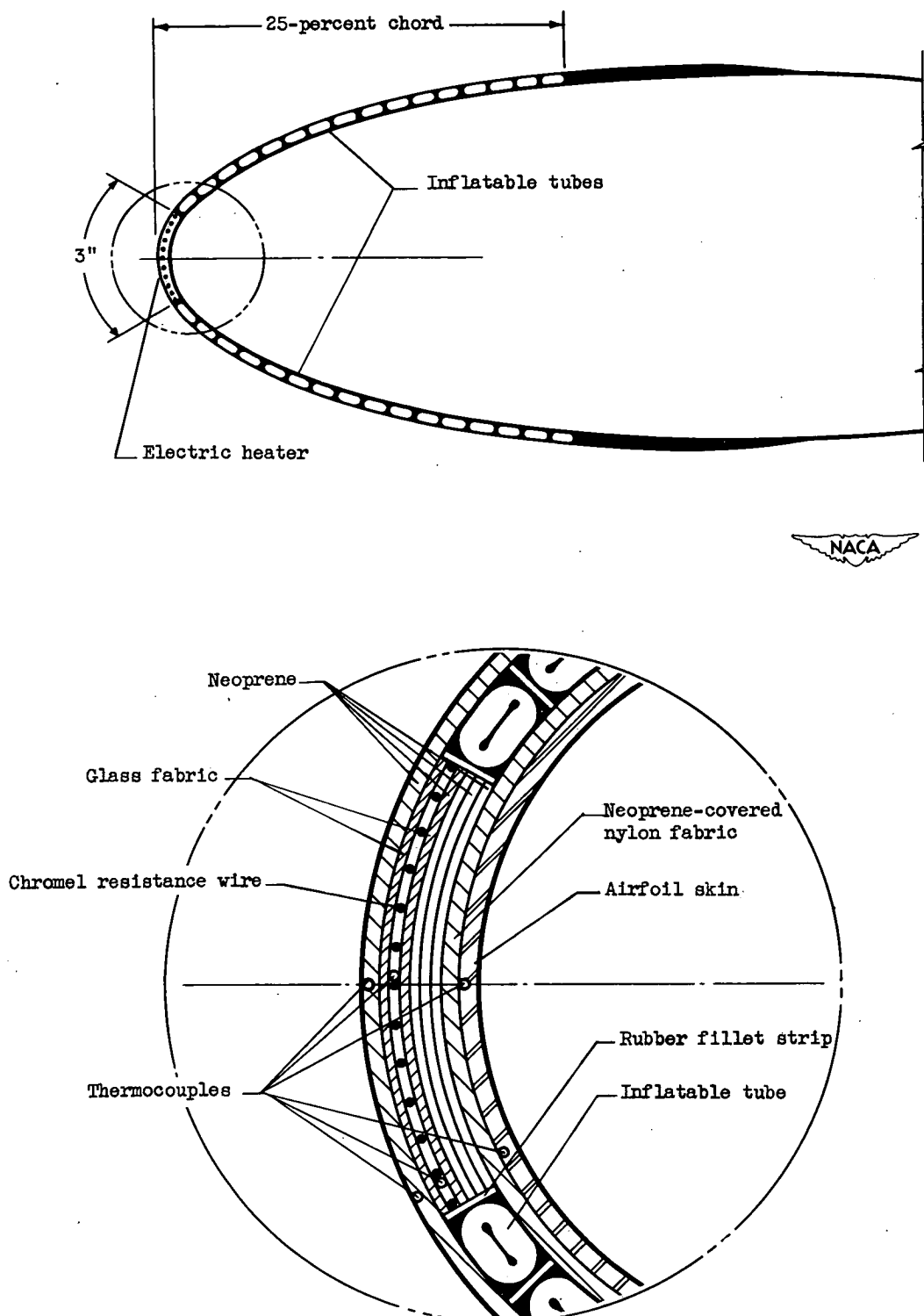
Figure 2. - Construction and installation details of thermal-pneumatic de-icer mounted on 42-inch-chord NACA 0018 airfoil.
