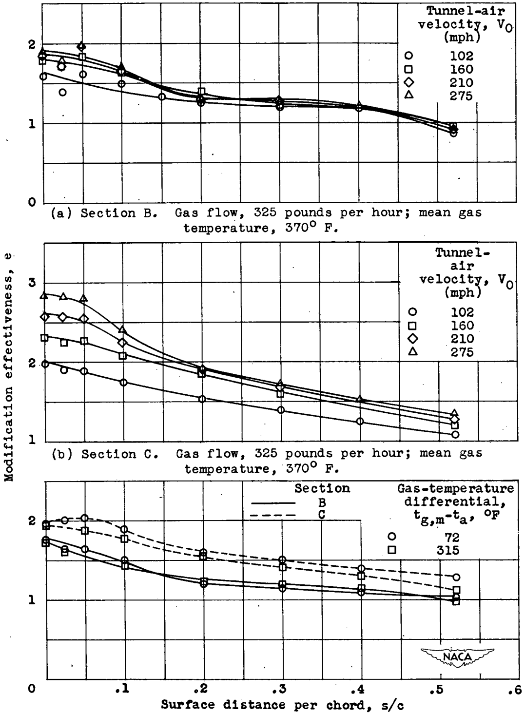
(c) Sections B and C. Gas flow, 325 pounds per hour; tunnel-air velocity, 102 miles per hour.
