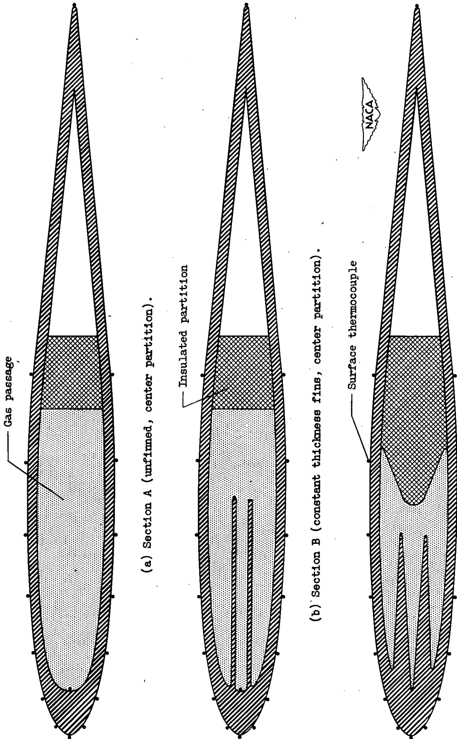
Figure 3. - Details of three gas-heated steel airfoil sections.
