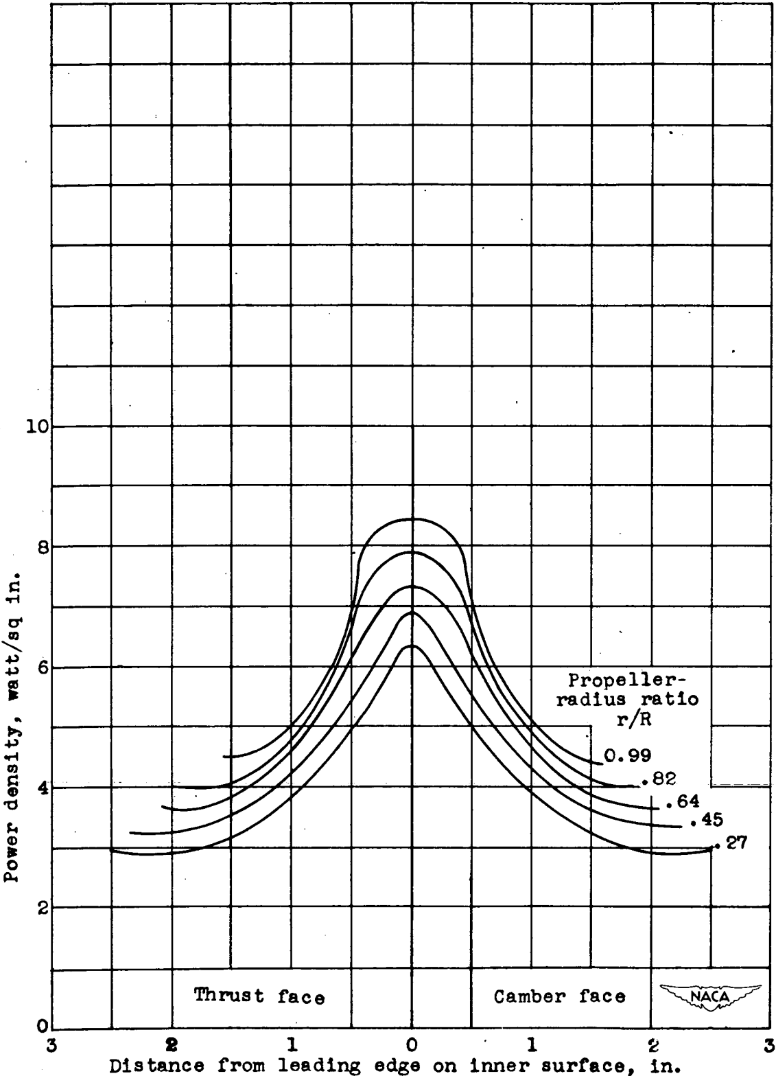
Figure 4.- Design power distribution at 1000 watts per blade (taken from data supplied by manufacturer).
